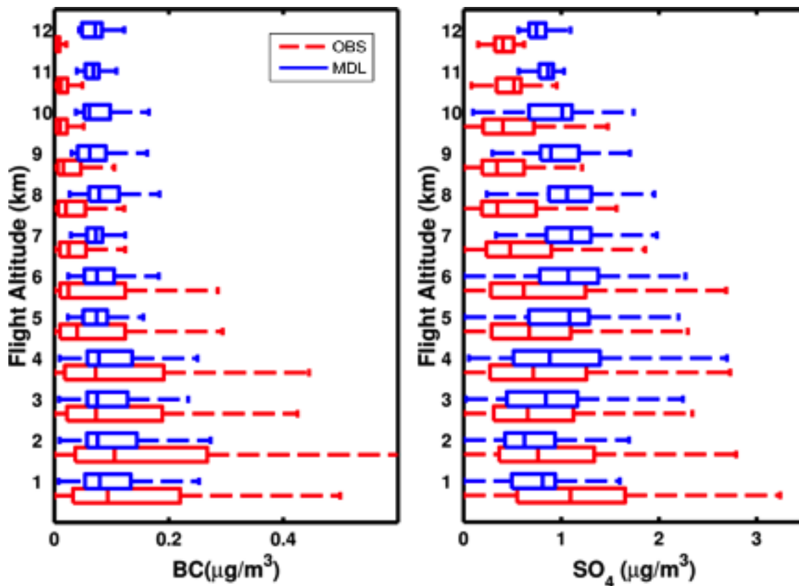
Figure 4: Comparison of model and observation BC and sulfate (SO 4 ) for all ARCTAS flights. In each box whisker panel, the middle line denotes the median value, while the edges of the box represent 25 th and 75 th percentile values respectively. The whiskers denote the maximum and minimum values.
