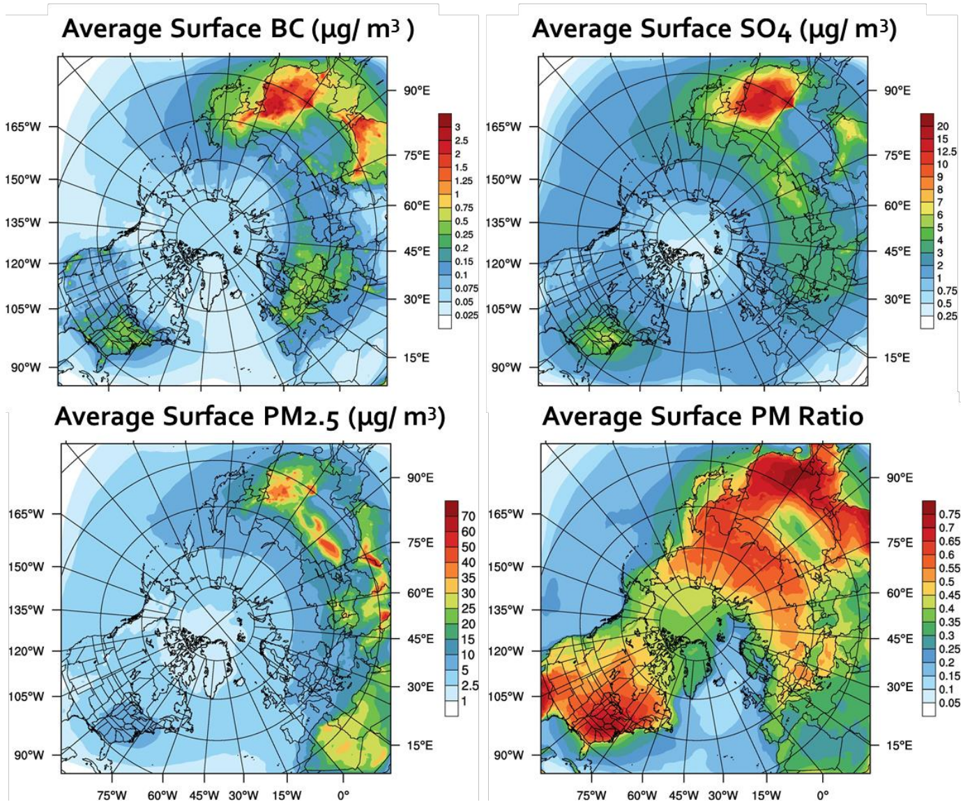
Figure 8: Spatial distributions of simulated BC ( \mu\text{g}/\text{m}^3 ), sulfate ( \text{SO}_4 ) ( \mu\text{g}/\text{m}^3 ), \text{PM}_{2.5} ( \mu\text{g}/\text{m}^3 ), and \text{PM}_{2.5}/\text{PM}_{10} ratio averaged over the simulation period. The annual averages are calculated by averaging model outputs from April, 01 2008 to March, 31, 2009. This figure is generated using NCAR Command Language (NCL) version 6.3.0, open source software free to public, by UCAR/NCAR/CISL/TDD, http://dx.doi.org/10.5065/D6WD3XH5 .
