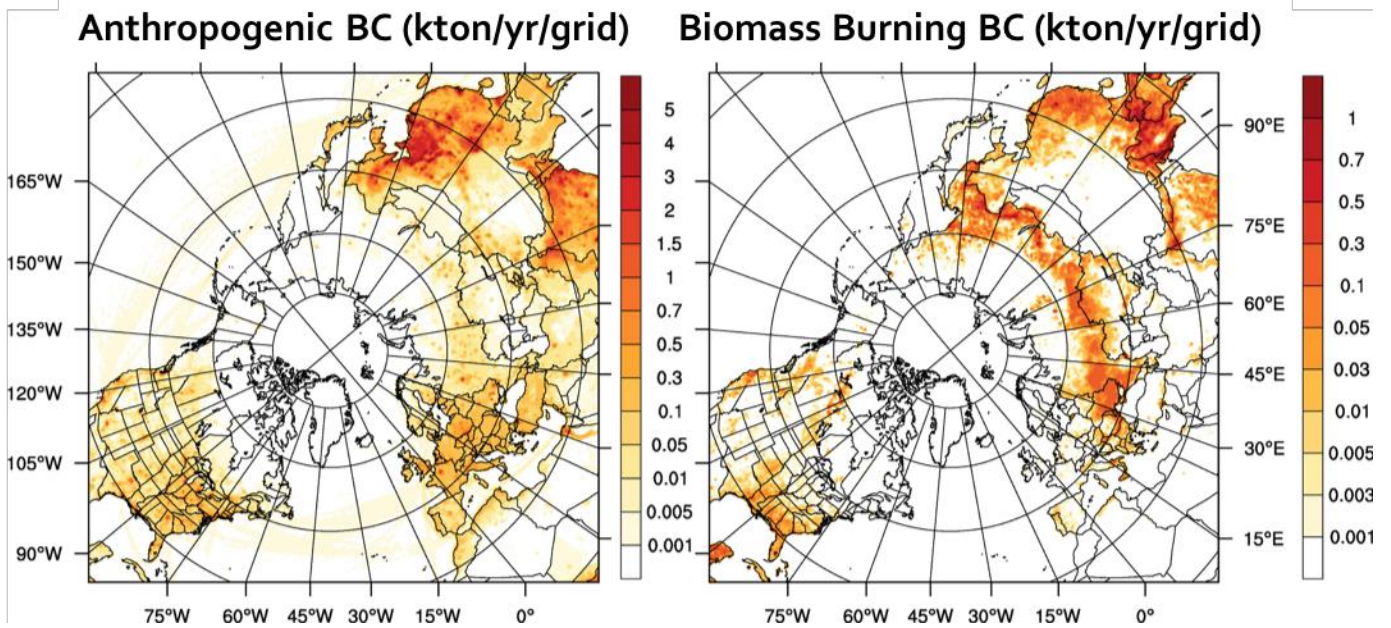
5 Figure 1: Spatial distribution of anthropogenic BC emissions (left) and wildfire BC emissions (right) in Gg/yr/grid. This figure is generated using NCAR Command Language (NCL) version 6.3.0, open source software free to public, by UCAR/NCAR/CISL/TDD, http://dx.doi.org/10.5065/D6WD3XH5 .
