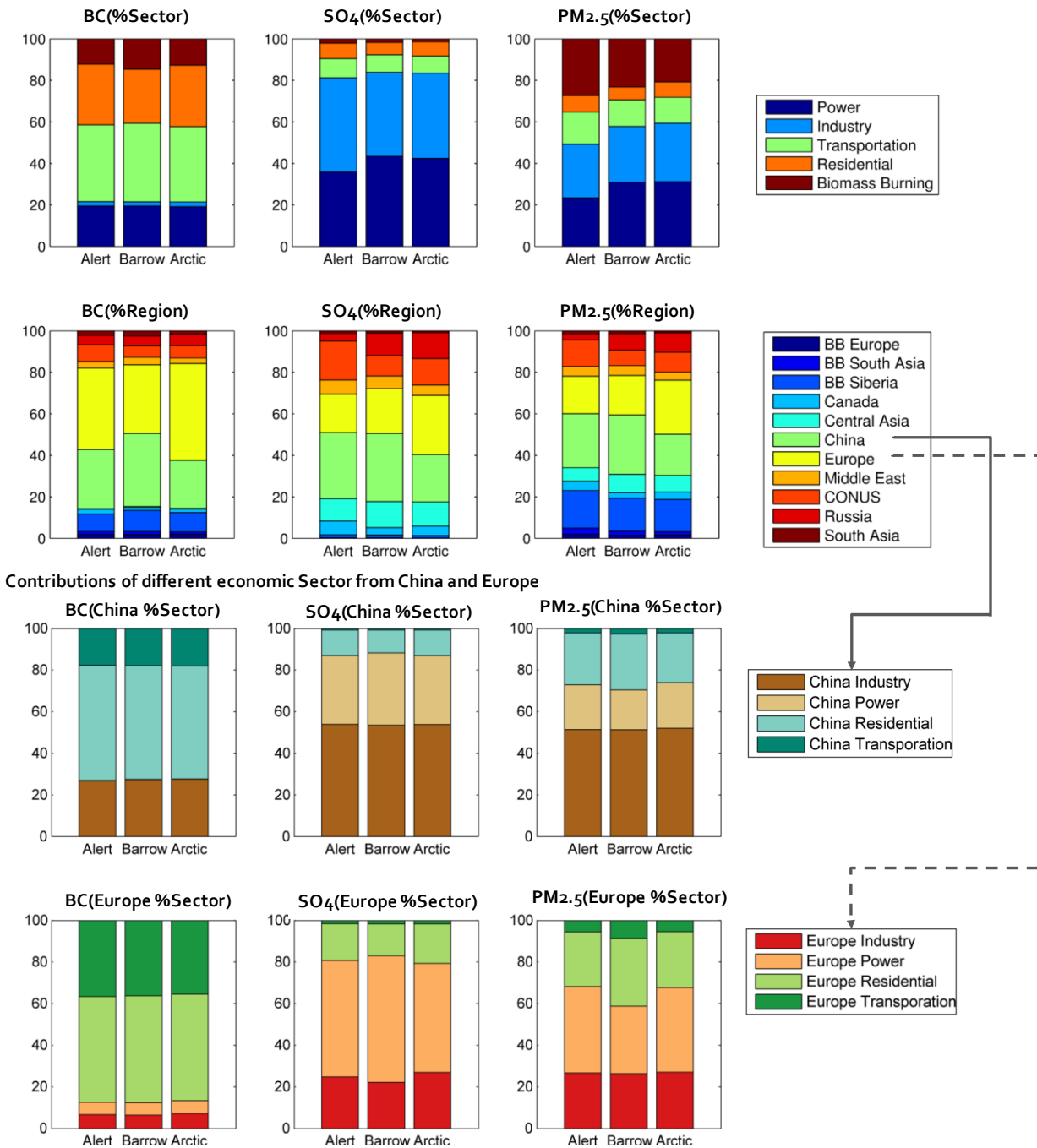
Figure 13: Summary of annual mean contributions to BC, sulfate (SO 4 ), and PM 2.5 by source sectors (top row) , and source regions (2nd row) at Alert, Barrow, and over the Arctic regions. The bottom two rows of bar plots show the relative contributions of various economic sectors from either China (3rd row) or Europe (bottom row) to total China or Europe contributions to Arctic BC, sulfate (SO 4 ) , and PM 2.5 concentration. BB denote biomass burning in this figure.
