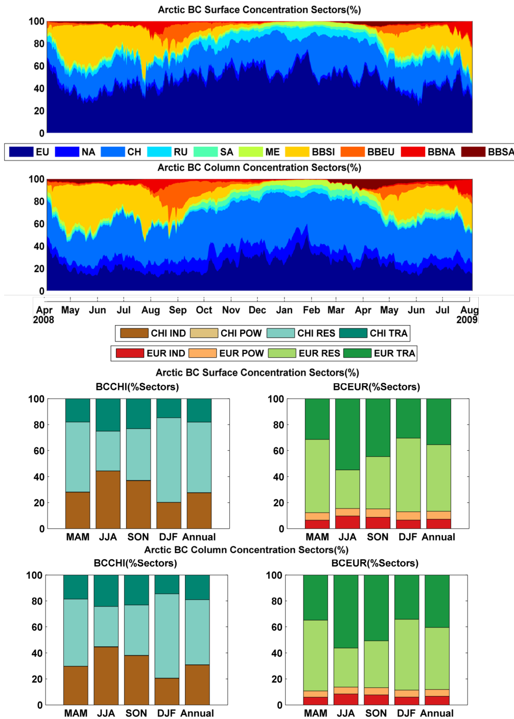
Figure 12: Top two subplots show the seasonality of BC major geographical contributors to the Arctic (latitudes > 60^{\circ}\text{N} ) surface (first row) and column (second row) concentrations. The bar plots (bottom 4 subplots) indicate the seasonality and annual average of contributions of various economic sectors from
