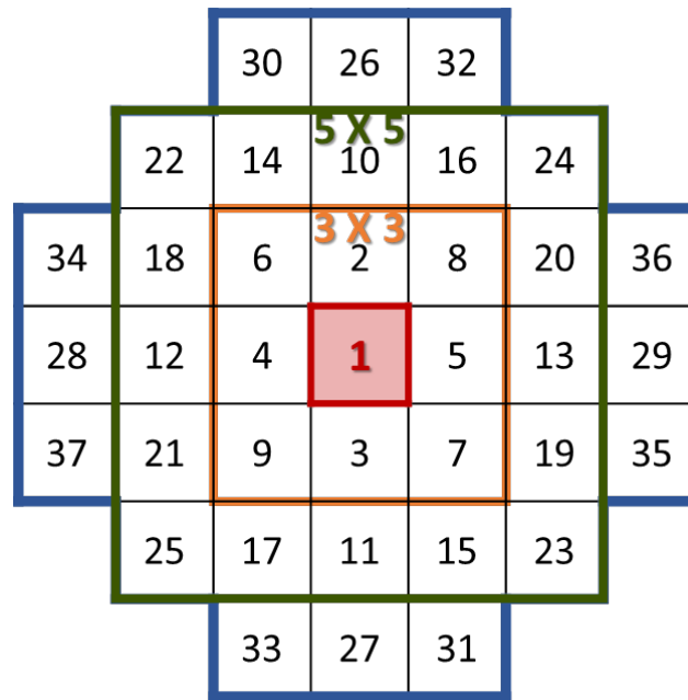
5 Supplementary Figure 1: The pixels within the circular neighbouring window with a radius of 3 pixels considered for oversampling. The number in each pixel indicates the order of inclusion of the pixel for oversampling. For example, oversampling for pixels of an interval might be conducted for first three pixels following the order, while oversampling for pixels of another interval might be conducted for up to the 13 th pixel within the window.
