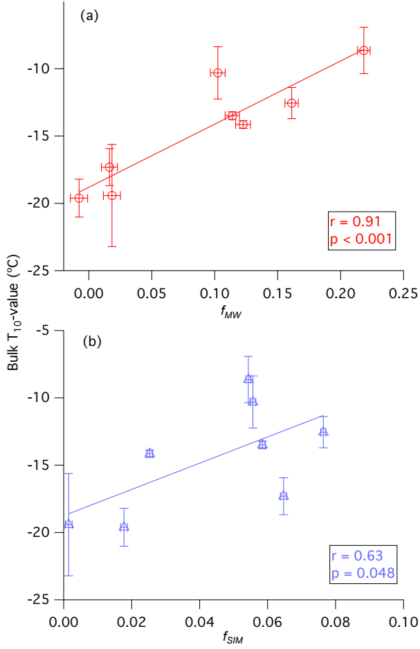
5 Figure 6. Relationships between T_{10} -values for bulk seawater and (a) the water volume fractions for meteoric water, f_{MW} , and (b) the water volume fractions for sea-ice melt, f_{SIM} . The x-error bars are due to the uncertainties in seawater salinities and seawater \delta^{18}O values used for calculating f_{MW} and f_{SIM} . For further details see Section 2.4. The y-error bars correspond to the 95% confidence interval for three repeat experiments.
