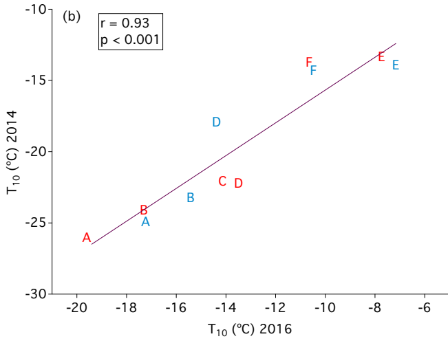
Figure 5. (a) Map showing regions of similar sampling locations in 2014 (pink) and in 2016 (blue). Sampling sites in 2014 that were near sampling sites in 2016 were paired together (indicated with boxes in the figure) and assigned letters A-F. Although there are two stations in box A for 2016, we only used data for the station that was closest to the one in 2014. (b) Relationships between T_{10} -values for microlayer and bulk seawater samples in 2014 and 2016 for similar sampling locations. The letters plotted in (b) indicate the locations in (a). Red letters represent bulk seawater data and blue letters represent microlayer data. Only freezing data that was at warmer temperatures than the field blanks are included.
