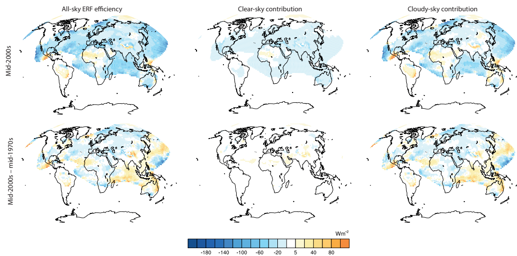
Figure 9. Anthropogenic aerosol effective radiative forcing efficiencies, in W m^{-2} per unit optical depth, for (left) all-sky, (middle) clear-sky, and (right) cloudy-sky. The top row shows efficiencies for mid-2000s anthropogenic aerosols. The bottom row shows differences made by using the pattern for the mid-1970s.
