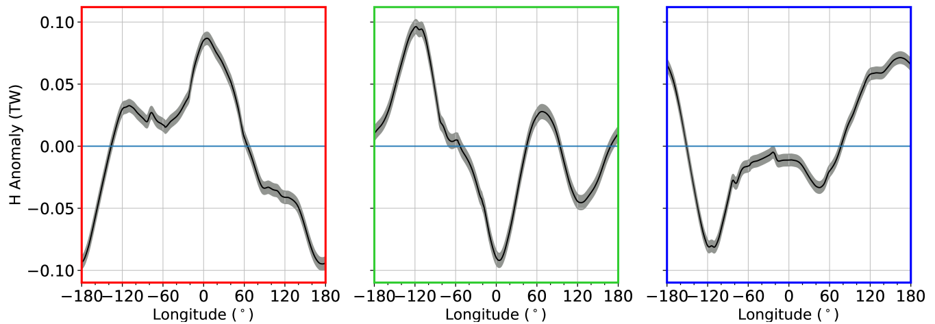
Figure 6. Composite of meridional heat transport anomalies at 75° N given in PW-TW for each of the three pathways. The mean values have been shown in Fig. 5. Red frame means transports through the North Atlantic, green frame through Siberia, and blue frame transports through the North Pacific. Grey shaded areas show the standard error. Positive sign denotes a transport anomaly to the north and negative sign denotes a transport anomaly to the south.
