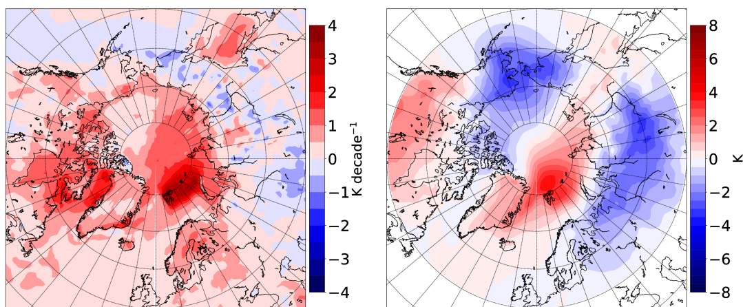
Figure 8. Left panel: temperature trend trends for the winter mean. Calculated, calculated for the winters from 1979/80 to 2015/16. Dotted regions indicate significance at the 95 % level. Trend is Trends are given in Kelvin per decade. Right panel: composite of temperature anomalies from the North Atlantic Pathway and the inverse of the North Pacific Pathway temperature anomalies as provided in Fig. 3, weighted by their relative frequency of occurrence (Fig. 2 top right number numbers ).
