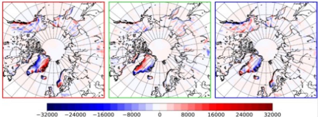
Figure A: Composite of mean of vertically integrated MSE transport divergence minus mean of the analyzed time frame.
