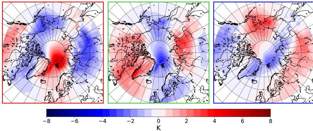
Figure 3. Composite of 2 meter temperature anomalies for each of three the pathways: the North Atlantic Pathway (left; red colored frame), the Siberian Pathway (middle; green colored frame), and the Northern Pacific Pathway (right; blue colored frame). Contour spacings show temperature anomalies in 0.5 K. Blue colors indicate a cold anomaly and red colors indicate a warm anomaly compared to the mean of the analyzed time frame.
