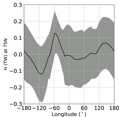
Figure 5. Mean vertically integrated (200 hPa-1000 hPa) meridional heat transport at 75° N given in Petawatts/Terawatts. Grey shaded areas show the standard deviation based on the daily data.
