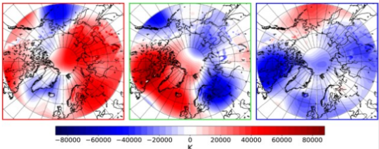
Figure 4: Composite of vertically integrated potential temperatures minus mean for the analyzed time frame.
