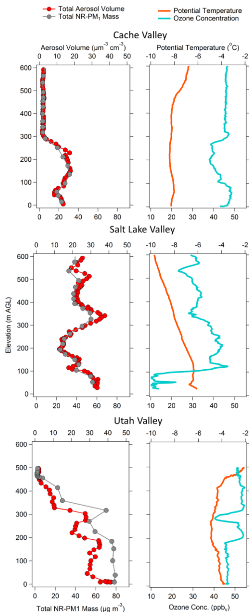
Figure 7: Comparison between selected vertical profiles. On the left is shown the aerosol volume, measured with the UHSAS (in red) and NR-PM 1 mass measured with the AMS (in grey) as function of elevation in m AGL. On the right: are shown vertical profiles of ozone concentration (light blue) and potential temperature (orange) for the same three missed approaches. The missed approach in Cache Valley took place on Jan 28 at 18:38 MST at the Logan-Cache Airport (LGU); the one in Salt Lake Valley on Jan 28 at 20:22 MST at Salt Lake City International (SLC), and the one in Utah Valley on Jan 30 at 13:24 MST at the Provo Municipal Airport (PVU).
