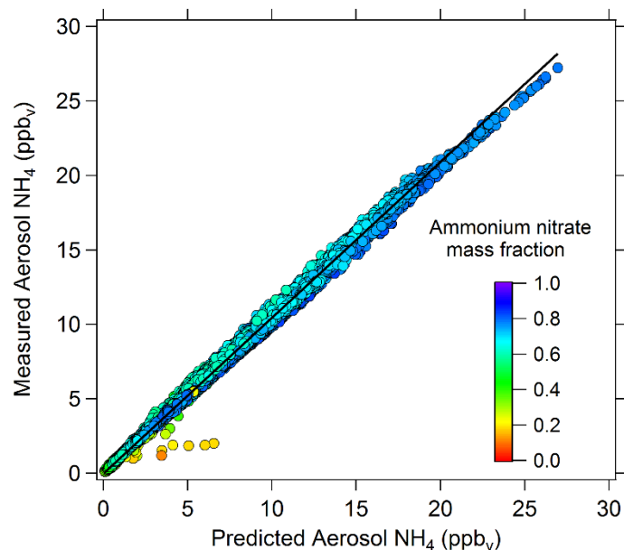
Figure 5: Aerosol ion balance from the AMS measurements. On the x-axis is the calculated mass of ammonium for fully neutralized aerosols ( \text{NH}_4^+ = 18 * (\text{NO}_3^- / 62 + \text{SO}_4^{2-} / 96 * 2 + \text{Cl}^- / 35.45) ). On the y-axis is the measured ammonium ( \text{NH}_4^+ ) in the aerosol particles. The black line is the 1:1 line, where points on the line correspond to neutralized aerosols and below the line are acidic aerosols. Data are color-coded by the ammonium nitrate mass fraction.
