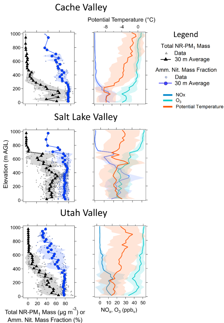
Figure 8: Left: average vertical profiles of NR-PM 1 mass (black triangles) and ammonium nitrate mass fraction (blue circles) measured during Episode#2. The triangular small grey markers and the small light blue circles are data used in the averages for all the missed approaches at the same airports as in Figure 7. The black triangles and dark blue circles are averages over 30 meters with their associated standard deviations. Right: corresponding vertical profiles of NO x (blue lines), O 3 (aqua lines) and potential temperature (orange lines).
