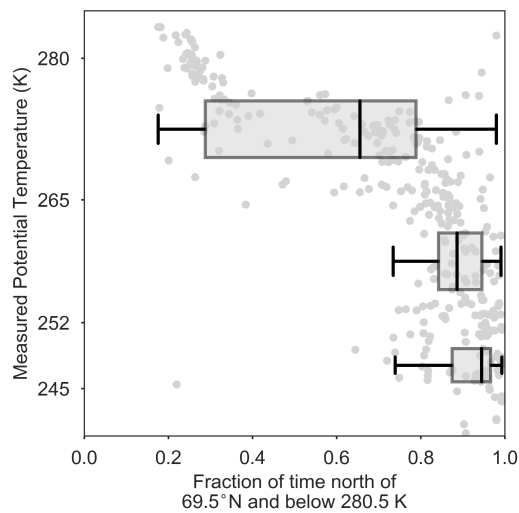
Figure 4. Observed potential temperature (K) as a function of versus FLEXPART-ECMWF predicted fraction of the past 10 days in the polar dome (i.e., below 280.5 K and north of 69.5°N). The FLEXPART-ECMWF relative residence time is binned in the lower (245 – 252 K), middle (252 – 265 K) and upper (265 – 280 K) polar dome.
