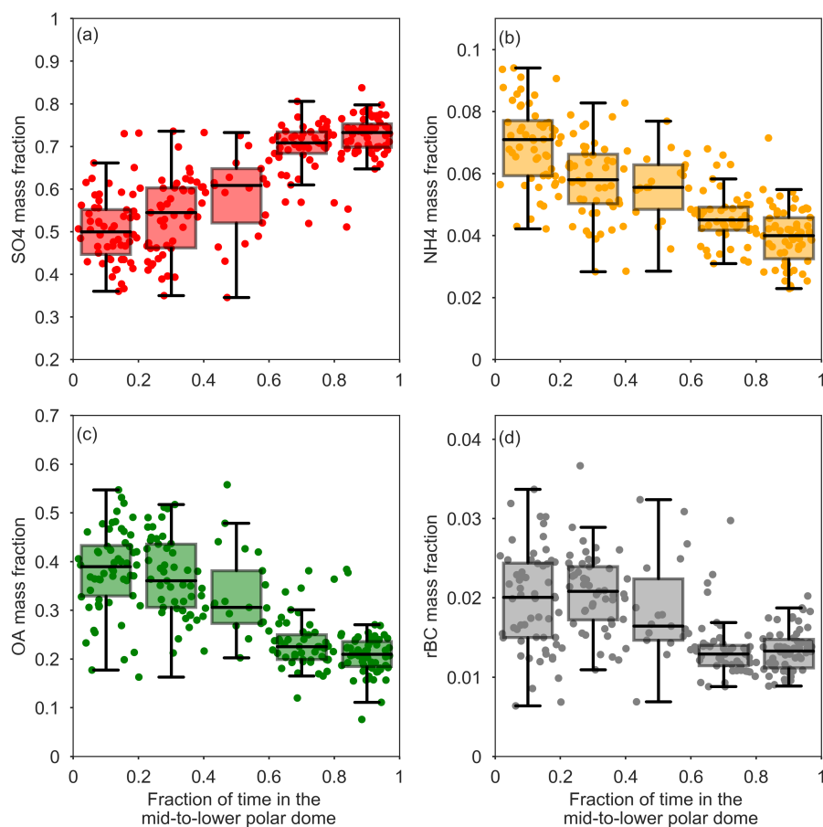
Figure 7. Submicron aerosol mass fractions as a function of versus FLEXPART-ECMWF-predicted fraction of the previous 10 days prior to measurement spent in the middle to lower polar dome (north of 69.5°N (Bozem et al., 2018) and, based on trace gas profiles, below 265 K (~1600 m)). Data points corresponding to individual FLEXPART-ECMWF releases are shown as circles, and summary statistics are shown as boxes (25 th , 50 th , 75 th percentiles) and whiskers (5 th , 95 th percentiles) for data binned by time spent in the middle and lower polar dome.
