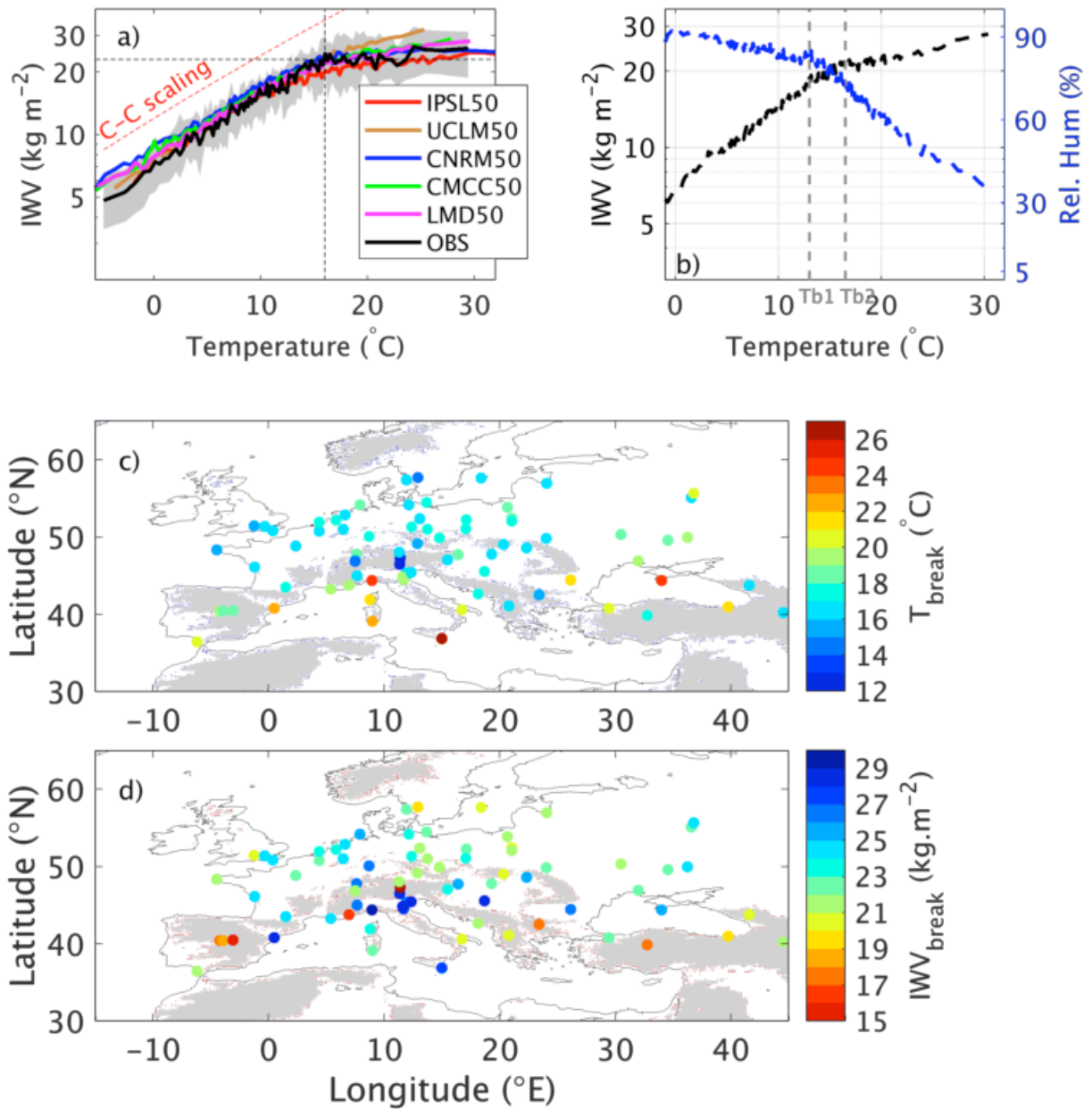
Figure 5: (a) I WV – T(2m) relationship at SIRT A station from observations and models. Median values are plotted for observations and models. The grey band represents the interval between the 20th and 80th quantiles for observations. The black vertical dashed line shows T_{\text{break}} , the black horizontal dashed line shows I WV_{\text{break}} , and the red slant dashed line shows C-C scaling (b) Median values of I WV and RH(2m) as a function of T(2m) at SIRT A from observations only. The vertical grey dashed lines indicate the values of T_{b1} and T_{b2} (see text section 4). (c) Map of T_{\text{break}} at all the GPS stations. (d) Map of I WV_{\text{break}} at all the GPS stations.
