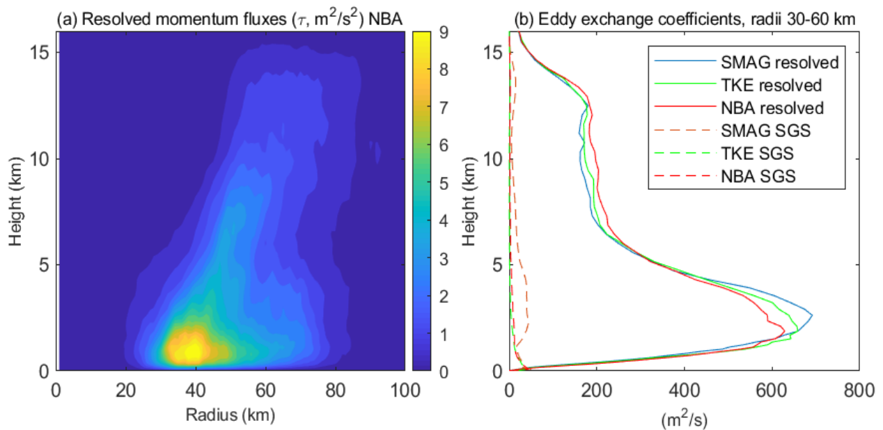
Figure 2: (a): Azimuthal-mean radius-height distribution of the vertical momentum fluxes, \tau = (\overline{w'u'^2} + \overline{w'v'^2})^{\frac{1}{2}} , induced by the resolved eddies with scales smaller than 2 km from the WRF-LES that uses the 3D NBA SGS model. (b): Vertical profiles of the parameterized (dashed) and resolved (solid) vertical eddy exchange coefficients of momentum averaged over 30 – 60 km radii (where the eyewall is located) from the three LESs that use different 3D SGS models. Note that the results are averaged over 3 – 8 simulation hours and the SGS eddy exchange coefficients are the direct output from the 3D SGS models used in the simulations.
