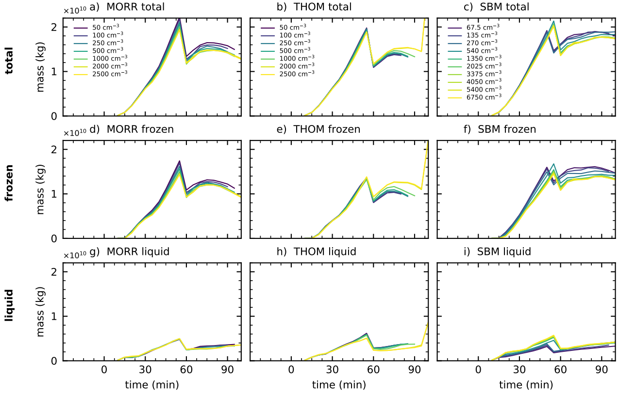
Figure 12. Total water mass, liquid water mass and frozen water mass in the analysed right-moving cell for the three different microphysics schemes (Morrison: left, Thompson: middle, SBM: right) in CASE1. The jump in the curves occurs at the point where the cell splits into two individual cells.
