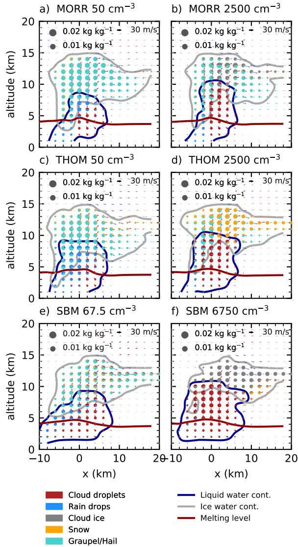
Figure 5. Hydrometeor mass mixing ratios in a slice along the line of travel of the cell for the cleanest (left) and most polluted (right) simulations after 60 minutes of simulation for the three microphysics schemes in CASE1.
