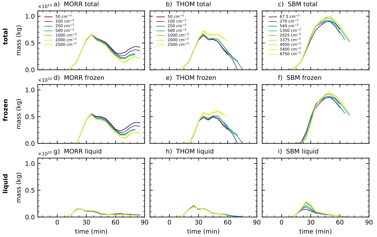
Figure 15. Total water mass, liquid water mass and frozen water mass in the analysed left-moving cell for the three different microphysics schemes (Morrison: left, Thompson: middle, SBM: right) in CASE2.
