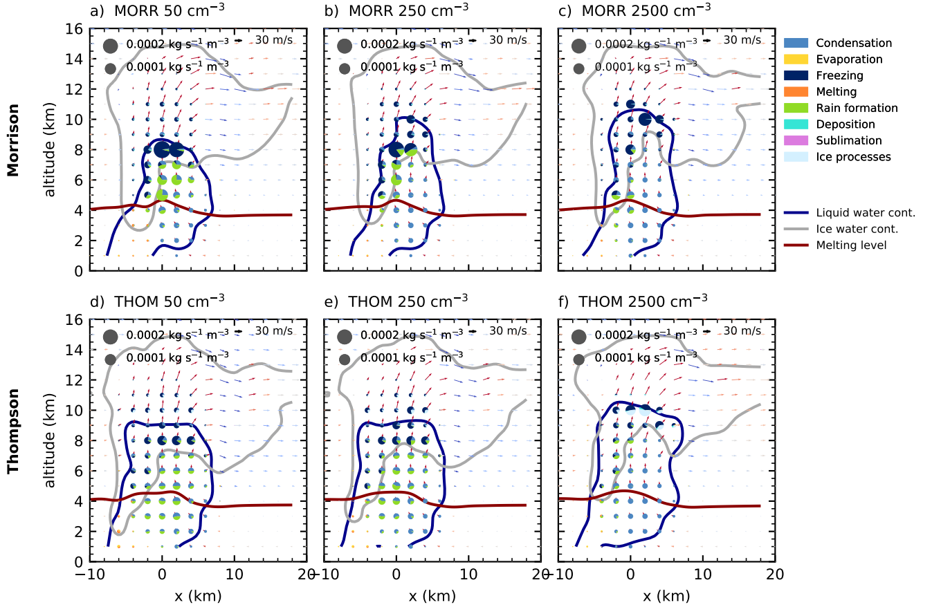
Figure 4. Cloud microphysical morphology along a slice through the cloud parallel to the track of the cell for simulations with three different CDNC values (left: 50 cm -3 , middle: 2500 cm -3 , right: 2500 cm -3 ) after 60 minutes of simulation using the two bulk microphysics schemes (top: Morrison, bottom: Thompson).
