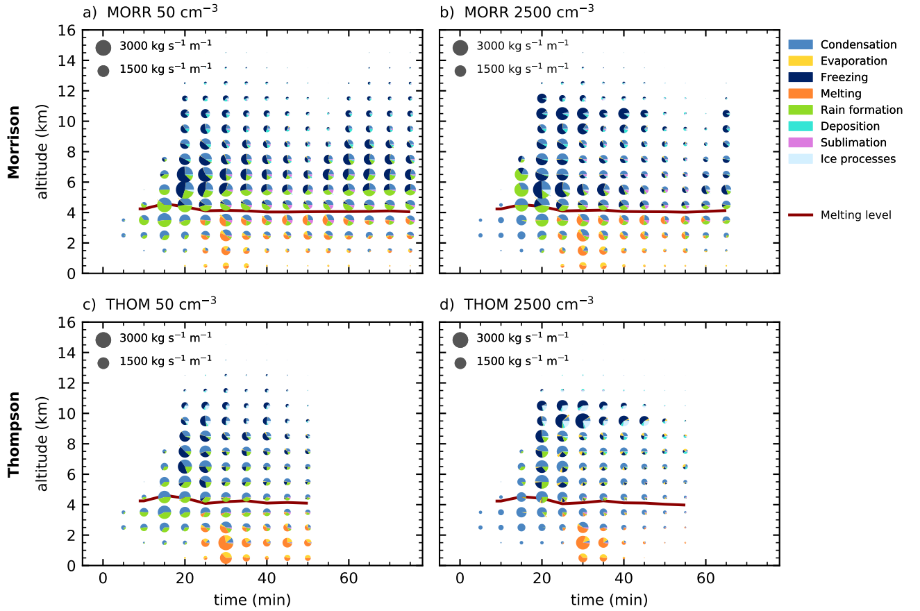
Figure 14. Temporal evolution of the microphysical process rates in CASE2 for the cleanest (left) and most polluted (right) simulations and the two bulk microphysics schemes (Morrison: top, Thompson: bottom). The pie charts denote the different groups of microphysical process rates with the area proportional to the sum of the microphysical process rates in the specific altitude interval inside the cloud volume.
