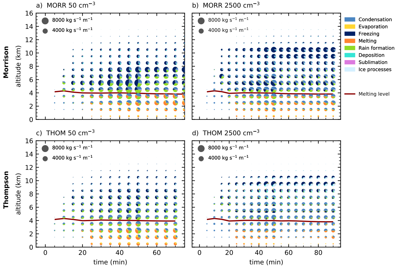
Figure 6. Time evolution of the microphysical process rates for the cleanest (left) and most polluted (right) simulations and the two bulk microphysics schemes (Morrison: top, Thompson: bottom) in CASE1. The pie charts denote mass transfer summed up over the volume of the cloud in each altitude interval for the different groups of microphysical process rates with the area of each colour proportional to the mass transfer. The red line shows the height of the 0°C isotherm.
