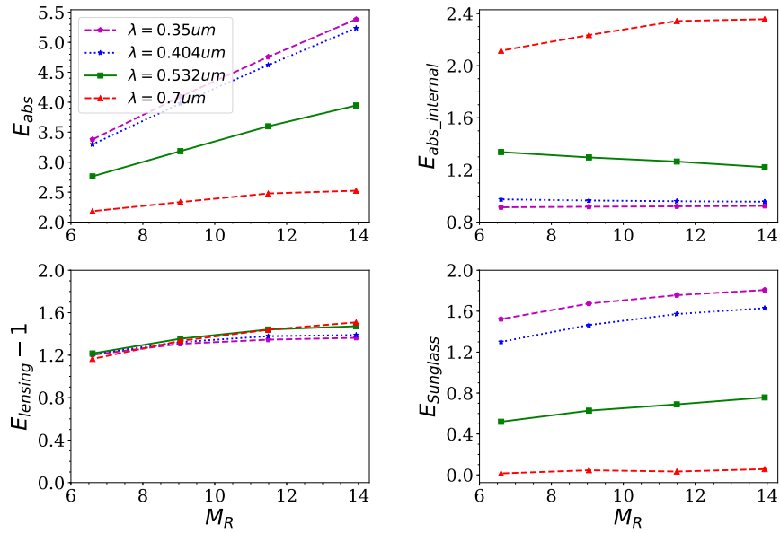
Figure 11. E_{abs} and E_{abs\_lensing} of thickly-coated BC with BrC coatings varying with M_R ( r_g = 0.06 \mu\text{m} , \sigma_g = 1.5 ).
