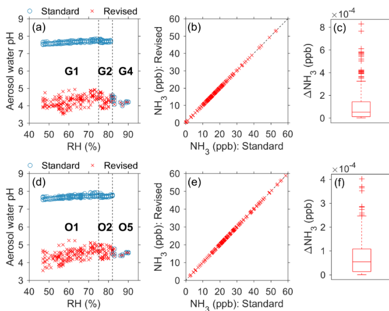
Figure S3. Comparisons of the predicted pH and gas phase \text{NH}_3 concentrations between the standard and revised ISORROPIA-II models with the stable state assumptions. (a–c) show the results using the AMS \text{PM}_{10} measurements (an \text{NH}_3\text{--H}_2\text{SO}_4\text{--HNO}_3\text{--HCl--H}_2\text{O} aerosol), and (d–f) show the results using the GAC-IC \text{PM}_{2.5} measurements (a \text{K--NH}_3\text{--Na--H}_2\text{SO}_4\text{--HNO}_3\text{--HCl--H}_2\text{O} aerosol).
