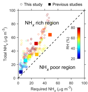
Figure 2. Relationship between required NH x and total NH x concentrations under Beijing winter haze conditions. The circles indicate hourly measurements in this study and the filled squares indicate measurement results from previous studies (Wang et al., 2016; Liu et al., 2017a) in winter Beijing. The dash line indicates a 1:1 relationship and defines the NH x -rich region (above) and NH x -poor region (below).
