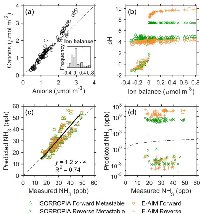
Figure 31. Relationship between ion balance and predicted particle pH in forward mode and reverse mode calculations, and a comparison of measured and predicted gas phase \text{NH}_3 mixing ratios. (a) Cation-to-anion equivalent ratios in \text{PM}_{2.5} during the field measurements. The inserted figure displays the frequency distribution of ion balance values. The dash line indicates a 1:1 relationship. (b) Predicted pH vs. ion balance. The dash line indicates ion balance equal to zero. (c-d) Comparisons of predicted and measured gas phase \text{NH}_3 mixing ratios. The dash lines indicate a 1:1 relationship. The solid line in (c) represents the linear correlation between predicted and measured \text{NH}_3 levels (the ISORROPIA forward metastable and E-AIM forward calculations have essentially the same results). The eligible number of samples ( n = 106 ) is limited by the requirement in E-AIM that \text{RH} > 60\% .
