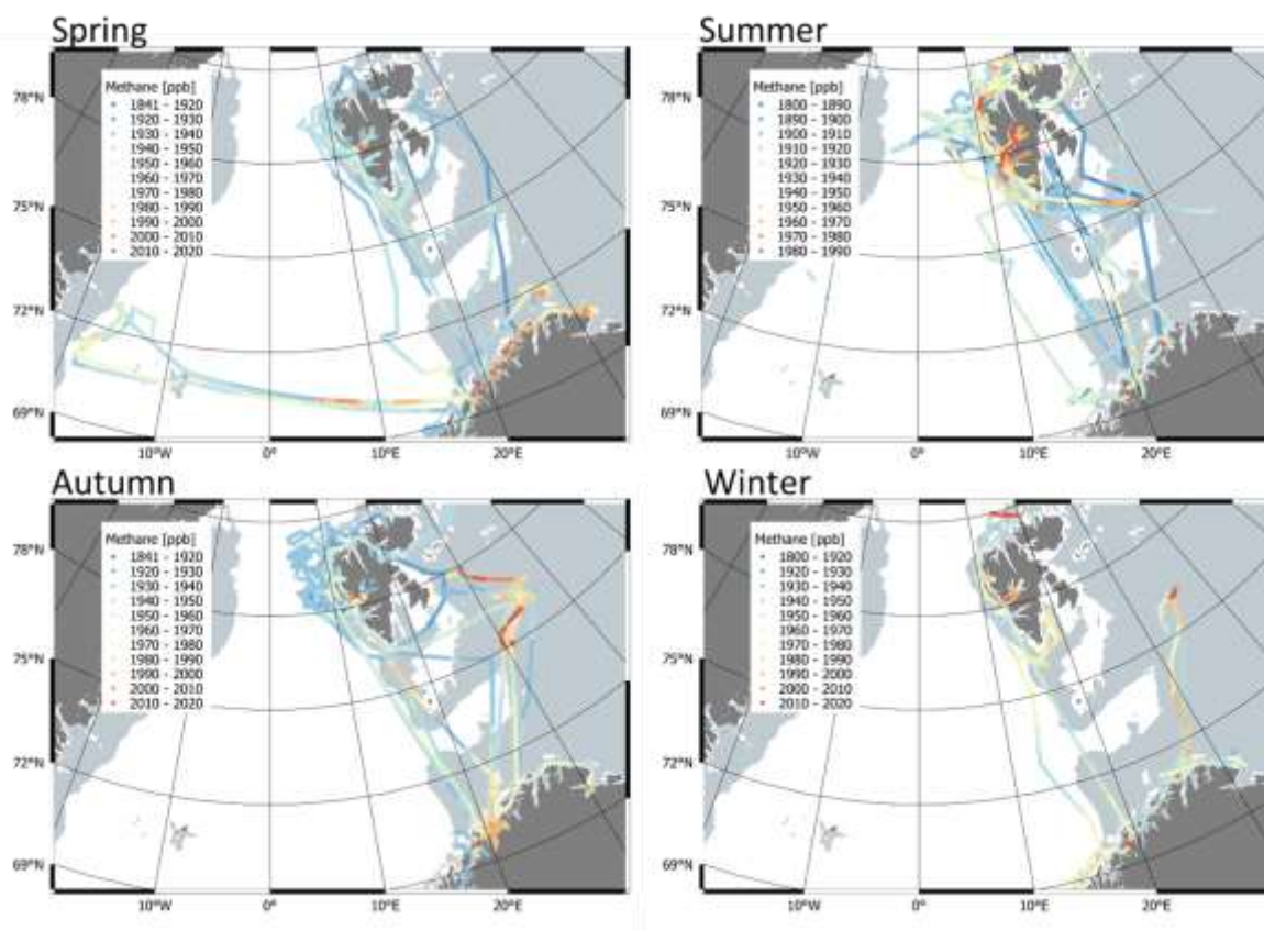
Figure 5: Methane mixing ratios observed at the RV Helmer Hanssen (colour scale), by location and plotted by calendar season (i.e. winter is December/ January/ February). Please note the change in colour scale between panels.
