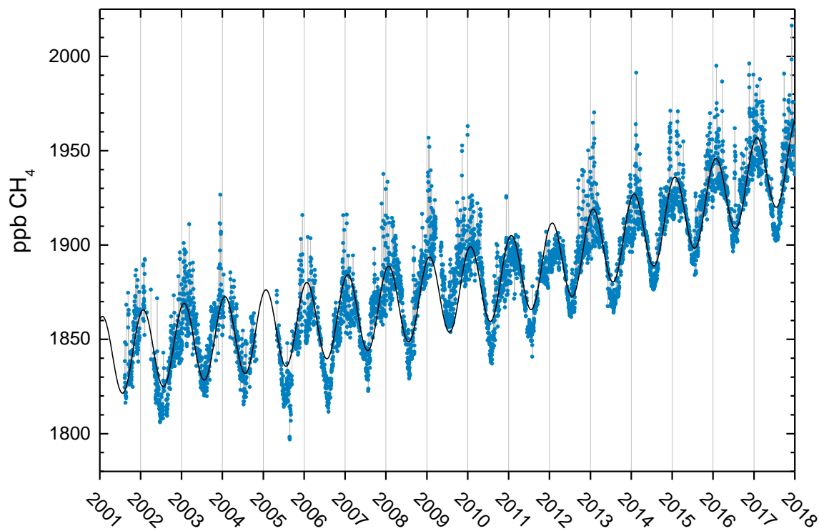
Figure 3: Observations of daily averaged CH 4 mixing ratio for the period 2001-2017 at the Zeppelin Observatory. The blue dots are daily mean mixing ratios in ppb, and the black solid line is the empirically fitted CH 4 mixing ratio (Eq. 1).
