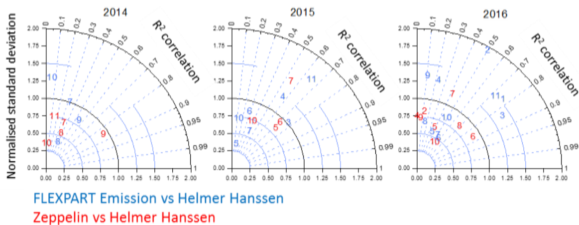
5 Figure 7: Taylor diagrams showing the monthly R 2 correlation (angle) and normalised standard deviation (radial axis) of modelled CH 4 emissions (blue) and CH 4 observed at Zeppelin Observatory (red, only for ship positions within 75-82° N, 5-35° ) compared to the RV Helmer Hanssen CH 4 time series. Numbers refer to month of the year. Ideal agreement would be found at 1 on the radial axis (black line) and 1 on the angular axis.
