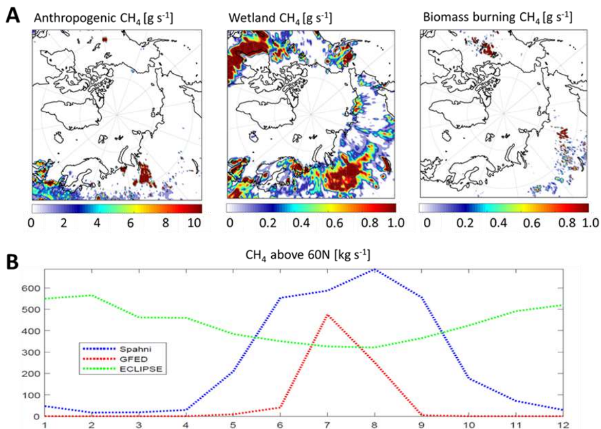
Figure 4: A) Annual average high latitude CH 4 emissions from anthropogenic sources, wetlands and biomass burning according to GAINS ECLIPSE (Stohl et al., 2015; http://www.iiasa.ac.at/web/home/research/researchPrograms/air/ECLIPSEv5a.html ), LPX-Bern (Spahni et al., 2011;Stocker et al., 2014; www.climate.unibe.ch ) and the Global Fire Emissions Database, GFED, (Randerson et al., 2017), respectively. B) Monthly variation in anthropogenic, wetland, and biomass burning emissions above 60°N
