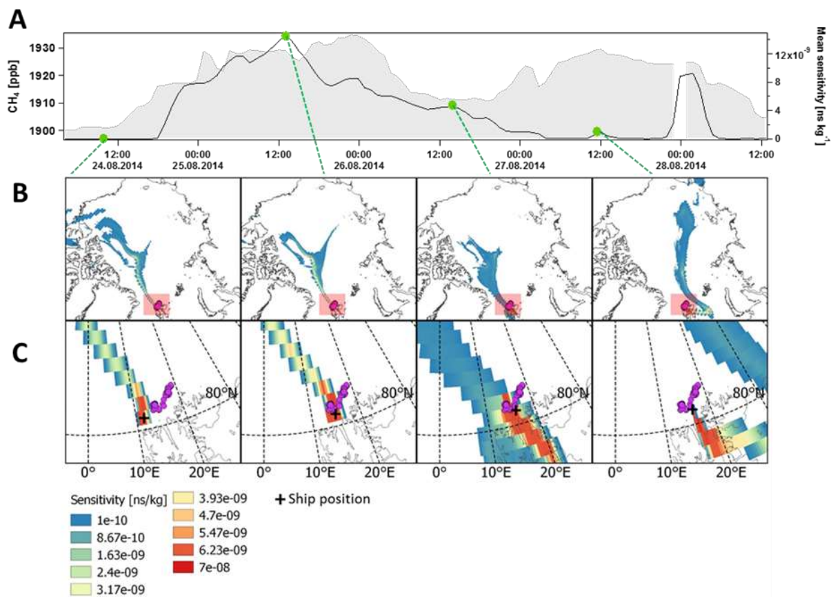
5 Figure 8: A) Methane (CH 4 ) measured North of Svalbard at the RV Helmer Hanssen shortly before, during, and after an episode of increased mixing ratios (grey shaded area) and mean footprint sensitivity (black line) to active flares located at 80.39-81.11°N, 13.83-19°E, according to (Geissler et al., 2016), B) Regional FLEXPART footprint sensitivities in ns kg -1 , colour scale, and C) Local footprint FLEXPART sensitivities, for the area given by the red overview in B), including the locations of seabed gas flares, from (Geissler et al., 2016).
