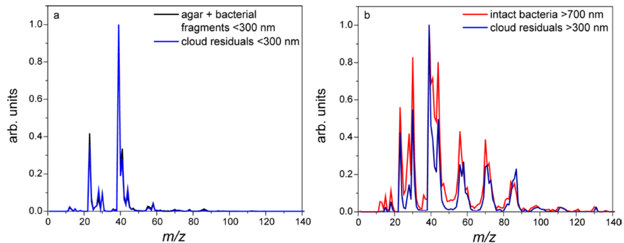
Figure S2: (a) Comparison between the MS of cloud residuals smaller than 300 nm and the reference MS of the small particle mode ( d_{va} < 300 nm); (b) Comparison between the MS of cloud residuals larger than 300 nm and the MS of intact bacteria ( d_{va} > 700 nm).
