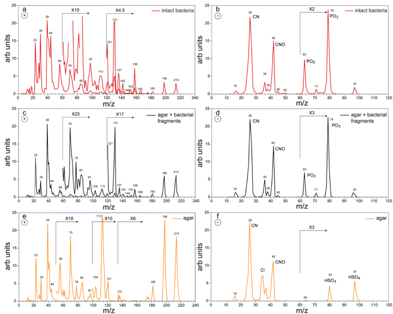
Figure S1: Positive (a) and negative (b) MS of intact Pseudomonas syringae bacteria measured before Expansion 1; Positive (c) and negative (d) MS of the small particles mode, measured before Expansion 1; Positive (e) and negative (f) MS of pure agar particles measured in a separate experiment.
