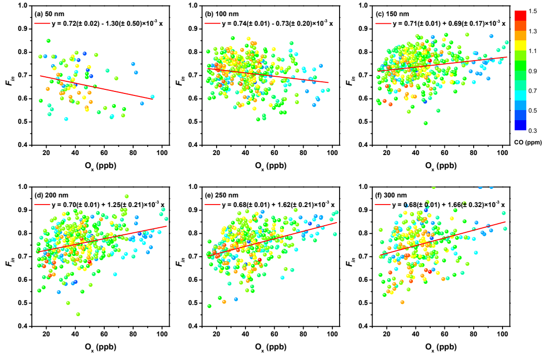
Figure 3: Correlation between the hourly-averaged number fractions of internally mixed BC ( F_{in} ) and the photochemical oxidant ( O_x ) mixing ratios for different size bins (50, 100, 150, 200, 250, and 300 nm). Data points are color-coded with respect to the concentrations of CO (an indicator of primary BC emissions). Low F_{in} values generally appear at high CO concentrations, and vice versa. For 150, 200, 250 and 300 nm diameters, F_{in} values increased with oxidant concentration. The slope of the linear regression (red line) is representative of the oxidation rate of F_{in} (the fit standard error is shown in brackets).
