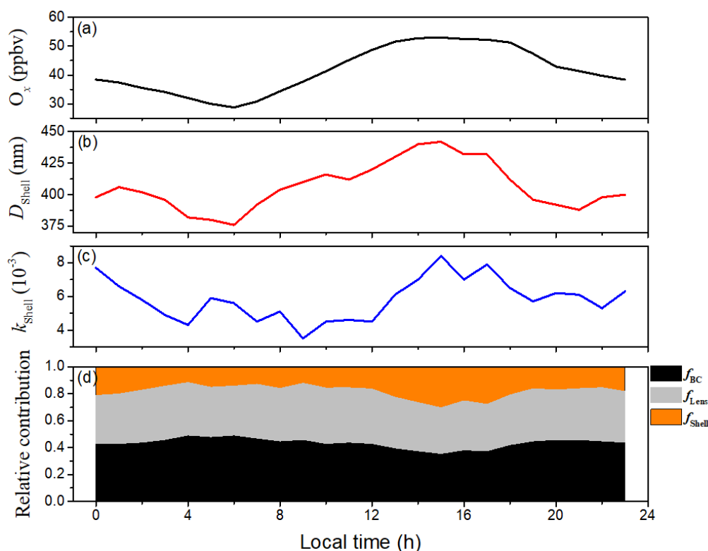
Figure 9: The retrieved diurnal variations of the (b) coating thickness ( D_{shell} ) and (c) imaginary part of the CRI ( k_{shell} ) of the coated materials, and (d) the relative contribution of the absorption of BC ( f_{BC} ), lensing effect ( f_{Lens} ), and absorption of the shell ( f_{Shell} ). Broadly similar patterns were observed for D_{shell} , k_{shell} , f_{shell} , and (a) O_x concentrations.
