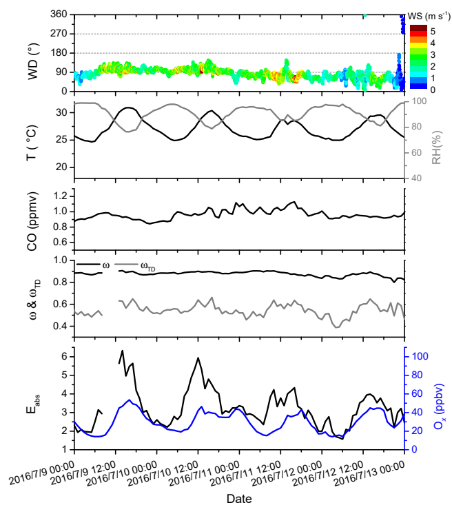
Figure S10: Time series of wind direction (WD, colored by wind speed (WS)), air temperature (T) and relative humidity (RH), CO concentrations, \omega , \omega_{TD} , E_{abs} and O_x concentrations for the four selected cases.
