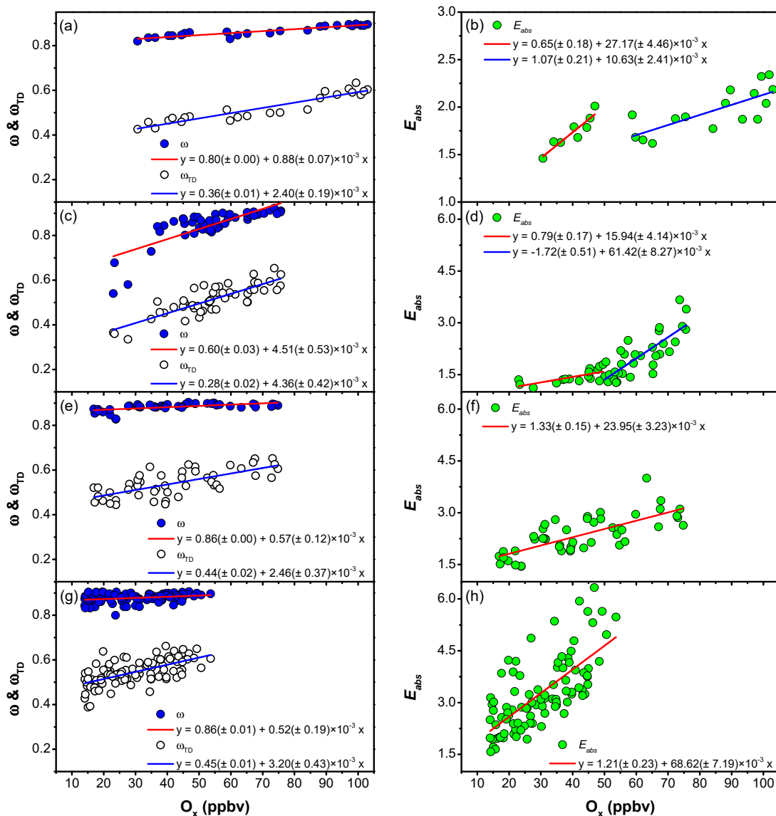
Figure 7: Four selected case study of the variations of hourly-averaged \omega , \omega_{TD} , and E_{abs} as a function of hourly-averaged O_x concentrations. (a,b) Case 1: on June 16, 2016, winds were typically from the north; (c,d) Case 2: June 25 to 26, 2016, winds direction varied from north to south.; (e,f) Case 3: July 7 to 8, winds were mainly from the southeast; 2016; and (g,h) Case 4: July 9 to 12, 2016, winds were mainly from the northeast. The slope of the linear regression (red and blue lines) is representative of the oxidation rate of each parameter (the fit standard error is shown in brackets).
