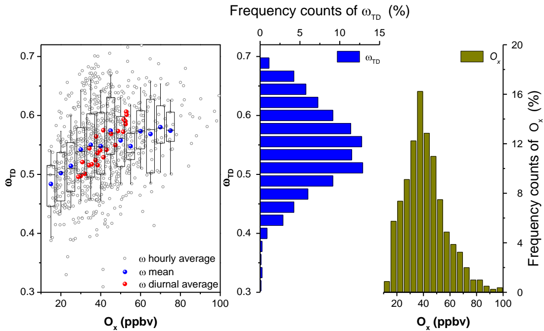
Fig. R3 Same as Fig. R1, the relationship between \omega_{TD} and O_x concentrations, and the frequency distribution of the measured \omega_{TD} and O_x .
