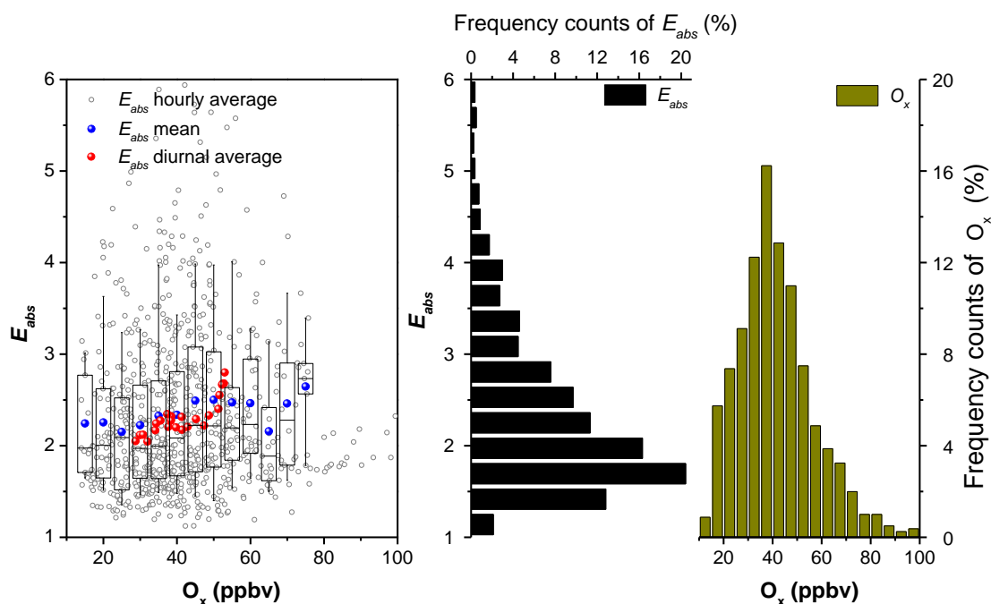
Fig. R1 Relationship between E_{abs} and O_x concentrations, and the frequency distribution of the measured E_{abs} and O_x . The gray circles are the measurement data with one-hour time resolution. The hourly averaged E_{abs} was then binned in O_x with bin size of 5 ppbv. The corresponding mean (blue solid dot), median (center solid line), lower and upper quartile (boxes) and 10 th and 90 th percentile (whisker) are shown as the box and whisker plots. The diurnal average data is shown as red solid dot for comparison.
