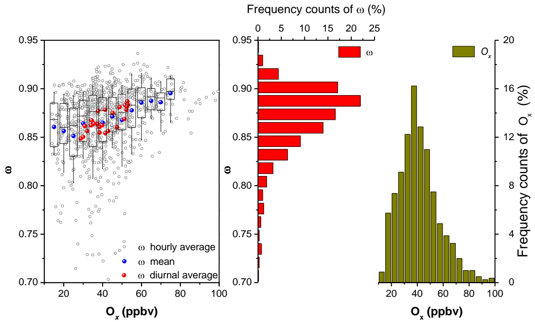
Fig. R2 Same as Fig. R1, the relationship between \omega and O_x concentrations, and the frequency distribution of the measured \omega and O_x .
