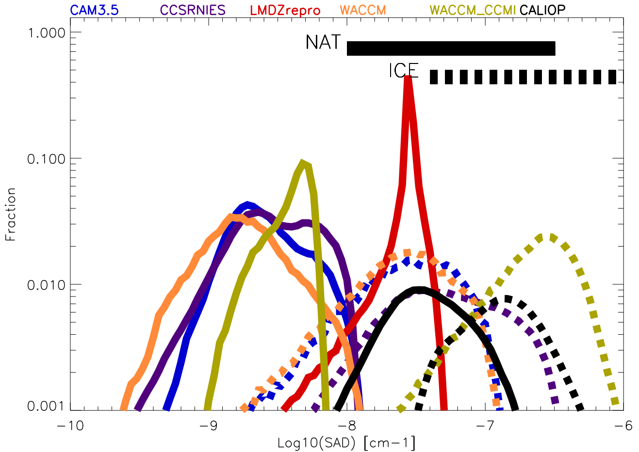
Figure 11. Histogram of the NAT (solid lines) and ice (dashed lines) SADs for some CCMVal models and for CALIOP are displayed. The histograms for the model data have been truncated and represent 93% of the total SAD. The straight lines at the top of the figure indicate the range of SAD values for NAT and ice “observed” by ground-based lidars and are taken from Adriani et al. (1995).
