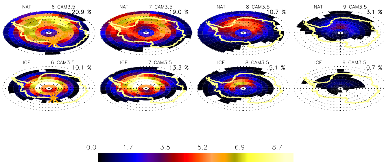
Figure 6. CAM3.5 PSCs vertical extent for NAT and ice, averaged over five years during the months of June, July, August, September (left to right). Please note that the color scale is different from the other maps. In the left column the location of McMurdo is indicated with a yellow asterisk. The fraction of the overall air volume (between 12 and 30 km height south of 60^{\circ} S) occupied by different PSC classes for each month is reported in the top right corner.
