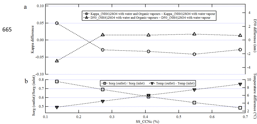
670 Figure 6. (a) Kappa and D_{50} difference of (\text{NH}_4)_2\text{SO}_4 particles measured with and without organic vapours in the sample and sheath air in the CCNc, (b) Temperature difference and the 675 corresponding calculated ratio of S_{\text{org}} between outlet and inlet of the CCNc under different SS.
