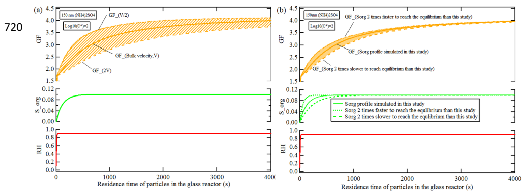
725 Figure 9. Simulated GF with residence time for organics with \log_{10}(C^*)=2 : sensitivity to (a) axial variability; (b) radial variability.
