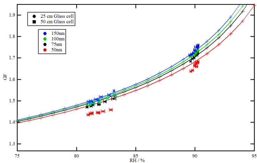
Figure 2. GF of (\text{NH}_4)_2\text{SO}_4 particles after transit through the 0.25 and 0.5 m glass reactor containing NaCl- \text{H}_2\text{O} solution with the water activity at 0.9.
