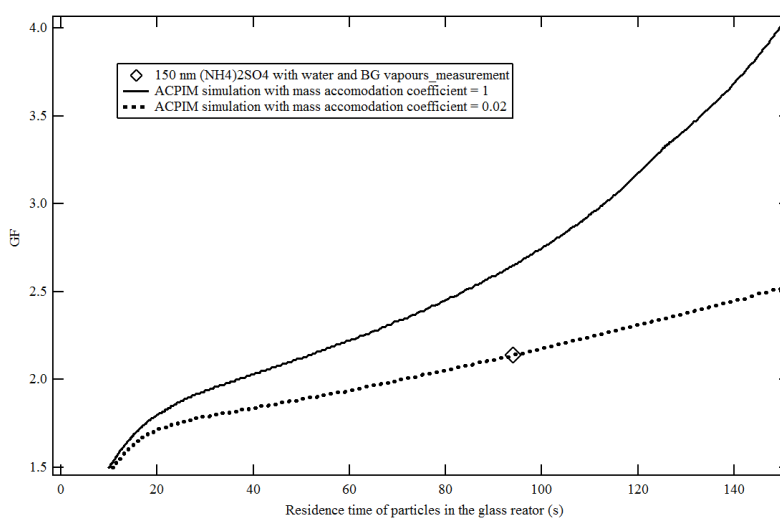
690 Figure 7. Measured and simulated GF with residence time for (\text{NH}_4)_2\text{SO}_4 particles exposed to water and BG vapours.
