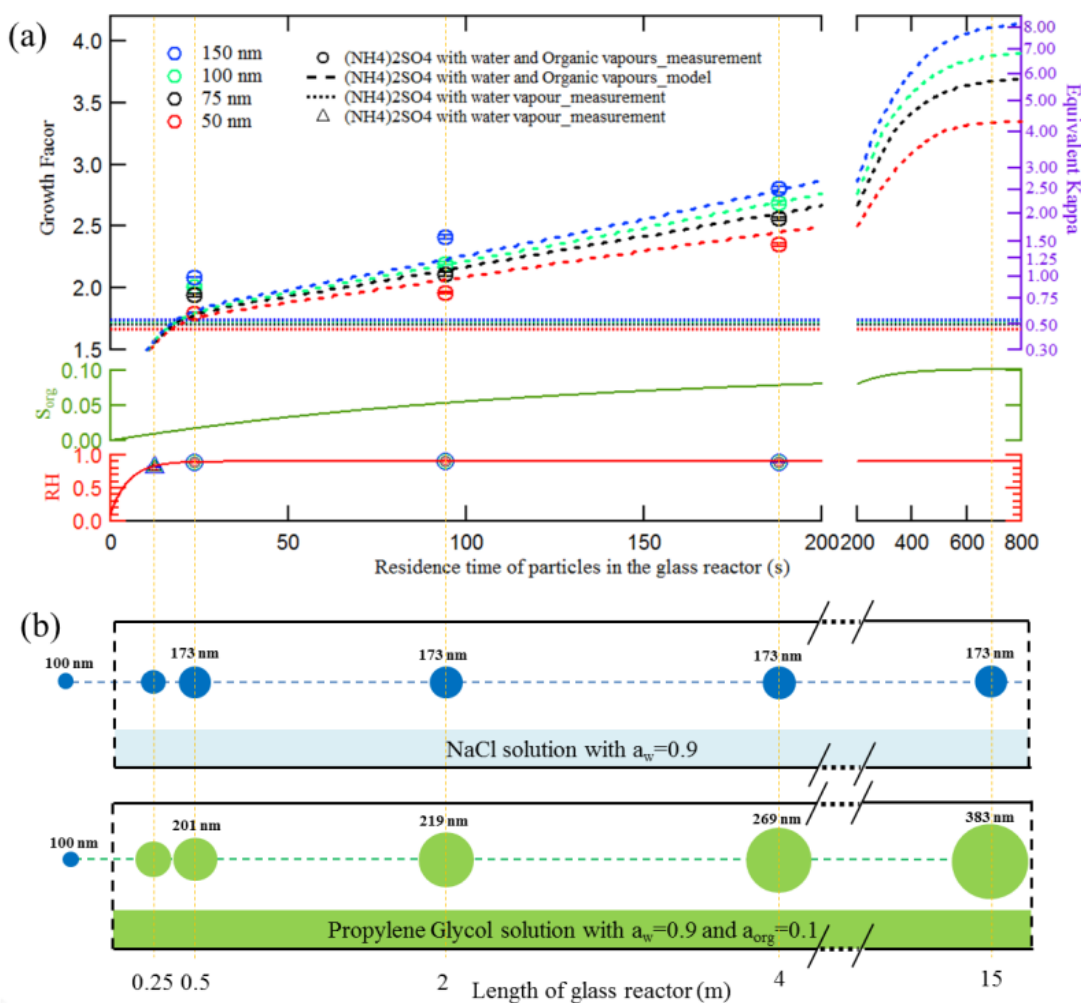
Figure 4. Growth of (\text{NH}_4)_2\text{SO}_4 particles exposed to water and propylene glycol, PG, vapours. (a) Measured (circle) and simulated (dash line) GFs with the residence time, the equivalent hygroscopicity (the \kappa that an involatile particle would need in order to show the growth factor in the absence of co-condensing vapours) corresponding to the GF axis is presented on the right hand axis of the top panel, the simulated RH and S_{\text{org}} profile are presented as solid red line and green line. (b) Schematic illustration of 100 nm (\text{NH}_4)_2\text{SO}_4 particles growth in the glass reactor, particle diameters to scale.
