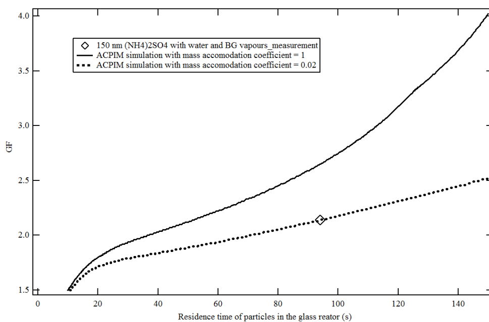
Figure 7. Measured and simulated GF with residence time for (NH 4 ) 2 SO 4 particles exposed to water and BG vapours.
