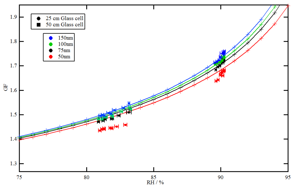
Figure 2. GF of (\text{NH}_4)_2\text{SO}_4 particles after transit through the 0.25 and 0.5 m glass reactor containing \text{NaCl-H}_2\text{O} solution with the water activity at 0.9.
