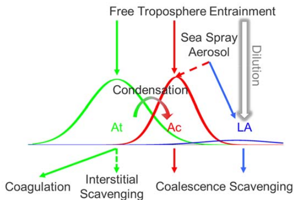
Figure 10. Concept model of key controlling processes of MBL aerosol number concentrations for each mode at ENA. Dash lines indicate the non-dominating but contributing processes. Negligible processes are not shown here.
