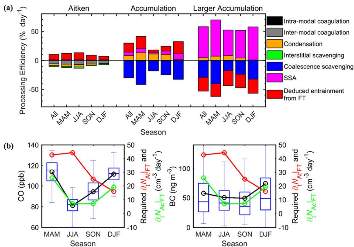
Figure 9. Major controlling processes for each mode. (a) Estimated secondary processing efficiency of each mode in different seasons. (b) Comparison of required seasonal-average FT entrainment rate to N_{At} and N_{Ac} , with CO and BC. The whiskers and boxes indicated the 90th, 75th, median, 25th and 10th percentile, respectively. The black circle and lines indicated overall means.
