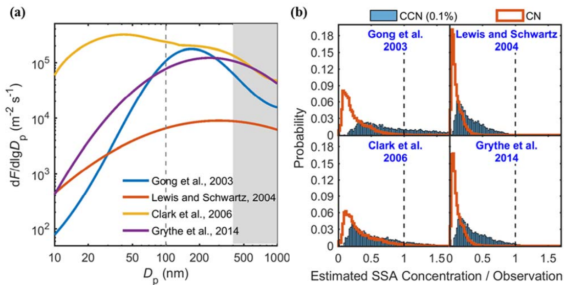
Figure 8. Estimation of SSA contributions to CN and CCN(0.1 %). (a) Previously published SSA production flux functions used here, and (b) SSA contribution to observed CN and CCN(0.1 %) estimated with each of the four SSA production flux functions.
