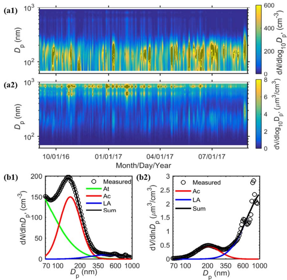
Figure 3. Representative aerosol size distribution measured at the ENA site. Time series of the (a1) number and (a2) volume size distributions during the study period from Sept. 2016 to Aug. 2017, and the fitted lognormal modes of (b1) number and (b2) volume distributions averaged over the one year period. The fluctuations at \sim 600 nm (also seen in Fig. 4) are considered as instrumental artefacts.
