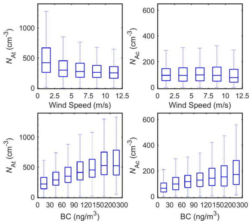
Figure 7. Dependence of N_{At} and N_{Ac} on WS and BC in 2015 to 2017. The whiskers and boxes indicated the 90th, 75th, median, 25th and 10th percentile, respectively.
