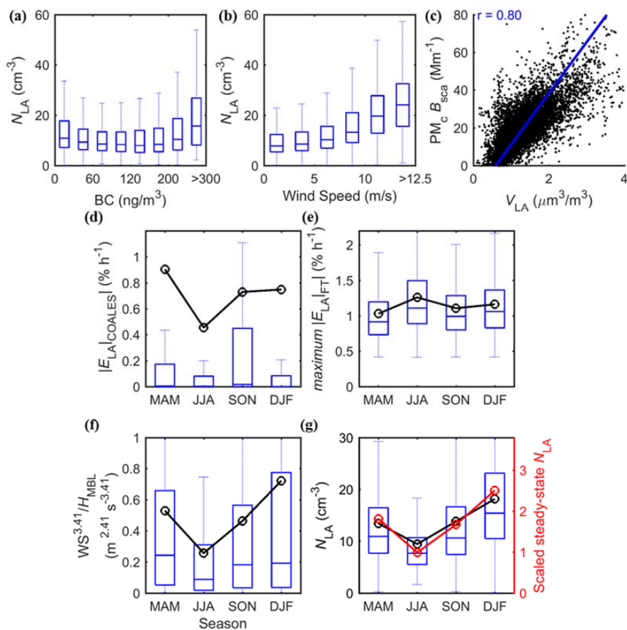
Figure 6. Evidences of key controlling processes of LA mode as SSA and coalescence scavenging. (a,b) Dependencies of N_{LA} with BC and WS for data in 2015 to 2017; (c) correlation between V_{LA} and \text{PM}_{C\_sca} for data in 2015 to 2017. The value of r given referred to the Pearson correlation coefficient, while the regression line based on York et al. (2004) is also shown for reference. (d,e) Estimated N_{LA} sinking efficiency due to (d) coalescence scavenging and (e) dilution of FT entrainment. (f) Indicators of the major N_{LA} source of SSA, and (g) the corresponding scaled ratios in comparison with observed N_{LA} seasonal patterns. Data shown in (d-g) are from Sept. 2016 to Aug. 2017. The whiskers and boxes indicated the 90th, 75th, median, 25th and 10th percentile, respectively. The black circle and lines indicated overall means.
