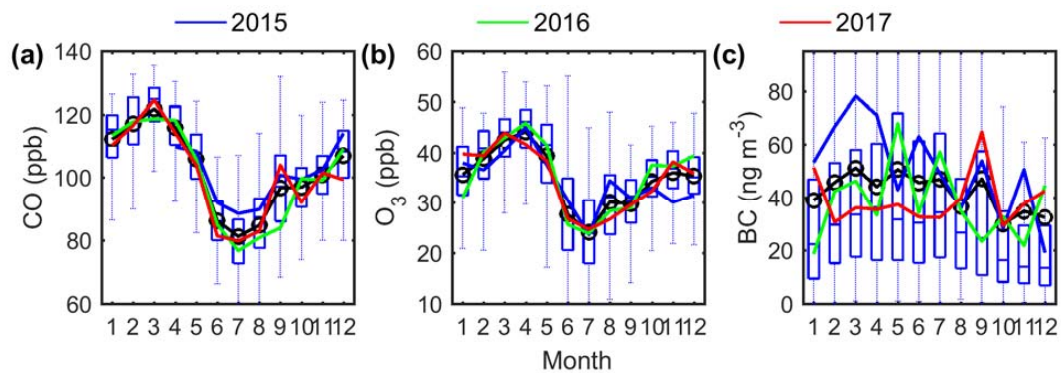
Figure 2. Seasonal variations of (a) CO mixing ratio, (b) O 3 mixing ratio, and (c) BC concentration at the ENA site. The blue, green, and red lines represent the monthly average for the year 2015, 2016, and 2017, respectively. The whiskers and boxes show the 90 th , 75 th , median, 25 th and 10 th percentiles, and the black circle and line represent the mean value of each month for the entire three years.
