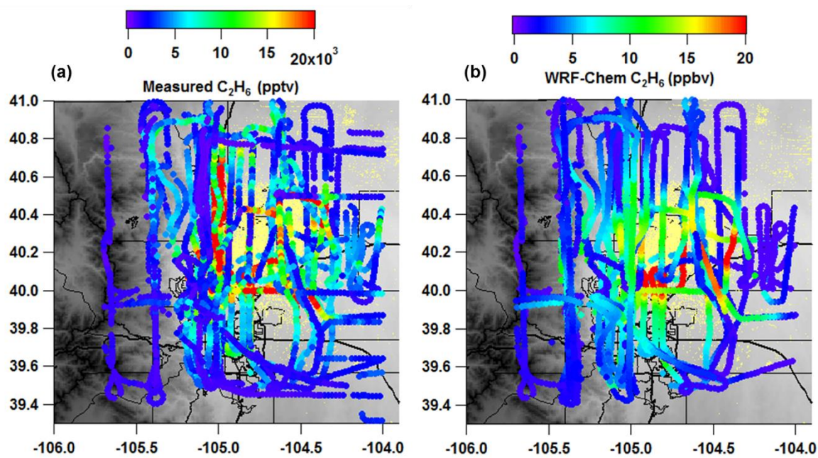
Figure S3. Flight tracks of C130 in the Front Range BL, color coded with ethane values from measurements (a) and BC-tdOG scenario (b). Locations of the O&G wells are shown with yellow dots.
