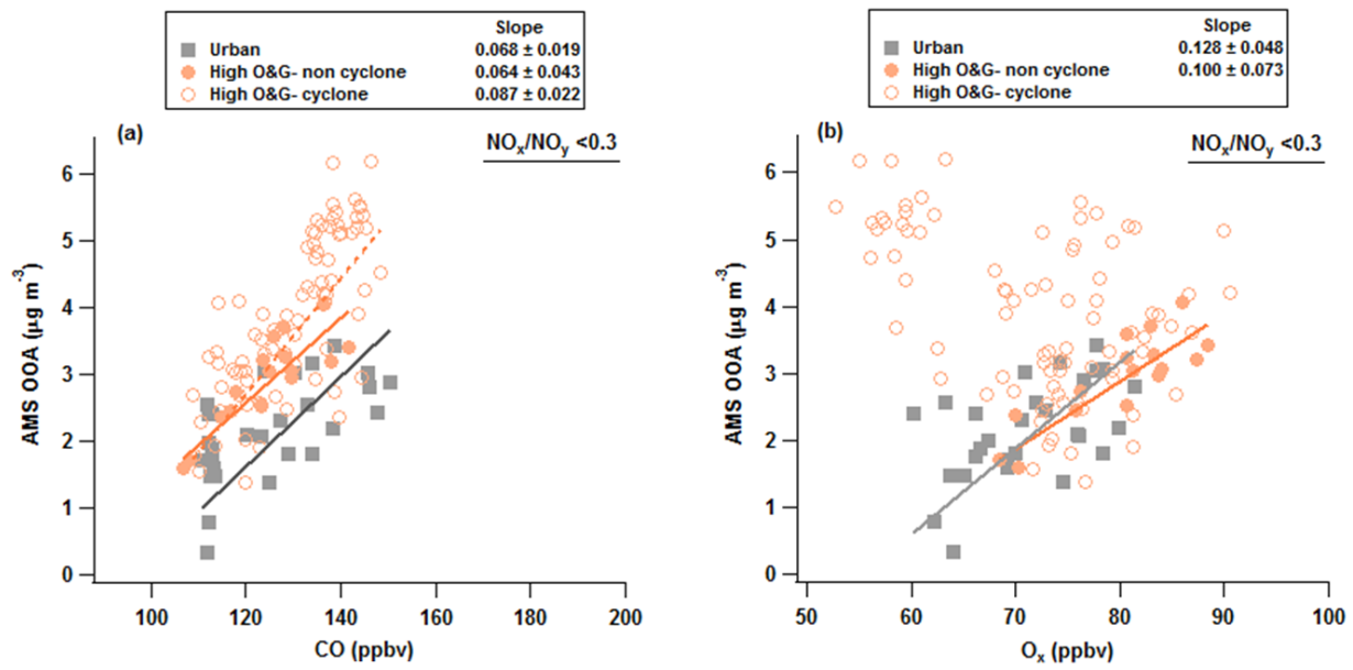
Figure S2. Correlation plots of PMF-derived OOA vs. CO (a) and odd oxygen, \text{O}_x defined as \text{O}_3 + \text{NO}_2 (b) in aged plumes.
