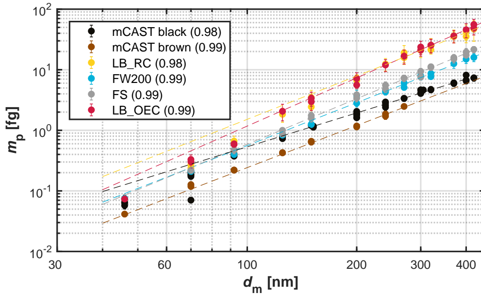
Figure 4. DMA-CPMA data for the different soot types: Electrical mobility diameter ( d_m ) vs. median particle mass ( m_p ) derived from fitting the resulting mass distribution with a log normal distribution. Error bars correspond to standard deviations of the individual measurements and dashed lines to the power law fits using eq.A4. The values in parenthesis give the R^2 of the fit.
