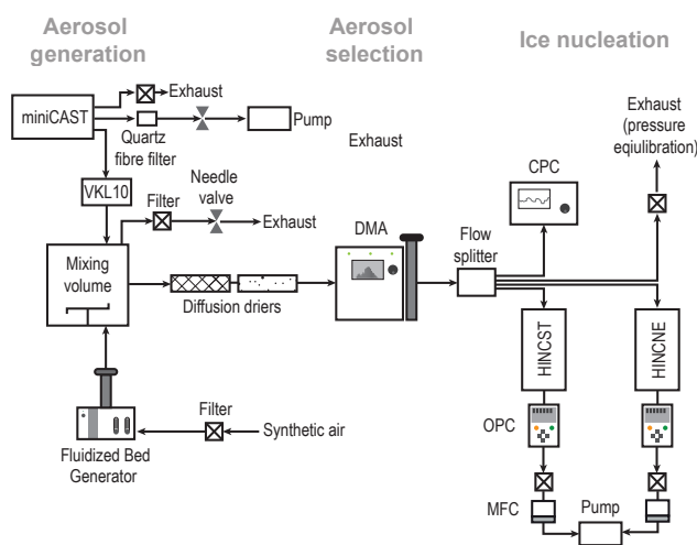
Figure 1. Schematic of the experimental setup comprising three different stages: aerosol generation, aerosol size selection and ice nucleation measurements. Arrows indicate the direction of the aerosol flow. Aerosol particles were either produced by the miniCAST burner or generated from the FBG. See text for details of instrument details and abbreviations.
