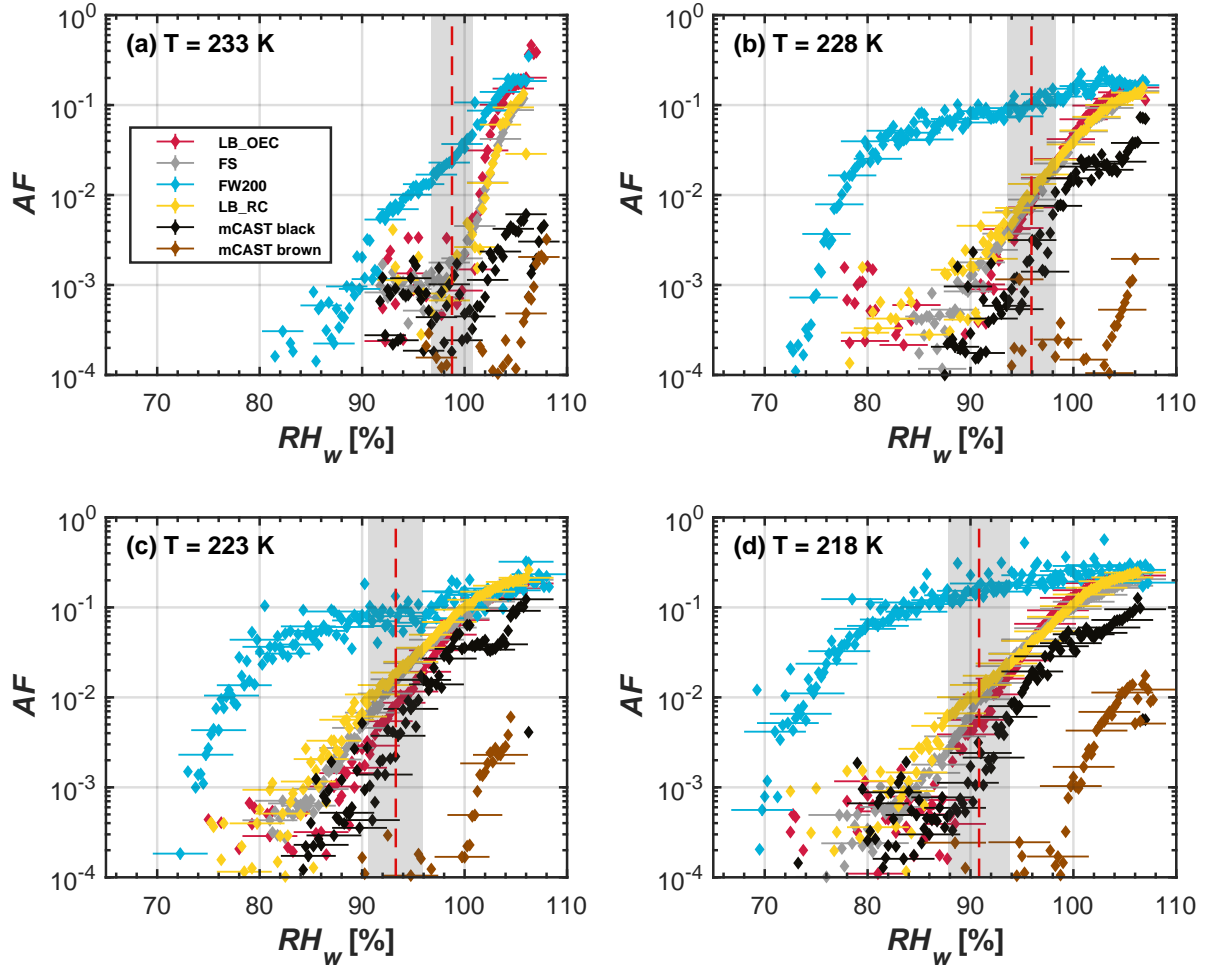
Figure 3. Mean RH scans of 400 nm mobility diameter soot particles, showing AF as a function of RH_w for different temperatures in the cirrus regime. Red dashed lines represent expected homogeneous freezing conditions according to Koop et al. (2000), and the gray shaded regions indicates the calculated RH_w variation across the aerosol lamina in HINC. Uncertainties, given for every 5 th data point, are as in Fig. 2.
