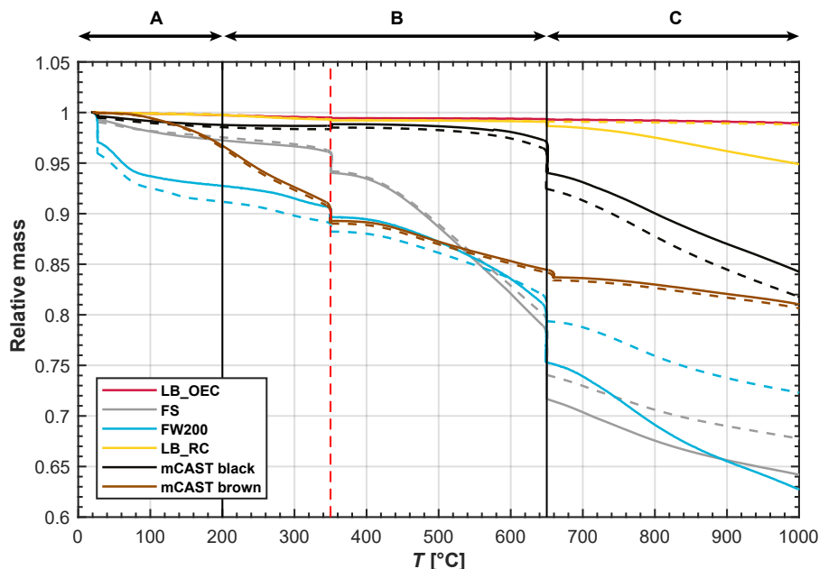
Figure 6. Results of the TGA analysis of the investigated soot types in a nitrogen atmosphere, showing the relative sample mass as a function of sample temperature. Solid and dashed lines indicate the results of two individual TGA runs. Indicated regions correspond to different ranges of volatilization, namely adsorbed water and highly heat sensitive material (A), medium heat sensitive material (B) and low heat sensitive material (C). Pyrolysis is expected to contribute to mass loss at temperatures above the vertical red dashed line.
