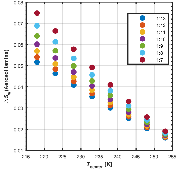
Figure D2. Relative humidity variation and uncertainty across the aerosol lamina, \Delta S_{w,\text{lam}} as a function of T_{\text{center}} for different ratios of F_{AP}/F_{\text{sheath}} within HINC. Each reported value denotes the maximum spread in S_w across the aerosol lamina considering all three cases of TC-temperature uncertainty (see text) and a center S_w value of 1.05. The work presented here used flow ratios between 1:10 and 1:12.
