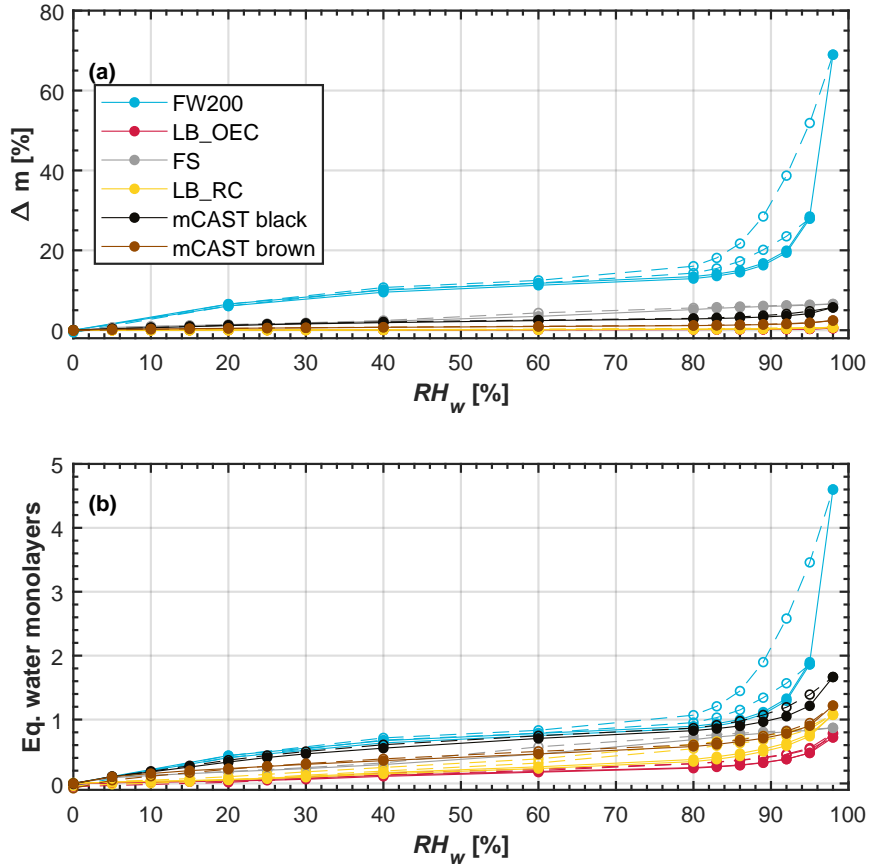
Figure 7. Water uptake (solid lines, filled symbols) and loss (dashed lines, open symbols) isotherms, given as (a) relative sample mass change and (b) equivalent water monolayers, as a function of RH_w , as measured by DVS at T = 298 K. Each set of curves corresponds to an individual, independent soot sample. The data points represent water uptake/loss at quasi-equilibrated RH_w conditions. Each soot type was probed for two independent experiments in the DVS and the curves of the two independent runs lie on top of each other. Exceptions are the mCAST samples, which were only probed once in the DVS. Curves are linear interpolations between quasi-equilibrated sample points to guide the eye. The curves of the LB_OEC and LB_RC samples lie on top of each other in panel (a). All experiments were performed to a maximum RH_w of 98 %, with the exception of one FW200 sample showing a maximum relative mass change of approximately 30 %, which was only probed up to RH_w = 95 %.
