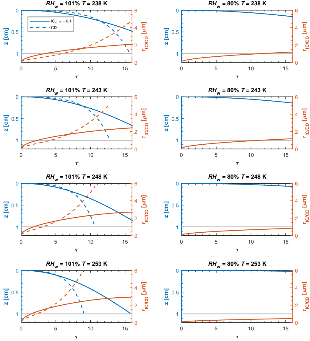
Figure D4. Expected diffusional growth and gravitational settling of spherical ice crystals (solid) and cloud droplets (dashed) for MPC temperatures, having an initial diameter of 200 nm. Symbols and reference lines as in Fig. D3.
