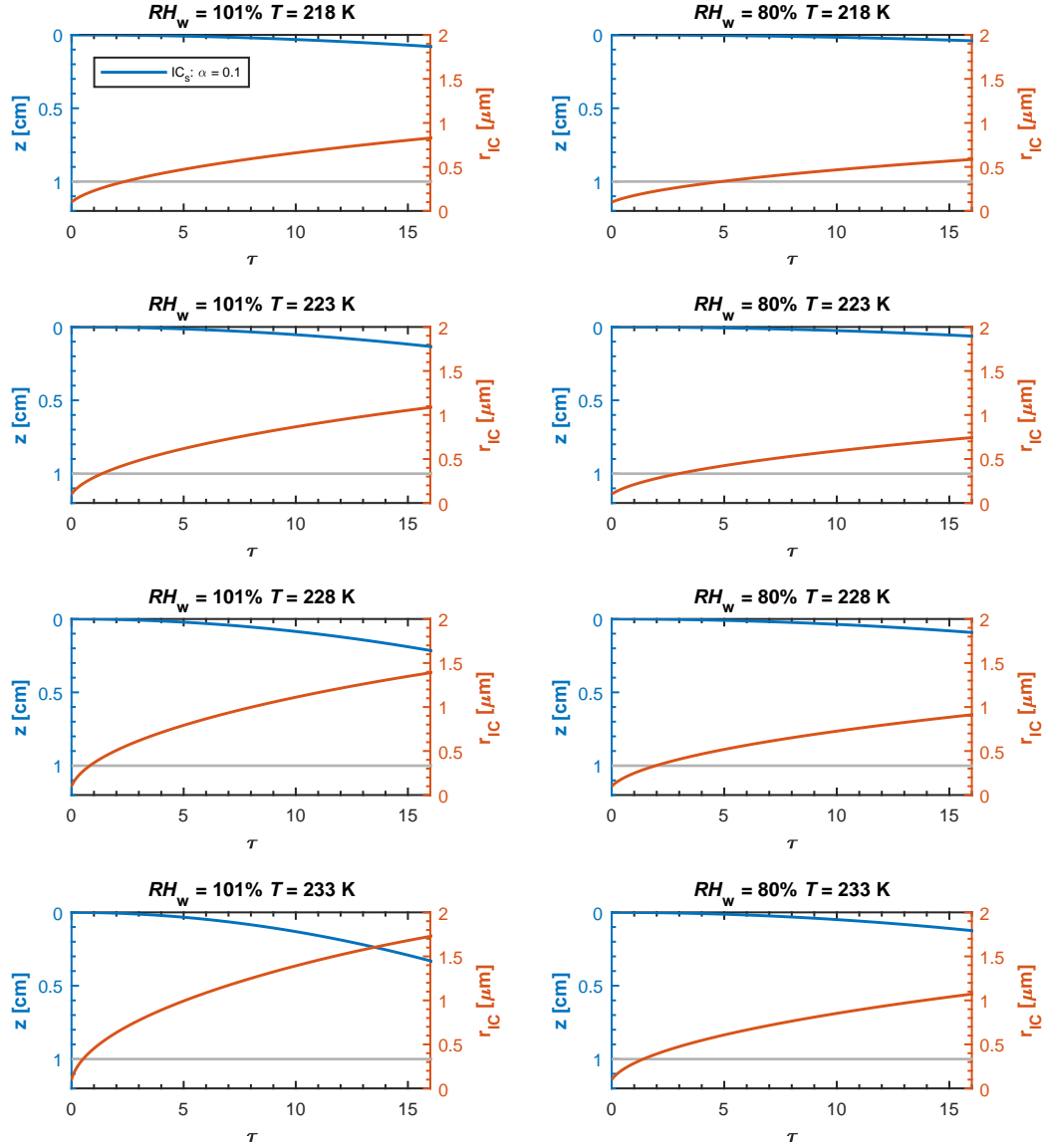
Figure D3. Expected diffusional growth of spherical ice crystals, having an initial diameter of 200 nm, within HINC for different cirrus regime temperatures, T_{center} , (rows) and RH_w along the centerline of HINC (columns), as a function of residence time. Orange lines indicate the ice crystal radius (right hand ordinate). Blue lines indicate the vertical distance covered by the ice crystal (left hand ordinate). Calculations are aborted, once a particle has traveled the half-distance of the two copper plates (1 cm), i.e. has hit the bottom plate of HINC, indicated by the horizontal, gray line (left hand ordinate), i.e. wherever any blue line crosses the horizontal gray line.
