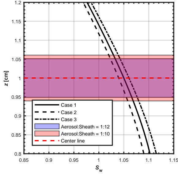
Figure D1. Example of S_w profile for the mid-portion of the vertical distance between the cold (at z = 0 cm, bottom) and warm (at z = 2 cm, top) wall of the HINC chamber, illustrating the variations in S_w across the aerosol lamina (black solid line) for exemplary conditions of T_{center} = 218 K, S_{w,center} = 1.05 and different F_{AP}/F_{sheath} flow ratios (red and blue shading). The S_w profiles given by the dashed and dash-dotted lines take into account uncertainty in temperature control arising from the thermocouples. The red dashed line indicates the position where particles are injected into HINC.
