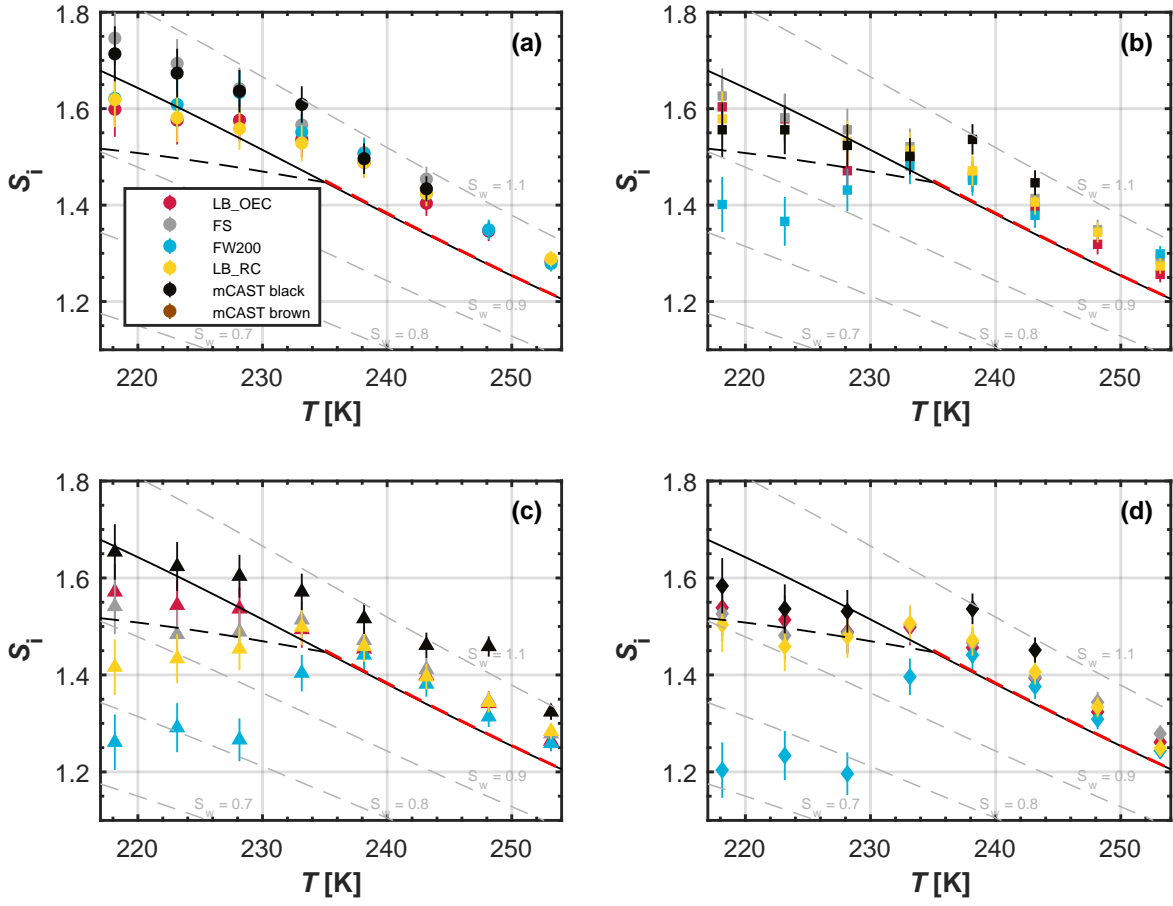
Figure 2. Onset saturation ratio with respect to ice ( S_i ) of freezing where 1 % of the aerosol particles are activated as a function of temperature for size-selected particles with mobility diameter of (a) 100, (b) 200 (c) 300 and (d) 400 nm (see SI Sect. S6). The black, solid lines denote water saturation using the water saturation pressure parameterization given by Murphy and Koop (2005); gray, dashed lines indicate offsets from this line in steps of 0.1 to guide the eye. The black, dashed lines mark the homogeneous freezing threshold for supercooled solution droplets according to Koop et al. (2000). The red dashed line indicates WDS conditions. WDS appears close to water saturation for the 1 \mu\text{m} OPC channel used. Each dot represents the mean of a minimum of two RH -scans performed with HINC. Temperature uncertainty is 0.1 K and S_i uncertainties, outlined in Appendix D1, are indicated as vertical bars. We note that mCAST black and brown do not activate to 1 % and are thus not plotted for some conditions (see SI Sect. S2 for complete AF curves).
