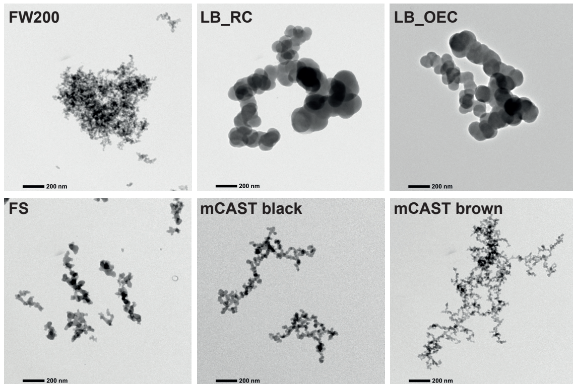
Figure 5. Exemplary TEM images of representative soot aggregates of the different soot types when selecting 400 nm mobility diameter particles with the DMA.
