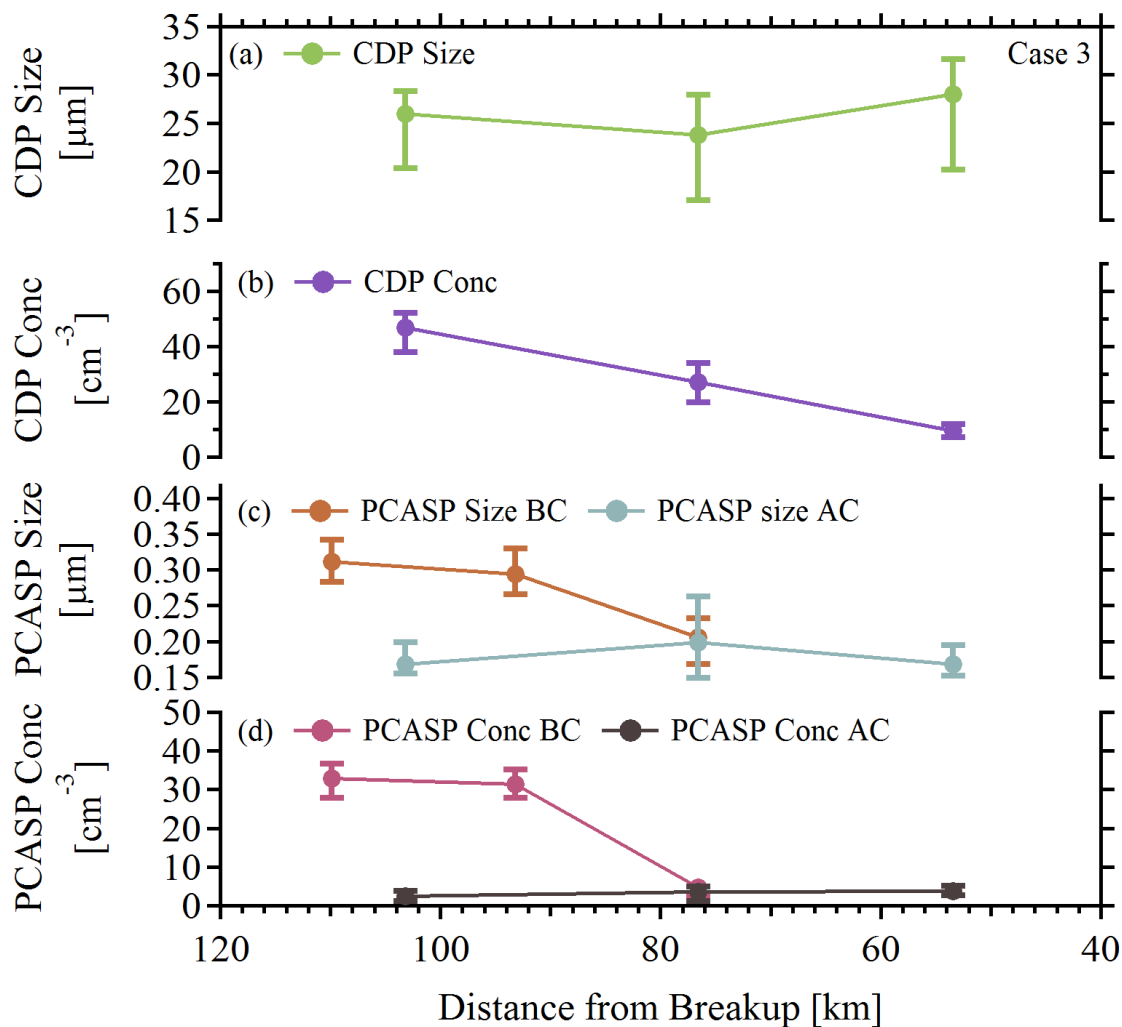
Figure 12: Median, 25th and 75th percentile values as a function of distance from breakup for CDP size, CDP concentration, PCASP size below cloud, PCASP size above cloud, PCASP concentration below cloud and PCASP concentration above cloud (case 3).
