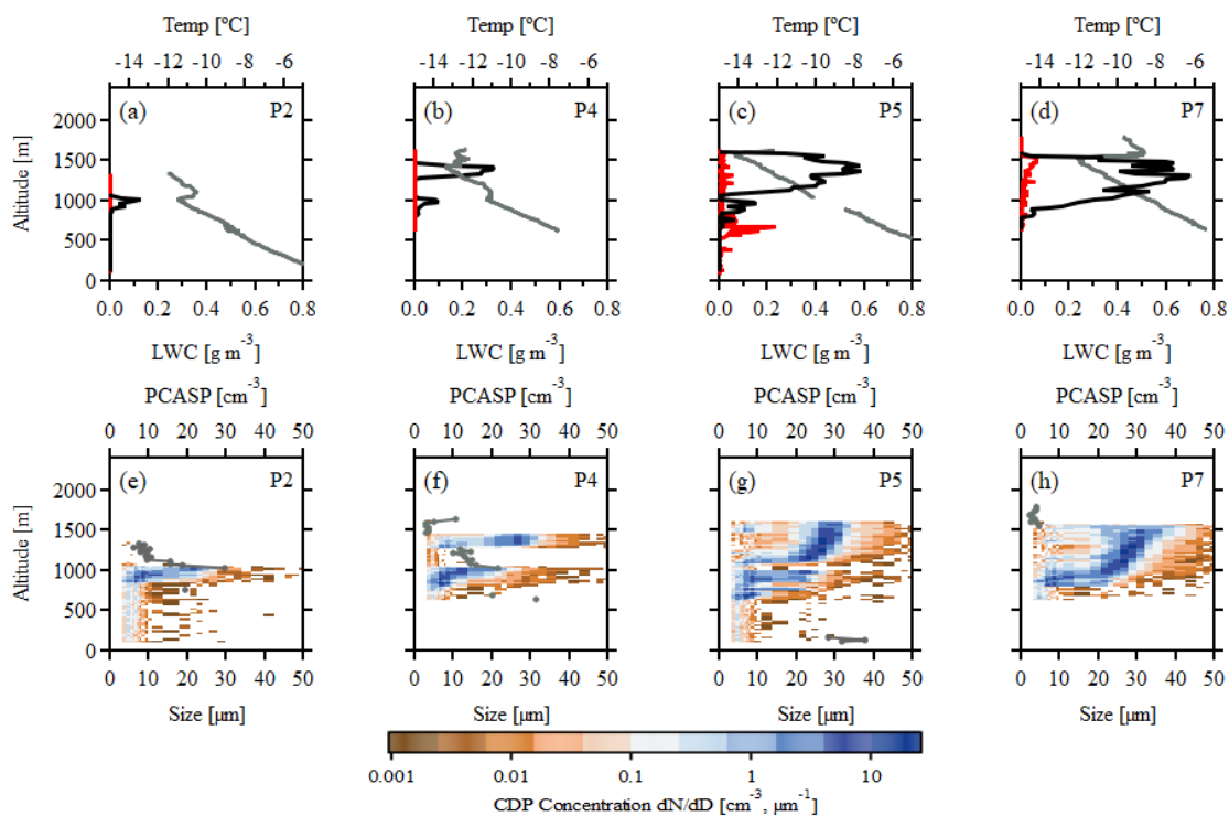
Figure 10. As fig. 5 but for profiles 2, 4, 5 and 7 for case 3.
