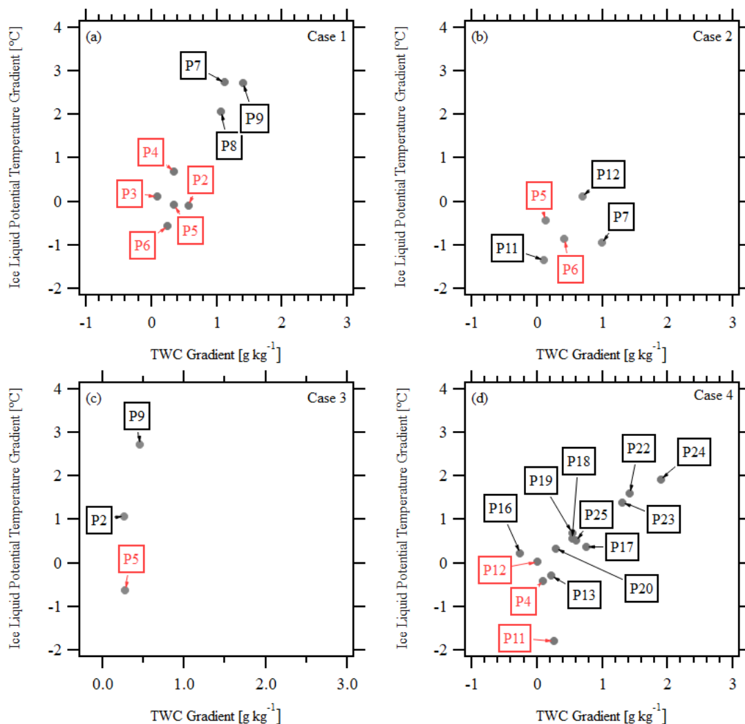
Figure 14: Gradients in \Delta\theta_l vs \Delta q_t for cases 1-4. Red profile number represent gradients within the stratiform boundary layer and black profile numbers represent gradients in transition or open regions.
