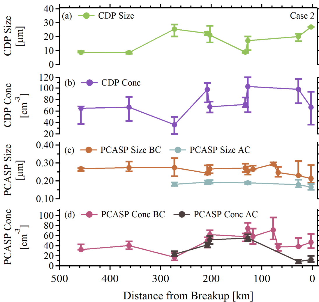
Figure 9: As fig. 6 but for case 2.
