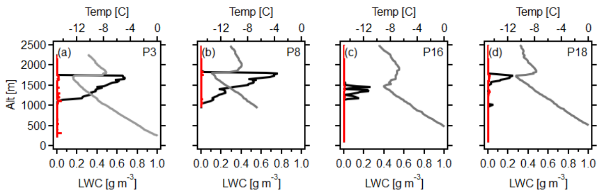
Figure 13: LWC (black trace) and temperature (grey trace) as a function of altitude for selected profile from case 4.
