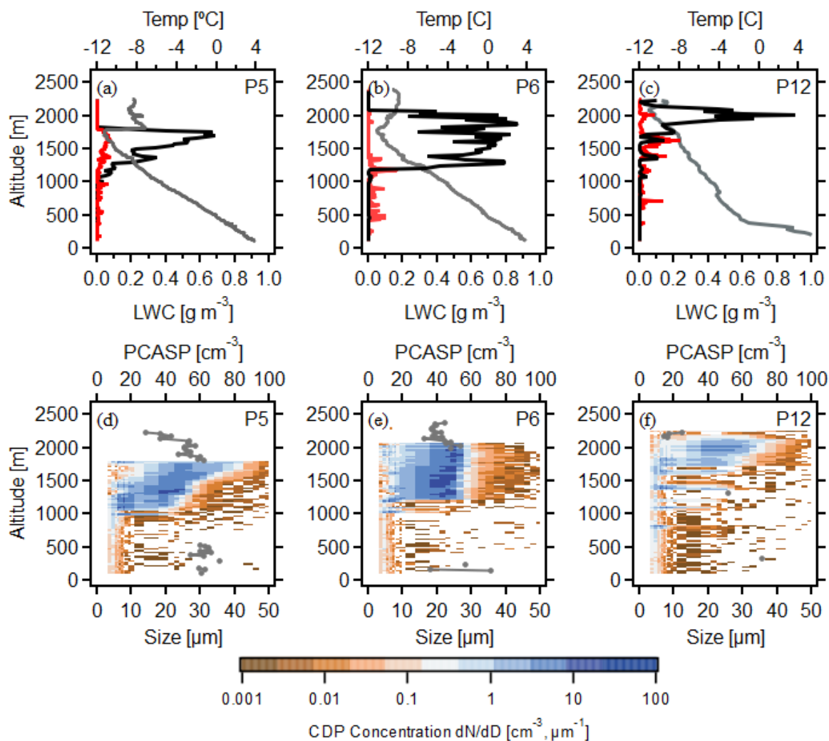
Figure 8: As Fig. 5 but for case 2.
