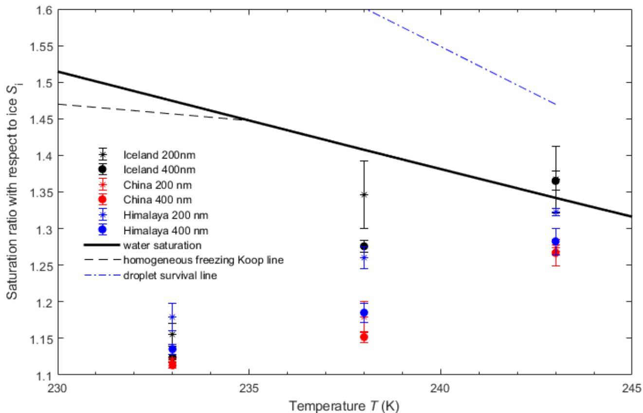
Figure 1: Average ice nucleation onset conditions ( AF = 0.1\% ) for each untreated dust and size. Error bars represent 1 standard deviation. Also shown are the water saturation line ( RH_w = 100\% ), the homogeneous freezing of solution droplets line (Koop et al., 2000) and the droplet survival line for PINC.
