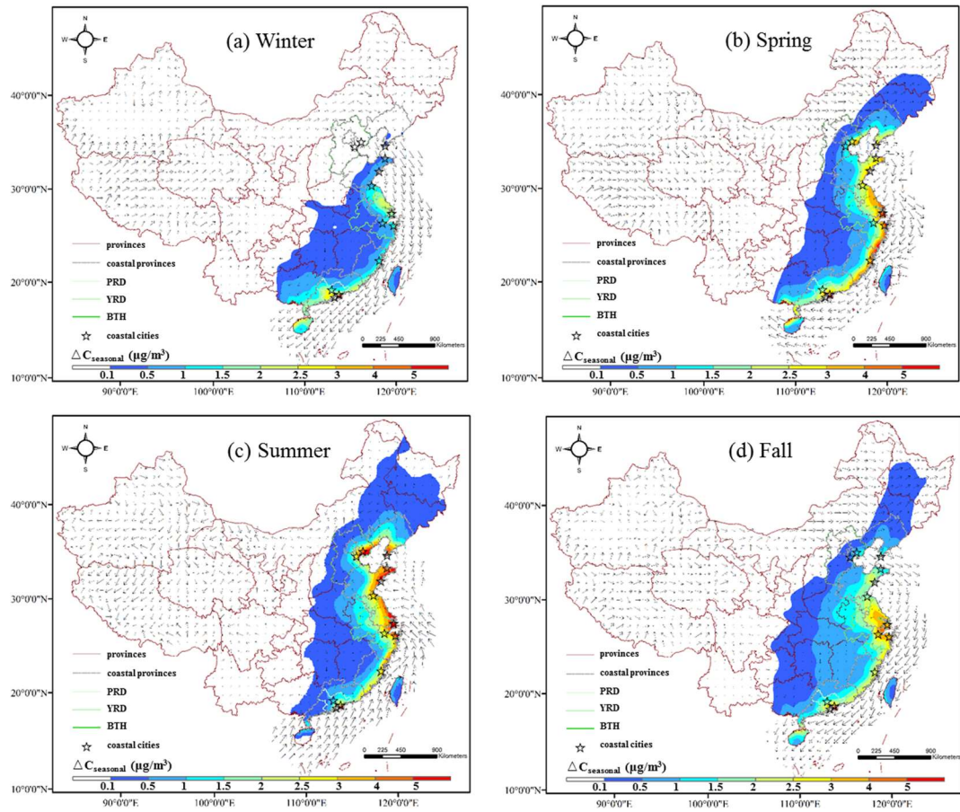
Fig 5: Contributions of shipping emissions to the seasonal mean PM 2.5 concentrations (base case- no ship case): (a) winter; (b) spring; (c) summer; (d) fall. Arrows represent the WRF modeled seasonal mean surface wind field.
