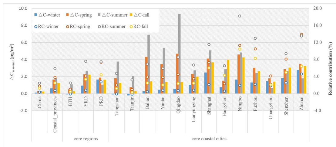
Fig 6: Contributions of shipping emissions to the seasonal PM 2.5 in core coastal regions and cities (base case- no ship case).
