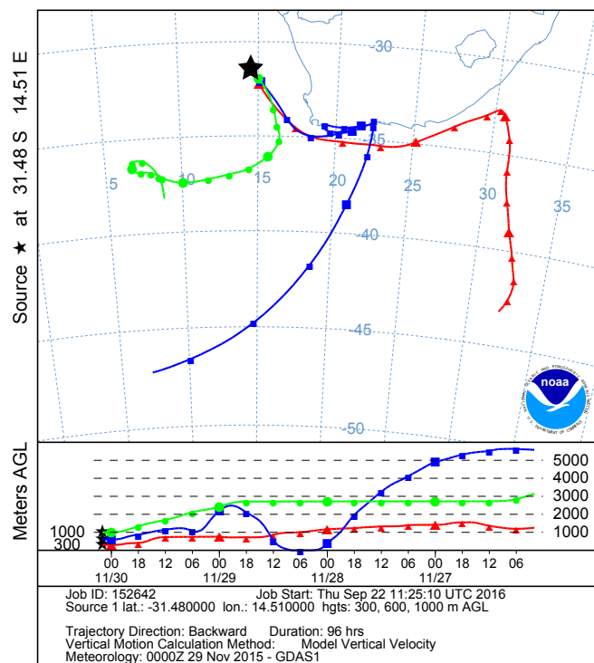
Figure 6. NOAA HYSPLIT backward trajectories for 4 days ending at the position of RV Polarstern (31.48°S, 14.51°E, marked by the black star) on 30 November 2015, 02:00 UTC at 300 m, 600 m and 1000 m AGL.
