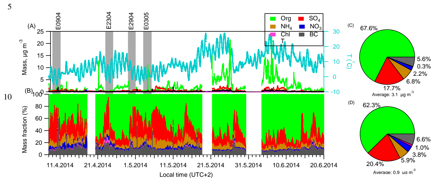
15 Figure 1: Time series and chemical composition of aerosol species determined by AMS in the campaign. The grey bars mark the four new particle formation events that this study focuses on. (A): Ambient temperature (T) and time series of aerosol mass concentrations. (B): Mass fractions of each aerosol component to the total aerosol mass concentrations. (C): Right pie charts show the average chemical composition for the campaign periods and (D): for the four new particle formation periods. 20
