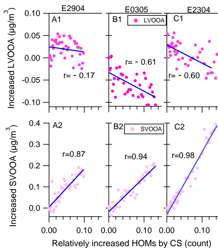
Figure 5: Comparisons of the increased mass of LVOOA (top panels) and SVOOA (bottom panels) in measurements (vertical axis) to the accumulated amount of HOMs condensed onto the particle phase (horizontal axis) at the particle growth stage (gray bars in Fig. 2). Note that AMS didn't work in E0904 growth period (event day of 9.4.2014) and thus the results are not shown.
