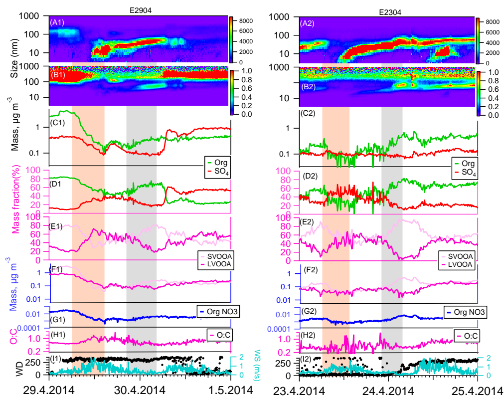
20 Figure 2: Observation of new particle formation events starting on 29.4.2014(E2904) and 23.4.2014 (E2304). The orange bars were marked for the analysis before and right after nucleation and the gray bars were for aerosol growth periods. Panels: (A) aerosol number size distributions from DMPS; (B) volume size distributions from DMPS; (C) mass concentrations of organic (green) and sulfate (red) species by AMS; (D) mass fractions of organic and sulfate to total aerosol mass concentrations; 25 (E) mass fractions of LVOOA (pink) and SVOOA (light pink) to total organic aerosol mass concentrations; (F) mass concentrations of LVOOA and SVOOA species determined by PMF; (G) the time series of organic nitrate aerosol; (H) O:C ratio of organic species by AMS; (I) wind speed (WS) and direction (WD).
