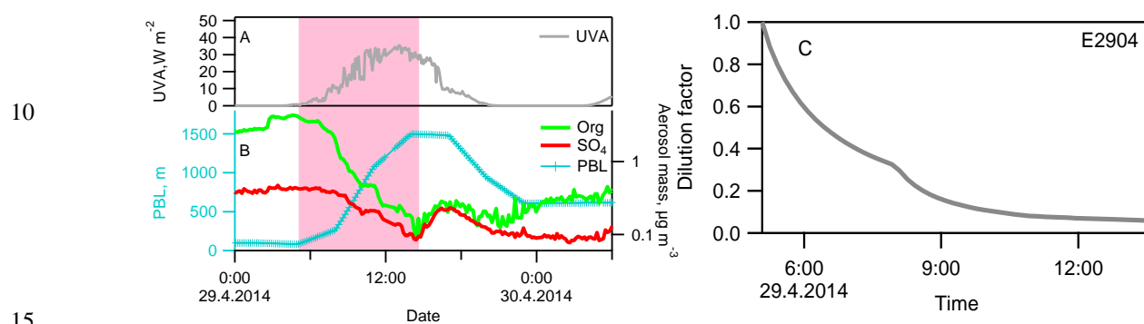
Figure 3: A closer view of the decrease of aerosol mass concentrations coinciding with PBL height development in E2904 (29.4.2014). (A) Ultraviolet (UV)-A radiation forcing; (B) the height of PBL and the mass concentrations of organic and \text{SO}_4 components measured by AMS; (C) dilution factor, estimated from PBL heights.
