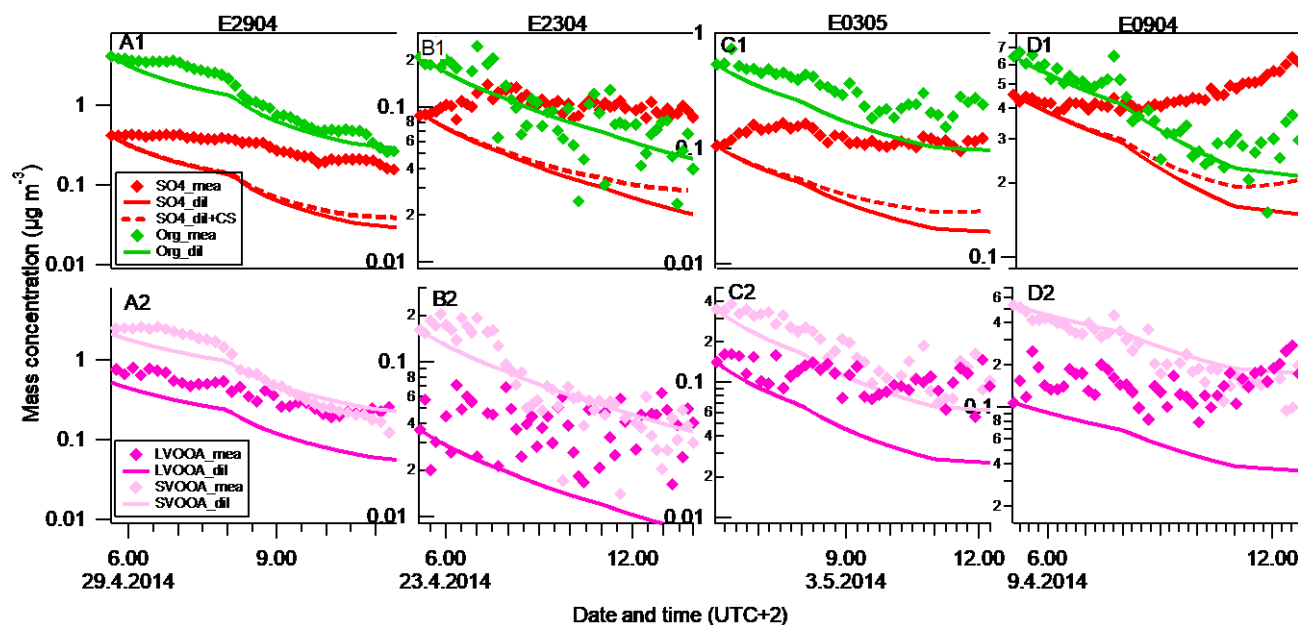
10 Figure 4: The time series of sulfate and organics (top panels), and LVOOA and SVOOA (bottom panels) aerosols depending on the dilution and vapor condensation effects before nucleation events in four events (orange bars in Figure 2). Diamond markers: the measured aerosol concentrations. Solid lines: the modelled aerosol concentrations assuming PBL heights to be an only controlling factor on aerosol mass concentrations. The aerosol concentrations were calculated by accounting for the air volume varying with PBL height. Dashed lines: the modelled aerosol concentrations accounted by both 15 the dilution effect and condensation of sulfuric acid.
