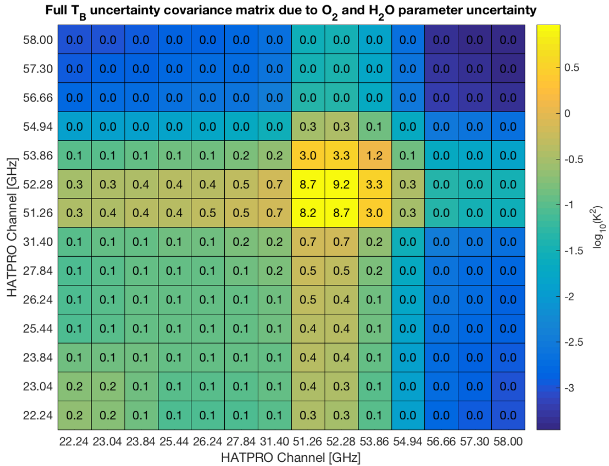
Figure 9: T_B uncertainty covariance matrix due to O_2 and H_2O absorption model parameter uncertainty at HATPRO channels for U.S. standard climatology. Numbers in the table are in K^2 , while the colour scale is in \log_{10}(K^2) .
