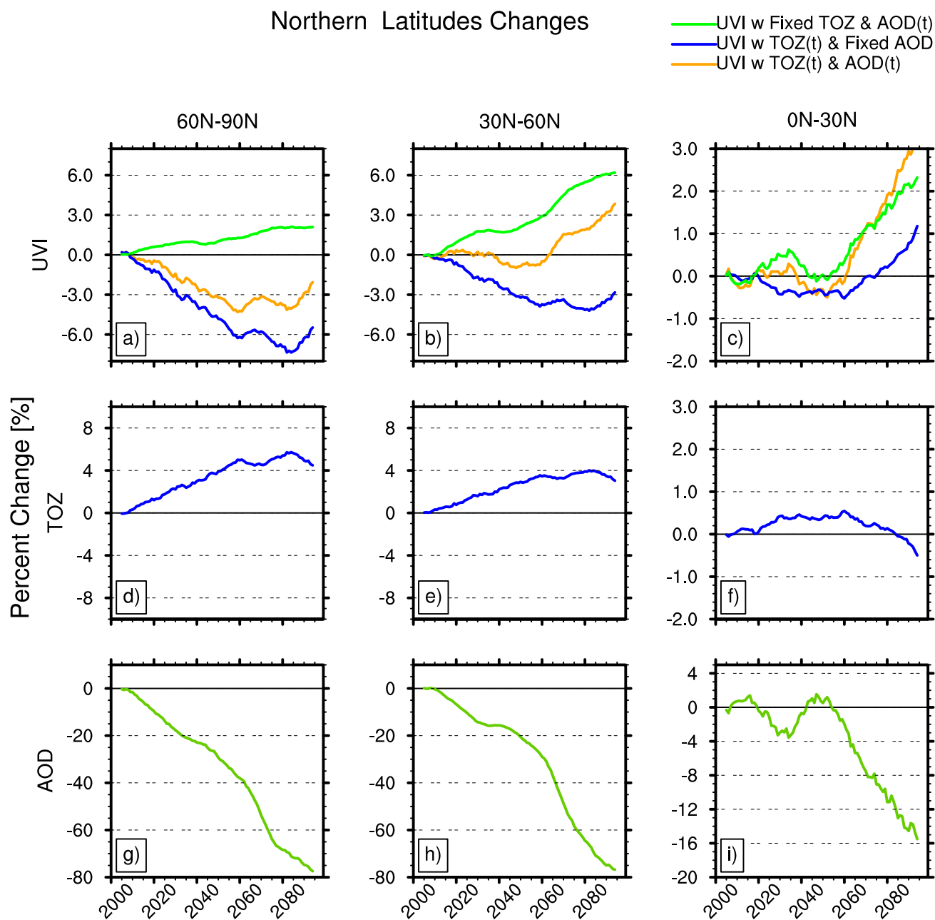
Figure 8. UVI, TOZ and AOD percent change from 2000-2010 values in the northern high, mid, and low latitudes for the EXP3 experiment. UVI modeled with transient TOZ and and AOD fixed at present-day climatological values are in blue. UVI modeled with TOZ fixed at present-day climatological values and AOD variable throught the 21st century are in green. UVI modeled with transient TOZ and AOD are in orange. TOZ and AOD are respectively in blue and green.
