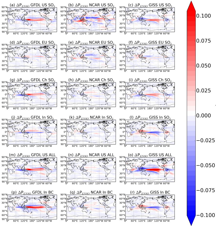
Figure 6: 200-year annual mean ENSO component of the precipitation response to aerosol emissions decreases in each of the three models (GFDL-CM3, first column; NCAR-CESM1, second column; GISS-E2, third column) for several different regional emissions decreases (simulations indicated in figure titles; see Table 1). See text for methodology.
