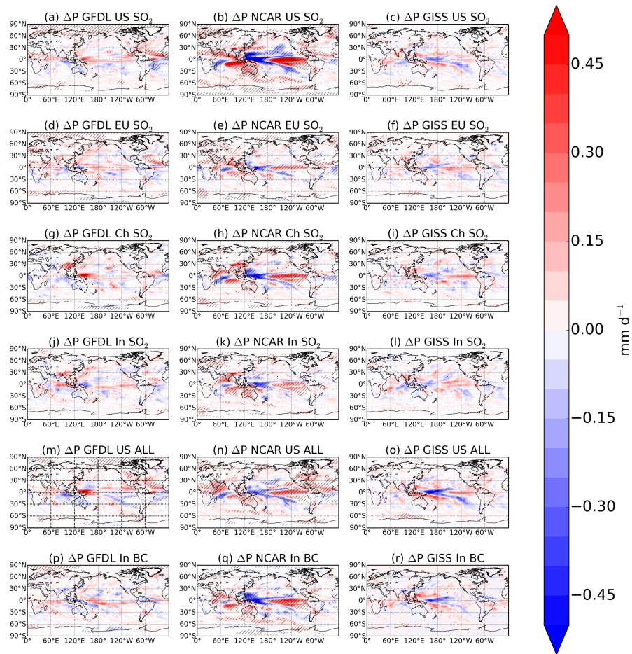
5 Figure 1: 200-year annual mean precipitation response to aerosol emissions decreases in each of the three models (GFDL-CM3, first column; NCAR-CESM1, second column; GISS-E2, third column) for several different regional emissions decreases (simulations indicated in figure titles; see Table 1). Hatching represents statistical significance at the 95% level according to a Student's t-test.
