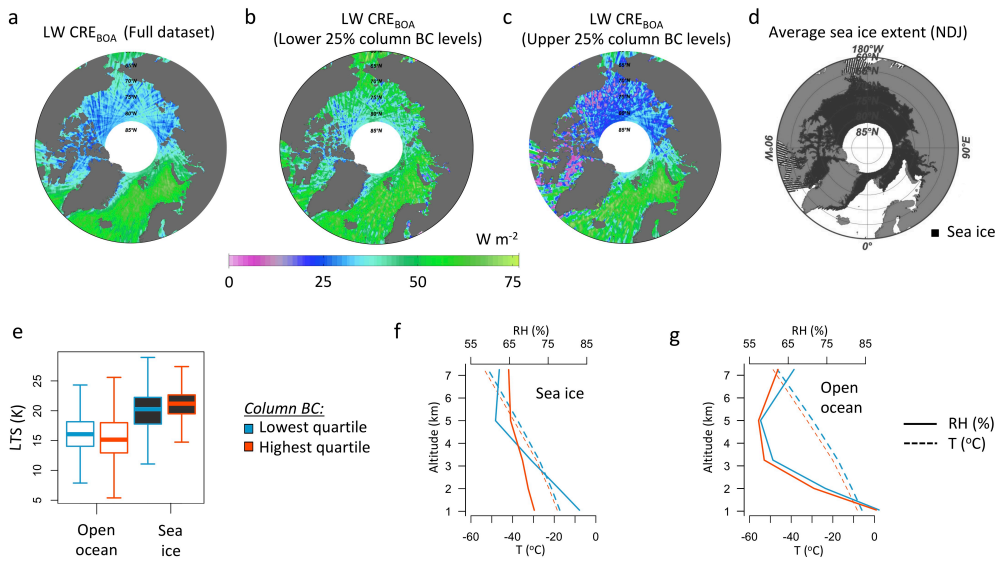
Figure 2: a-c) CloudSat FLXHR-LIDAR longwave cloud radiative effect at the bottom of atmosphere (i.e., surface) (LW CRE BOA ) during polar night for a) the full dataset, and the subsets of data containing the lower (b) and upper (c) quartiles of modeled column BC concentrations. For reference, d) shows the average winter (November to January) sea ice extent up to 82°N. Also shown are e) boxplots of the lower tropospheric stability (LTS, K), and f, g) the median temperature (T, °C) and relative humidity (RH, %) for the lower (blue) and upper (red) quartile column BC concentrations over open ocean and sea ice. All differences in e-g) are significant ( p < 0.0001 ), based on a Wilcoxon rank test.
