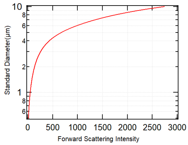
Figure S1: Calibration curve between forward scattering intensity and standard spherical particles' diameter
