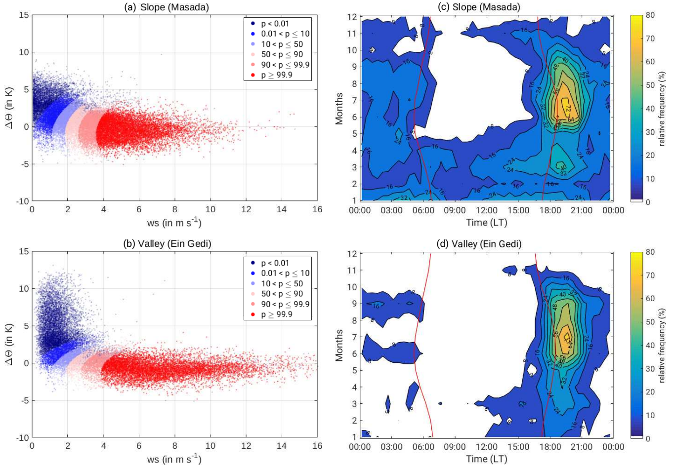
Figure 3. Left: Probability of foehn (colors) for wind velocity and potential temperature difference ( \Delta T = T_{crest} - T_{valley} , \Delta\theta = \theta_{crest} - \theta_{valley} ). The crest station is Jerusalem and the valley stations are Masada and Ein Gedi (Fig. 1). Right: Relative frequency of foehn occurrence with a detection probability of more than 75 %. Sunrise and Sunset are marked as red lines.
