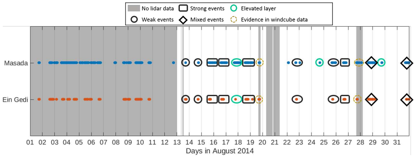
Figure 4. Occurrence of foehn in August 2014 at the slope (Masada, blue dots) and in the valley (Ein Gedi, red dots). Shown is the foehn occurrence with a detection probability of more than 75 %. Grey shaded area shows the dates were lidar data were not available.
