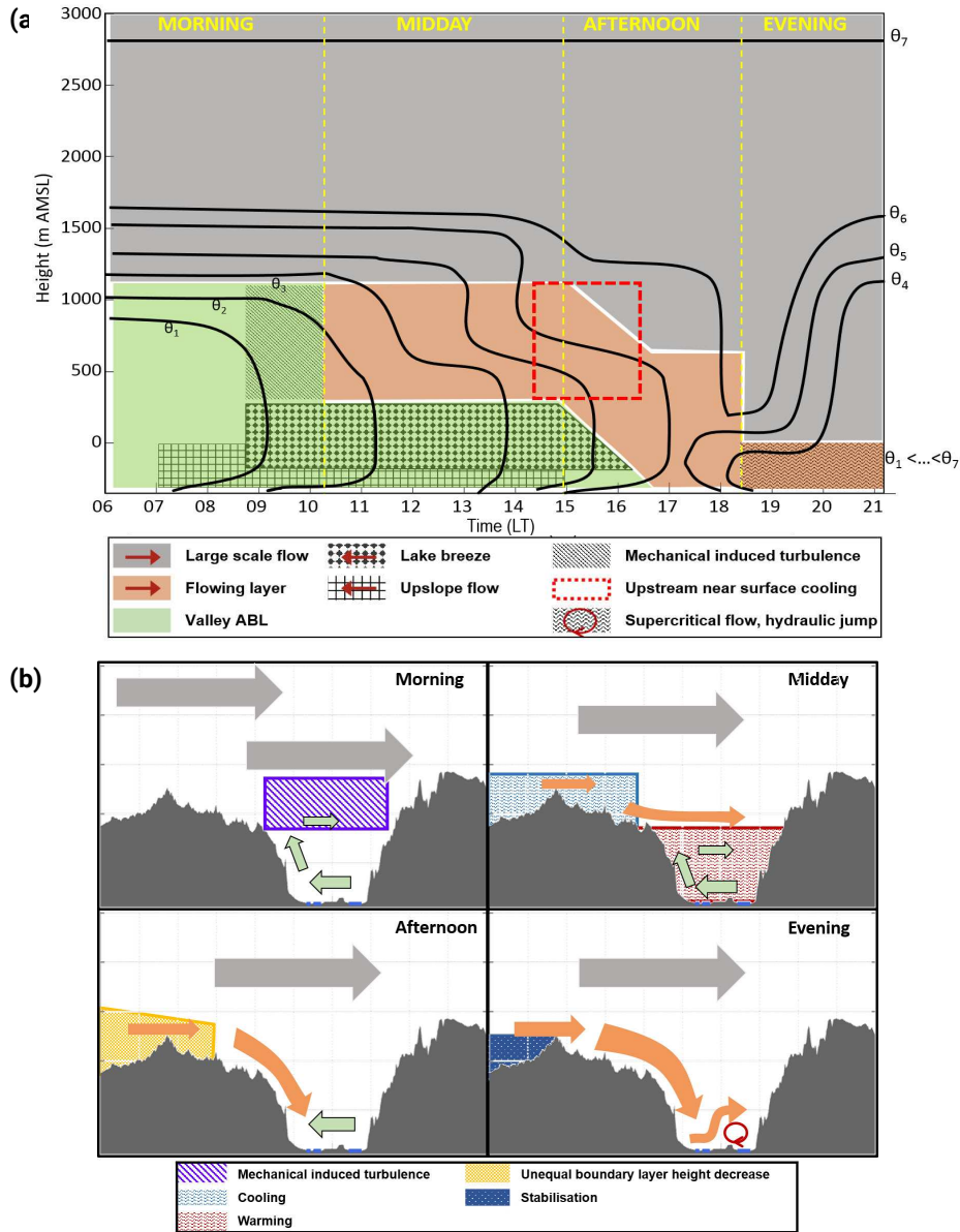
Figure 13. Conceptual model describing the different boundary layer processes in the valley on 16 August 2014. (a) The temporal evolution of the different layers and wind systems is given. The coloured areas refer to the distinct layers detected. Hatched areas describe distinct processes described in the text, and red arrows in the legend show the main wind direction in the respective layer. (b) The shows the wind systems (arrows) and the ongoing processes (shaded areas) leading to the next stage for morning, noon, afternoon, and evening, are shown in (b).
