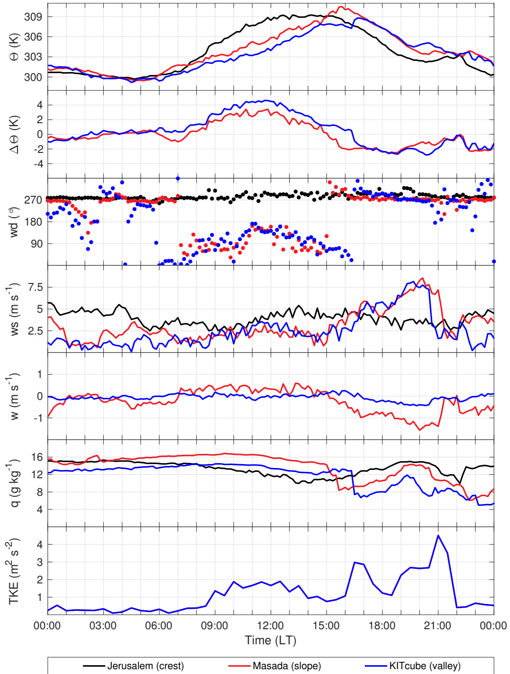
Figure 9. Time series of potential temperature ( \Theta ), potential temperature difference between crest and slope/valley ( \Delta\Theta ), wind direction ( wd ), wind speed ( ws ), vertical wind speed ( w ), specific humidity ( q ), and turbulent kinetic energy (TKE) for Jerusalem (crest), Masada (slope), and KITcube location (valley) on 16 August 2014.
