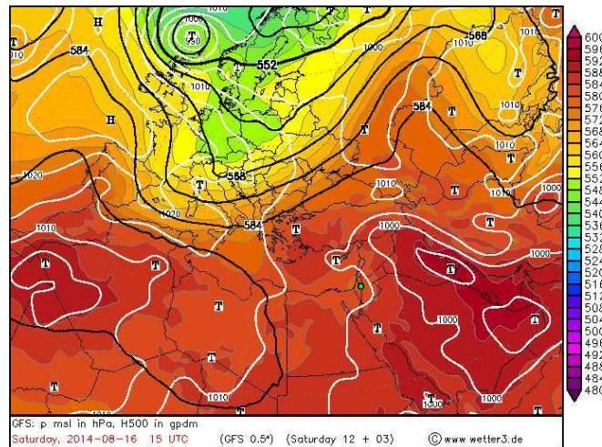
Figure 7. Large scale synoptic conditions on 16 August 2014, 15 UTC. Geopotential in gpdm at 500 hPa (black contours), surface pressure in hPa (white contours), relative topography 500/1000 hPa (coloured). Green dot indicates investigation area.
