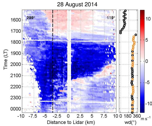
Figure 6. Example for a mixed event on 28 August 2014. Hovmoeller diagram of the near-surface radial velocity from lidar RHI scans at an azimuth angle of 299° and 7° elevation west of the lidar and 1.6° east of the lidar. The black dashed line indicates the end of the western slope and the beginning of the valley floor. Wind direction ( wd ) was measured in 40 m agl. Orange points highlight wind directions between 270 and 330°, the main wind direction of the foehn.
