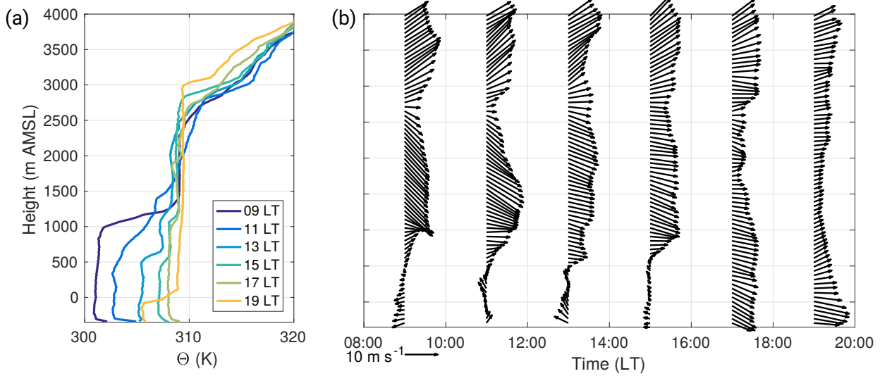
Figure 8. Potential temperature (a) and horizontal wind profiles (b), measured with radiosondes in the valley at the KITcube location. Data are shown for 16 August 2014.
