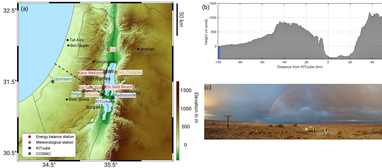
Figure 1. Topographic map of the research area with the measurement sites (a). Cross section along the dashed line in (a) is shown in (b), and a picture of the KITcube measurement site near Masada is shown in (c).
