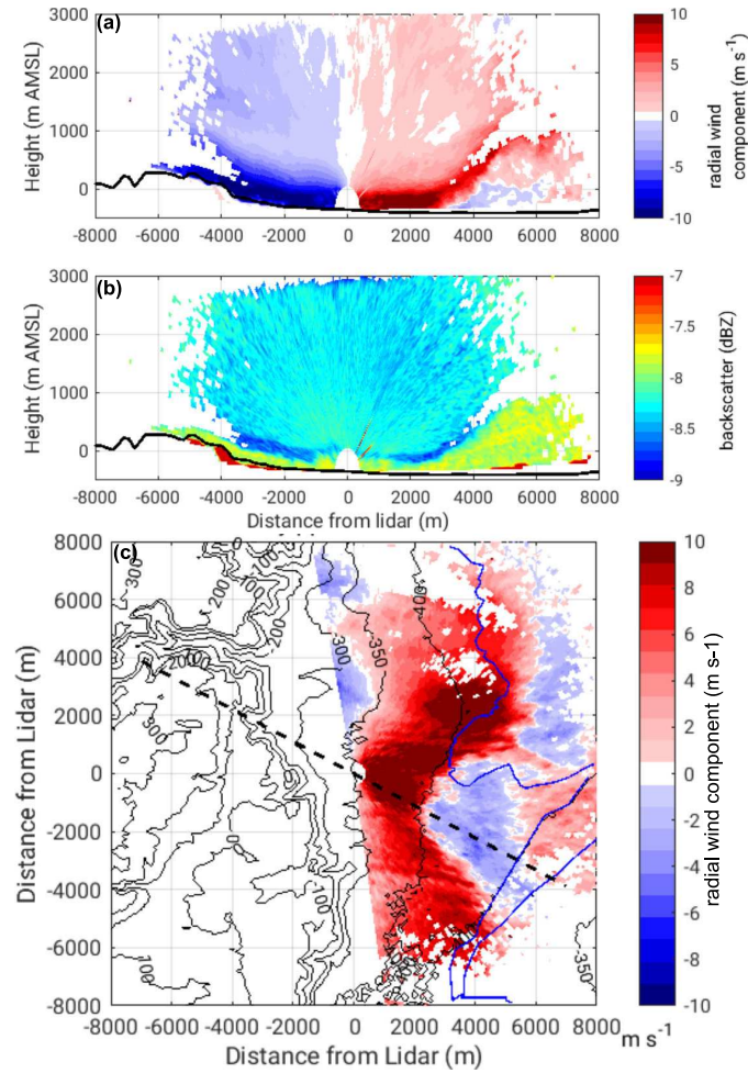
Figure 12. RHI scan at an azimuth angle of 299° (dashed line in (c)) showing radial velocity (a) and backscatter (b) on 16 August 2014, 19:36 LT. PPI scan at an elevation angle of 0.2°, shows radial velocity (c) at 19:51 LT. In (a) and (c) blue colours indicate a flow towards the lidar and red colours indicate a flow away from the lidar. The shoreline of the Dead Sea is indicated by a dark blue line in (c).
