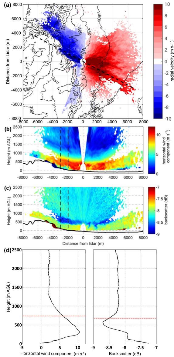
Figure 2. PPI scan of the radial velocity at 5° elevation on 16 August 2014, 19:01 LT (a). Blue colours indicate flow towards the lidar and red colours flow away from the lidar. The dashed line indicates the direction of the RHI scans of the horizontal component of the radial velocity shown in (b) and of the backscatter signal shown in (c) (note the different colour scales). RHI scans were performed on 16 August 2014, 19:06 LT. Vertical profiles of the horizontal radial wind velocity component and of the backscatter signal (d) averaged between the black dashed lines in (c). The red dashed lines indicate the foehn layer heights, automatically detected by the strongest vertical gradient of the respective profile above the maximum.
