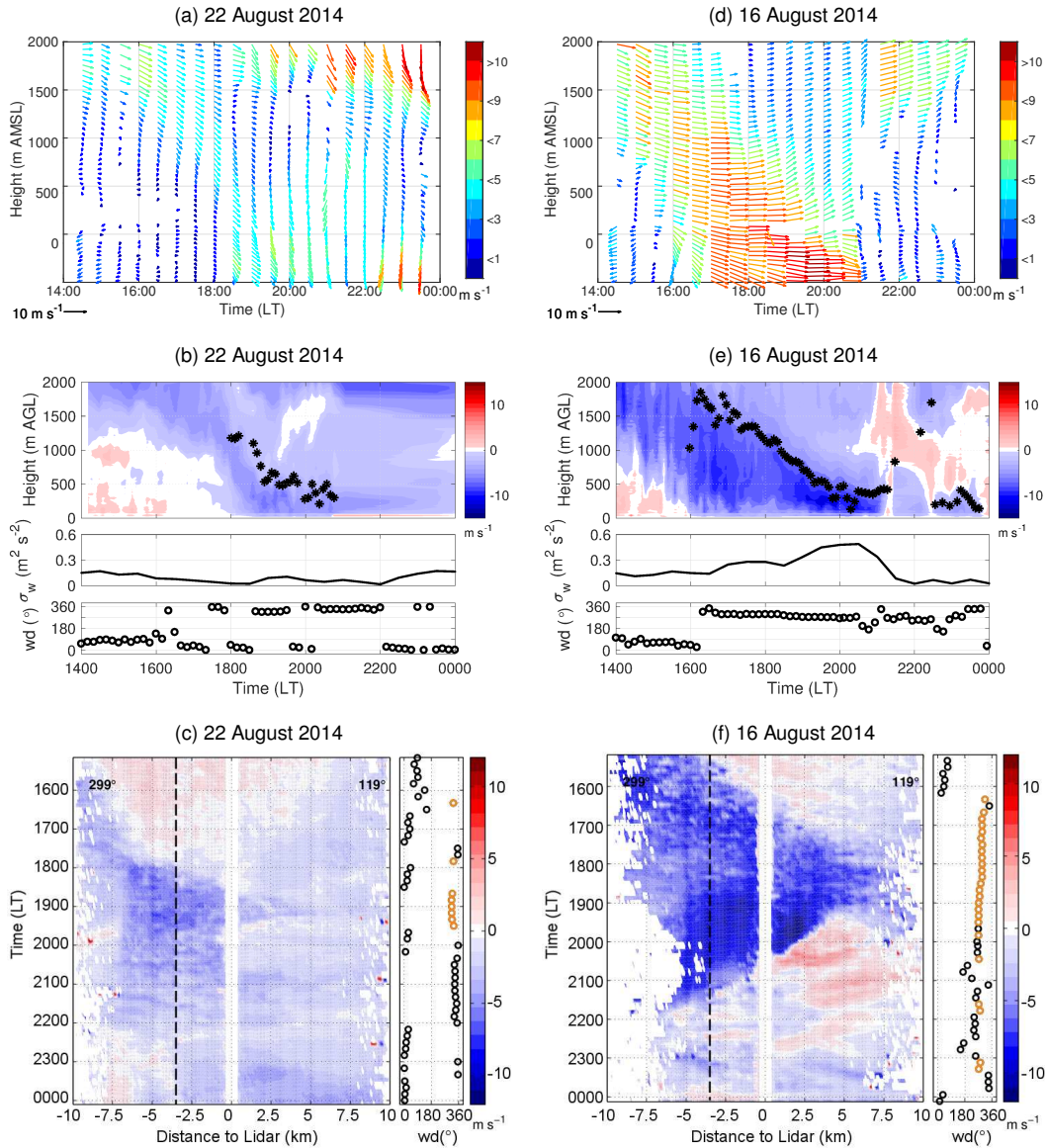
Figure 5. Example for a short and weak foehn event (a,b,c) and for a strong foehn event (d,e,f). Shown are 10 min mean vertical profiles of horizontal wind at the KITcube location (a,d). Length and colours of the arrows represent wind velocity and the direction of the arrows indicate the horizontal wind direction. Time-height cross sections of the averaged vertical profiles of the horizontal radial wind component derived from lidar RHI scans at 299^\circ (b,e). Negative values (blue colours) indicate a wind component from north-west and positive values (red colours) indicate a wind component from south-east. Black stars indicate the detected height of the foehn. Below the cross sections the variance of the vertical wind ( \sigma_w ) at 2 m agl and wind direction ( wd ) measurements in 40 m height are shown. Hovmoeller diagrams of the near-surface radial velocity from lidar RHI scans at an azimuth angle of 299^\circ and 7^\circ elevation west of the lidar and 1.6^\circ east of the lidar (c,f). The black dashed line indicates the end of the western slope and the beginning of the valley floor. Wind direction ( wd ) was measured in 40 m agl. Orange points highlight wind directions between 270^\circ and 330^\circ , the main wind direction of the foehn.
