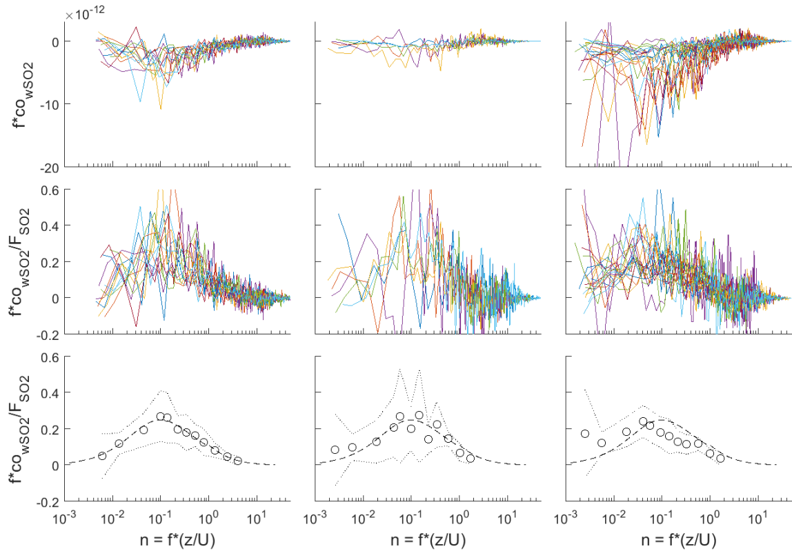
Figure 2. Frequency weighted cospectra of vertical wind and \text{SO}_2 concentration for flux intervals collected at Scripps Pier during three time periods. Left column: DOY 96-102; Center column: DOY 104-109; Right column: DOY 114-117. Top row: individual co-spectra for 13-minute flux intervals; Middle row: Same as top except co-spectra have been normalized to the average flux during the interval. Bottom row: Bin-averages of the flux normalized co-spectra (circles), \pm 1 standard deviation (dotted line), and idealized cospectral shape from Kaimal et al. (1972) (dashed line).
