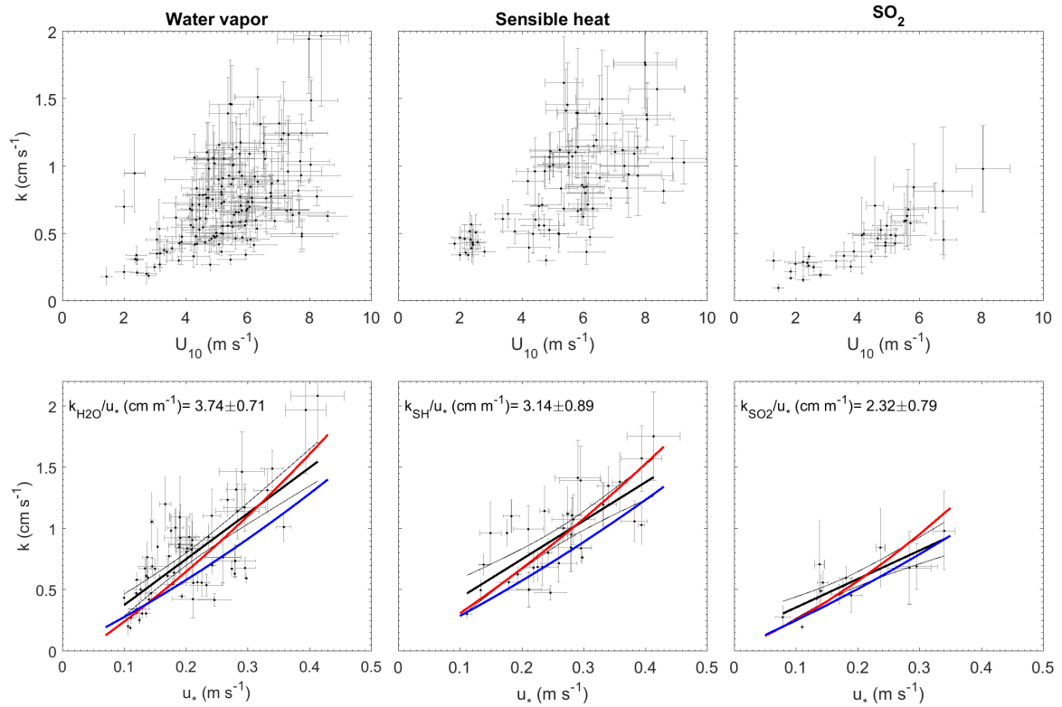
Figure 4. Transfer velocities measured at Scripps Pier as a function of wind and friction velocity. Top row: water vapor, sensible heat, and SO 2 as a function of U_{10} (black dots). Bottom row: water vapor, sensible heat, and SO 2 as a function of u_* with linear least squares regressions and 95% confidence intervals (black dots and black line). Red lines are a second order least squares regression of transfer velocities computed with the COAREG parameterization using measured drag coefficients (Fairall et al., 2000, 2011). Blue lines are transfer velocities computed with COAREG parameterization allowing the model to calculate friction velocities and drag coefficients.
