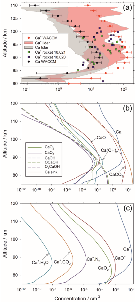
Figure 4: Annual mean concentration profiles of Ca species over Kühlungsborn (54° N): (a) comparison of WACCM-Ca model results (the horizontal error bars indicate 1 standard deviation from the mean) with the lidar measurements of Ca and Ca + (the shaded areas encompass 1 standard deviation from the mean). Note that the model output was sampled to the lidar data over the same period between 1997 and 2000. Also shown are mass spectrometric measurements of Ca + made by two rockets which were launched from Red Lake (50.9° N, Canada), on 24/Feb/1979 11:52 LT and 26/Feb/1979 11:55 LT (payloads 18.020 and 18.021 (Kopp and Herrmann, 1984; Kopp, 1997)); (b) modelled vertical profiles of neutral Ca species in WACCM-Ca, where “CaCO 3 ” = CaCO 3 + O 2 CaCO 3 + OCaCO 3 ; (c) modelled vertical profiles of ionic Ca species in WACCM-Ca.
