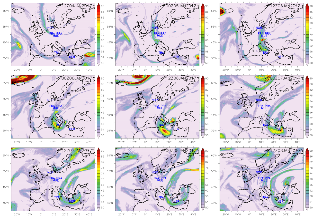
Figure 4. RegEns ozone mixing ratio (in ppb; color shaded) at 5000 m during the period 12Z 04 Jan 2017 to 12Z 08 Jan 2017 (12 hours interval). Also shown are the locations of the observational sites (blue text) used in the study.
