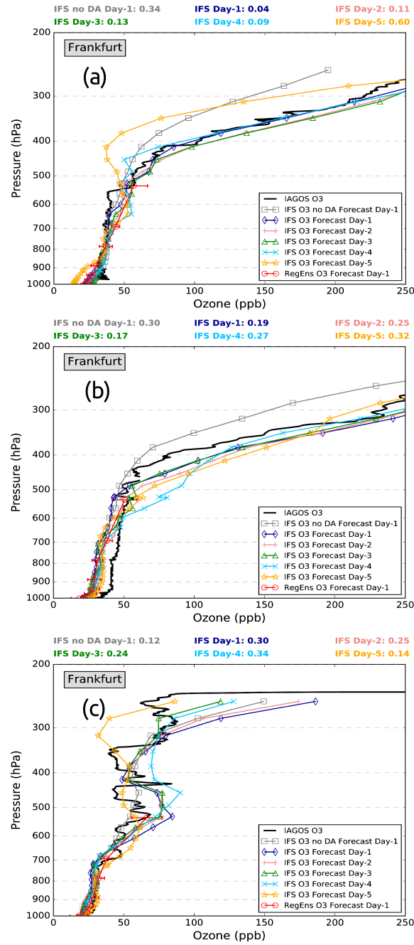
Figure 11. Profiles of ozone mixing ratio (ppb) over the broader area of Frankfurt (8.5°E, 50°E) for IAGOS (black line), IFS forecast Day-1 (dark blue line), IFS forecast Day-2 (coral line), IFS forecast Day-3 (green line), IFS forecast Day-4 (light blue line), IFS forecast Day-5 (orange line), IFS no DA (without data assimilation) forecast Day-1 (grey line) and RegEns (red line) during (a) 13Z 04 Jan 2017, (b) 06Z 05 Jan 2017, (c) 13Z 05 Jan 2017. The red bars denote the standard deviation among the regional ensemble members. The numbers above the diagrams show the FGE values of IFS ozone (with the corresponding color) at 300-500 hPa (a and b) and 400-600 hPa (c).
