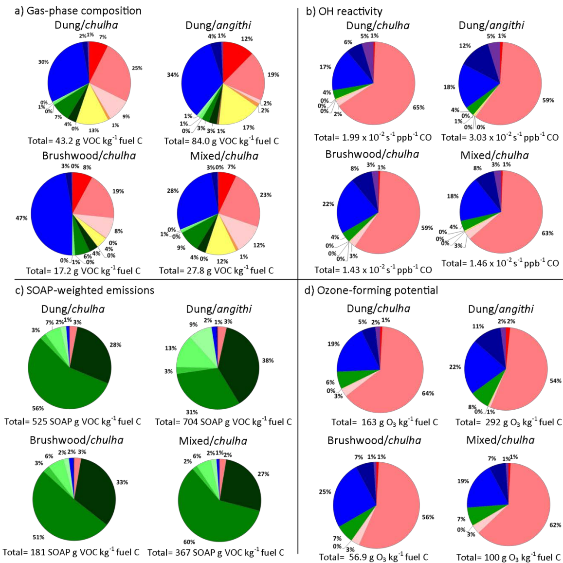
Figure 2. Pie charts showing the contribution of each species class to gas-phase composition (a), OH reactivity (b), SOAP-weighted emissions (c), and ozone-forming potential (d). For (b) and (d), total aromatics are shown rather than the breakdown of aromatics shown in (a) and (c). Sums of all components are shown below the pie chart.
