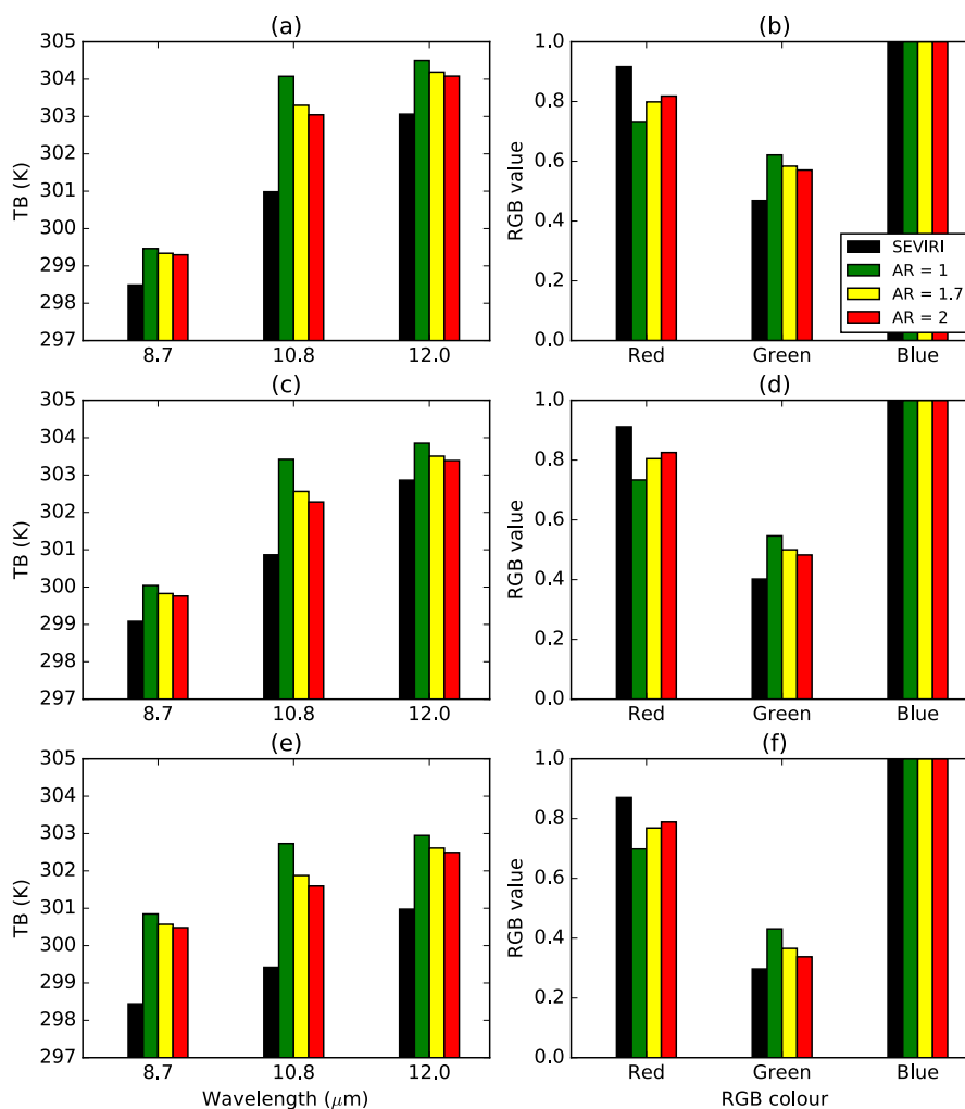
Figure 10. Mean brightness temperatures and RGB colours across the domain for the three ranges of surface emissivity values, for the SEVIRI measurements/retrievals and tested for the VO73 dust simulations with the three (horizontally aligned) aspect ratios of 1, 1.7, and 2, for the Junes and Julys of 2011-2013. Only points with AODs between 2 and 3 are included. Using emissivity at 8.7 \mu\text{m} , the panels are: (a, b) emissivity from 0.7-0.8; (c, d) 0.8-0.9; (e, f) 0.9-1.0.
