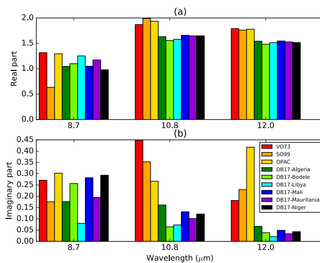
Figure 4. Plots of the real (a) and imaginary (b) parts of the dust refractive index, for nine of the dust databases considered in this study, which have been convolved across the MSG-3 SEVIRI filter functions.
