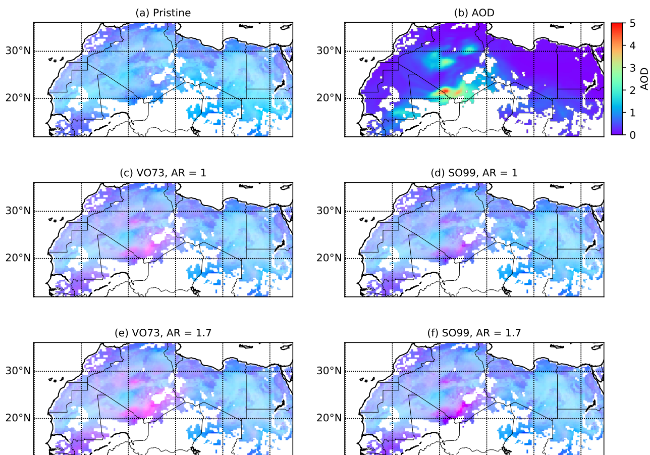
Figure 8. Simulated SEVIRI Desert Dust RGB images, 1200 UTC on 25th June 2013. (a) Pristine-sky; (b) COSMO-MUSCAT AOD at 550 nm; (c, e) VO73 dust for AR values of 1 and 1.7 (horizontally aligned); (d, f) the SO99 dust mixture for the two AR values.
