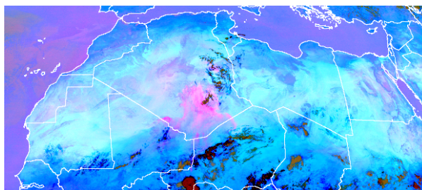
Figure 1. Desert Dust RGB image from MSG-3 SEVIRI, 1200 UTC on 25th June 2013.
