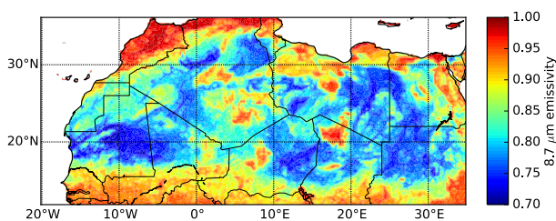
Figure 3. Map of climatological surface emissivity for the MSG-3 SEVIRI channel at 8.7 \mu\text{m} used by the RTTOV program for June, derived by Borbas and Ruston (2010) using MODIS satellite data.
