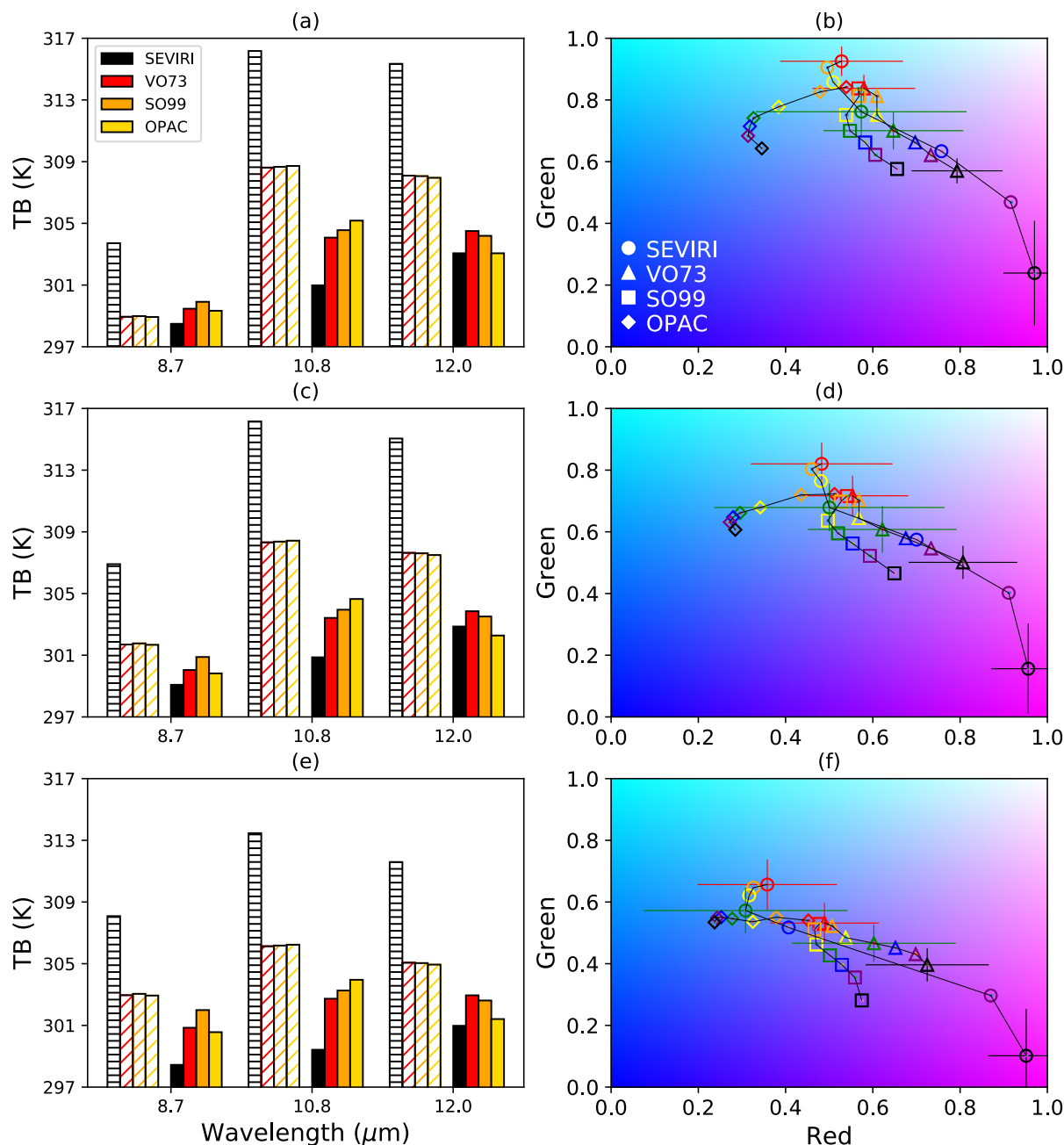
Figure 9. Mean brightness temperatures and colours across the domain for three ranges of surface emissivity values, for the SEVIRI measurements/retrievals and three of the dust simulations, for the Junes and Julys of 2011-2013. Using emissivity at 8.7 \mu\text{m} , the panels are: (a, b) emissivity from 0.7-0.8; (c, d) 0.8-0.9; (e, f) 0.9-1.0. The simulated dust is spherical. Per panel of brightness temperatures (left column), within each individual wavelength set there are two groups of bars: the striped bars on the left are points with AODs between 0 and 0.2 (i.e. the most pristine-sky case); the bold bars on the right are points with AODs between 2 and 3. The mean colours (right column) are plotted within specified AOD ranges denoted by the coloured symbols: red is 0-0.2; orange is 0.2-0.5; yellow is 0.5-1; green is 1-1.5; blue is 1.5-2; purple is 2-3; black is > 3 . The blue beam is held fixed at 1. Error bars denoting the standard deviations of the mean values are only included, for clarity, for three of the SEVIRI and the VO73 points.
