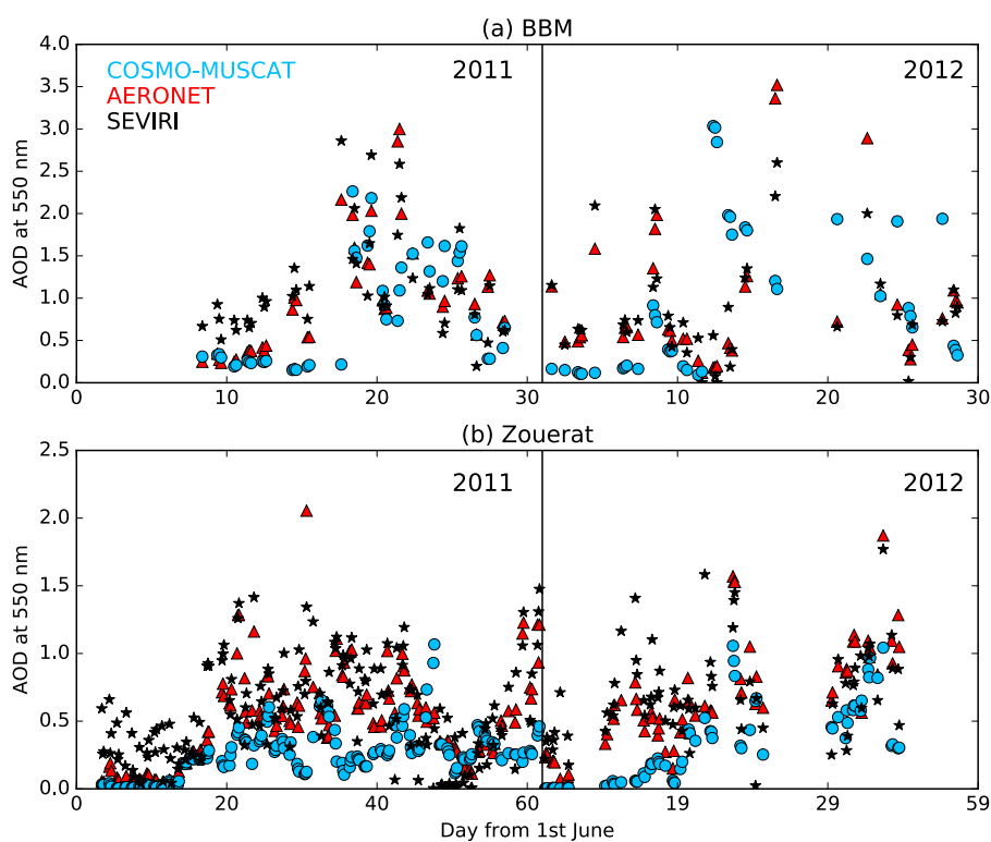
Figure 7. Time-series of measurements, retrievals, and simulations of AOD at 550 nm over the Fennec BBM and Zouerat AERONET sites, during 2011 and 2012 when AERONET data are available, linked into one time-series: (a) BBM, the two June months; (b) Zouerat, the four months of Junes and Julys.
