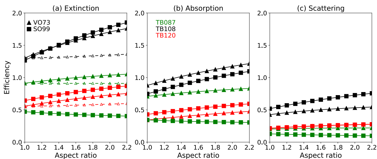
Figure 6. Plots of the derived (a) extinction, (b) absorption and (c) scattering efficiencies for the VO73 and SO99 dust types, as a function of particle aspect ratio, for COSMO-MUSCAT dust size bin 3 ( r_{\text{eff}} = 1.51 \mu\text{m} ) for the three MSG-3 SEVIRI channels at 8.7, 10.8, and 12.0 \mu\text{m} . The solid lines are for horizontally aligned particles, the dashed lines for randomly oriented particles. For clarity, the randomly oriented case is only included in the extinctions for VO73 dust.
