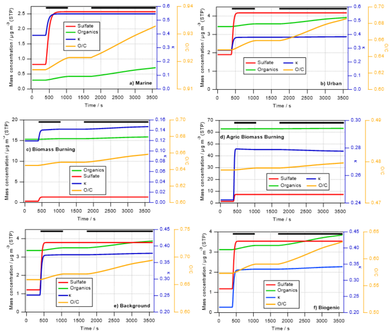
Figure 1 I (second right axis) show the predicted bulk O/C ratios as calculated based on predicted aqSOA formation ( Section 2 ). In all cases, the O/C ratio increases close to the beginning of the simulations, with the lines following the same trends as predicted for the aqSOA mass increase ( Section 3.1.1 ). The increase in O/C ratio continues still in the second passage of the parcel through the cloud. This increase is caused both by oxidation of dissolved VOCs and by the further oxidation of aqSOA products that have been formed in the cloud water (e.g. oxidation of glyoxylic to oxalic acid). Similar to the findings for the mass increase and \kappa , the largest increase in O/C ratio can be seen for the urban, marine and biogenic cases with \Delta(\text{O/C}) \leq 0.4 . For the biomass burning cases, the changes are rather subtle with an increase of \Delta(\text{O/C}) \leq 0.1 . It should be noted that this change might even represent an overestimate as we neglect numerous physical and chemical processes that could lead to a weaker increase in \Delta(\text{O/C}) or even to its decrease. Such processes include non-oxidative reactions that lead to aqSOA which will produce less-oxygenated aerosol. It was discussed that IEPOX might contribute significantly to aqSOA in wet aerosol (Budisulistiorini et al., 2017) or non-photochemical processes in fog (Sullivan et al., 2016). Wet deposition or further oxidation of oxygenated and highly
