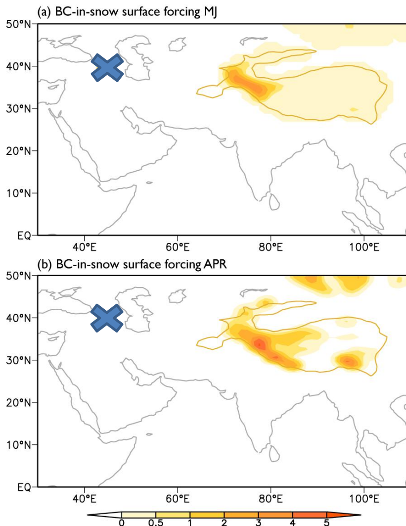
Figure R5: Surface forcing of black-carbon-in-snow during May to June ( \text{W m}^{-2} , a) and April ( \text{W m}^{-2} , b). Yellow line shows the profile of Tibetan Plateau above 2500 m.
