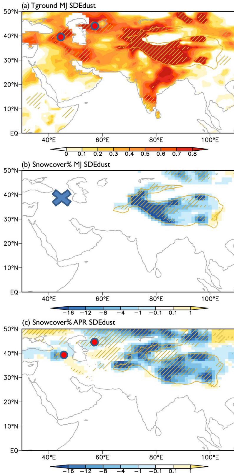
Figure R2: Changes in surface ground temperature in May and June (a) and snow cover fraction during May to June (%), (b) and April (%), (c) induced by snow-darkening effect. Oblique lines indicate differences significant at 95% confidence level. Yellow line shows the profile of Tibetan Plateau above 2500 m.
