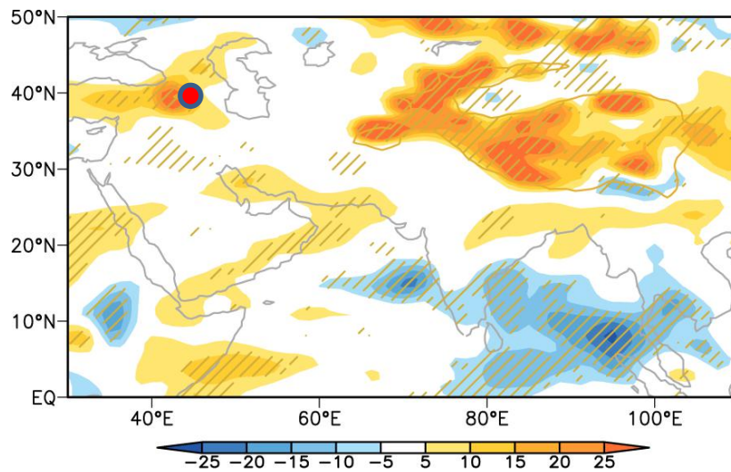
Figure R3: Changes in the surface shortwave radiation fluxes during April due to SDE of dust. Oblique lines indicate differences significant at 95% confidence level. Yellow line shows the profile of Tibetan Plateau above 2500 m.
