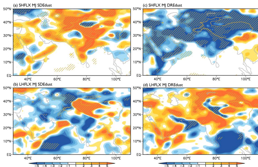
Figure R1: Changes in surface sensible and latent heat fluxes in May and June induced by snow-darkening effect (a, b) and direct radiative effect of dust (c, d), respectively. Oblique lines indicate differences significant at 95% confidence level. Yellow line shows the profile of Tibetan Plateau above 2500 m.
