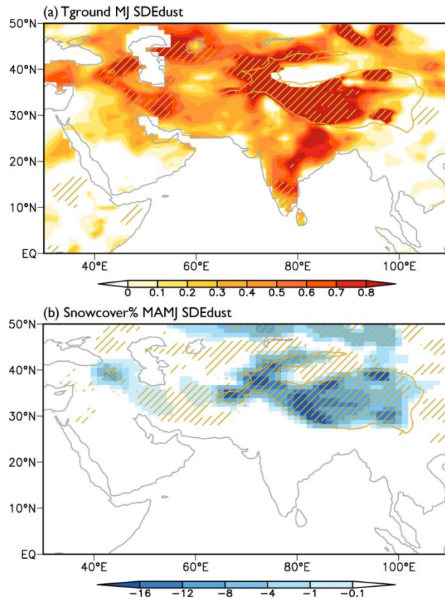
Figure R2: Changes in surface ground temperature in May and June (a) and snow cover fraction during March to June (b) induced by snow-darkening effect. Oblique lines indicate differences significant at 95% confidence level. Yellow line shows the profile of Tibetan Plateau above 2500 m.
