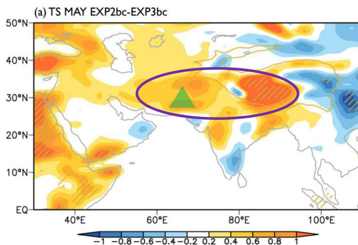
Figure R4: Changes in surface temperature induced by direct radiative effect of black carbon.
