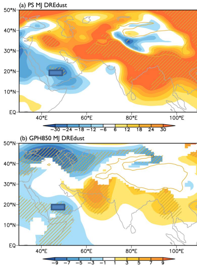
Figure R7: Changes in surface pressure and 850hPa geopotential height induced by direct radiative effect of dust. Oblique lines indicate differences significant at 95% confidence level.
