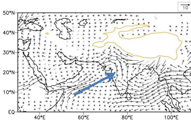
Figure R8: Changes in 850hPa wind vectors and moisture flux induced by direct radiative effect of dust. Black vectors indicate differences significant at 90% and 95% confidence levels for top and bottom subfigures, respectively.
