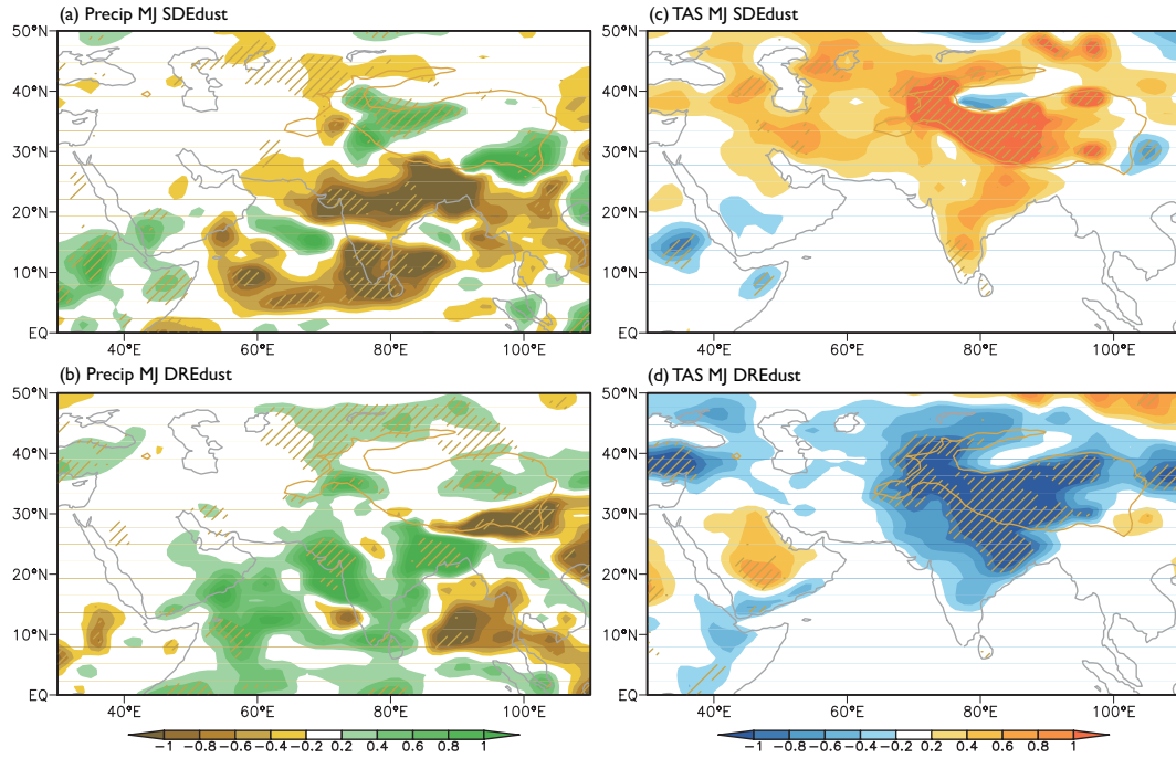
Figure 5. Spatial distribution of changes in precipitation rates (a, b, \text{mm day}^{-1} ) and surface air temperature (c, d, ^{\circ}\text{C} ) in May and June induced by snow-darkening effect (top) and direct radiative effect of dust (bottom), respectively. Oblique lines indicate differences significant at 95% confidence level. Yellow line shows the profile of Tibetan Plateau above 2500 m.
