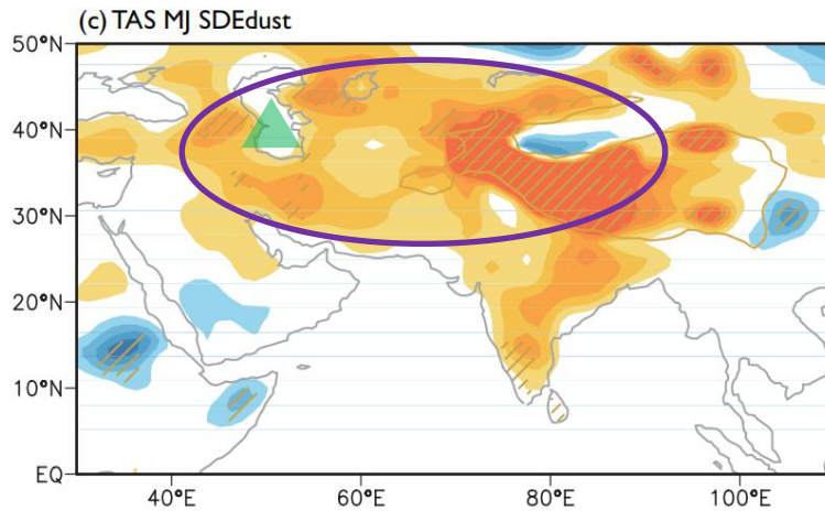
Figure R5: Changes in surface temperature induced by snow darkening effect of dust.
