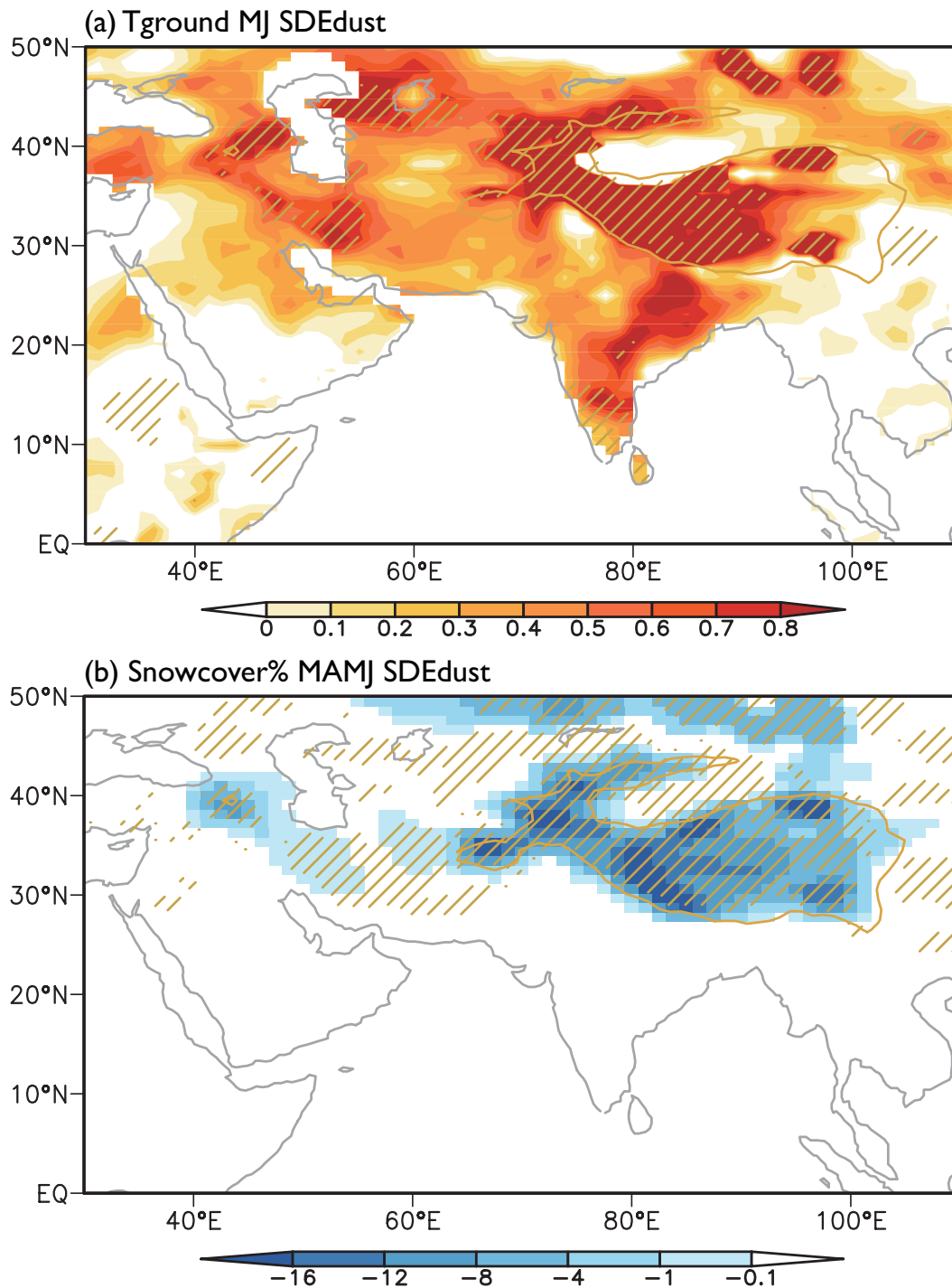
Figure 12. Changes in surface ground temperature in May and June ( ^{\circ}\text{C} , a) and snow cover fraction during March to June ( \% , b) induced by snow-darkening effect. Oblique lines indicate differences significant at 95% confidence level. Yellow line shows the profile of Tibetan Plateau above 2500 m.
