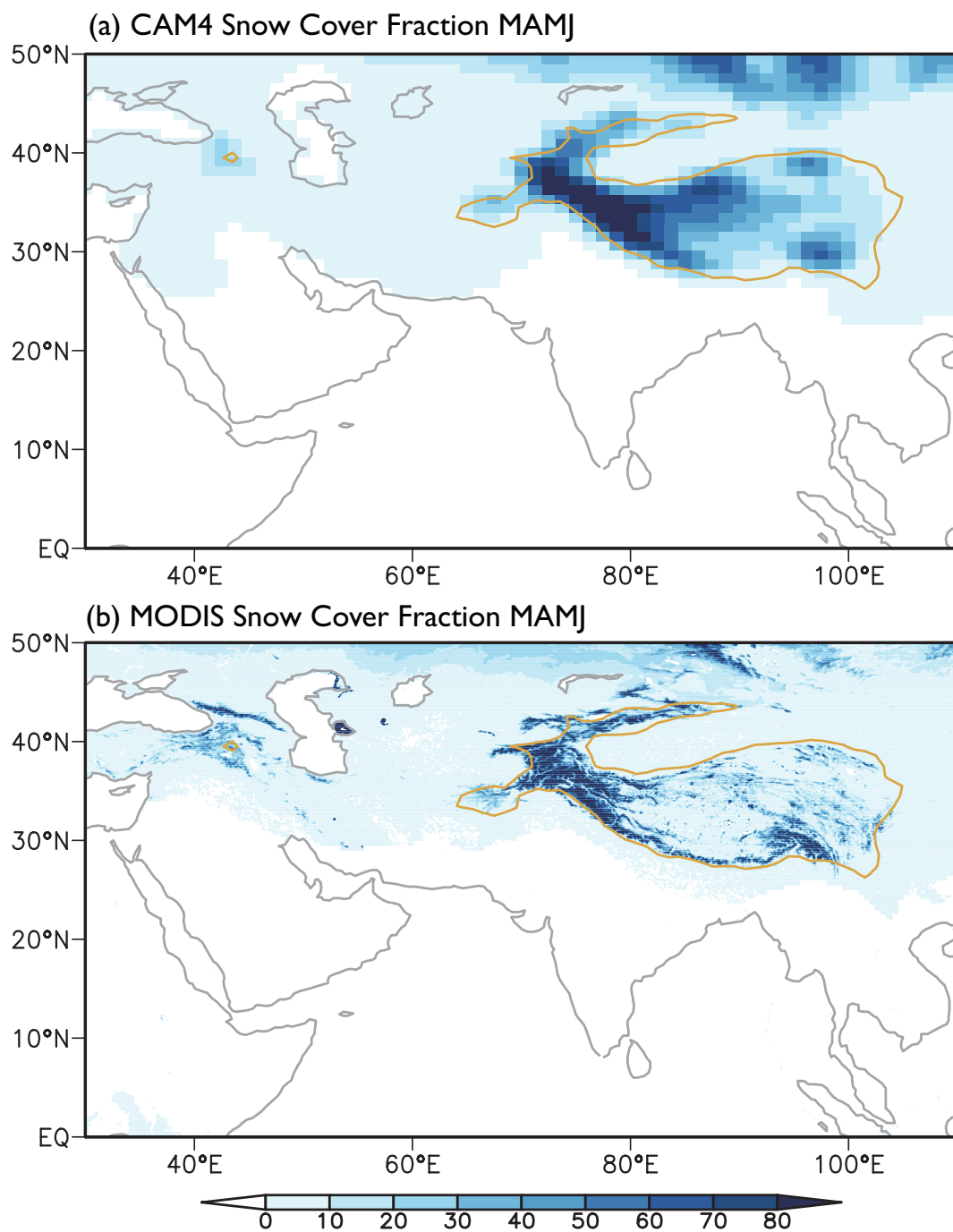
Figure 2. Snow cover fraction (%) over Asia for March to June in CAM4 (a) and in Moderate Resolution Imaging Spectroradiometer (MODIS)-retrieved observation. Yellow line shows the profile of Tibetan Plateau above 2500 m.
