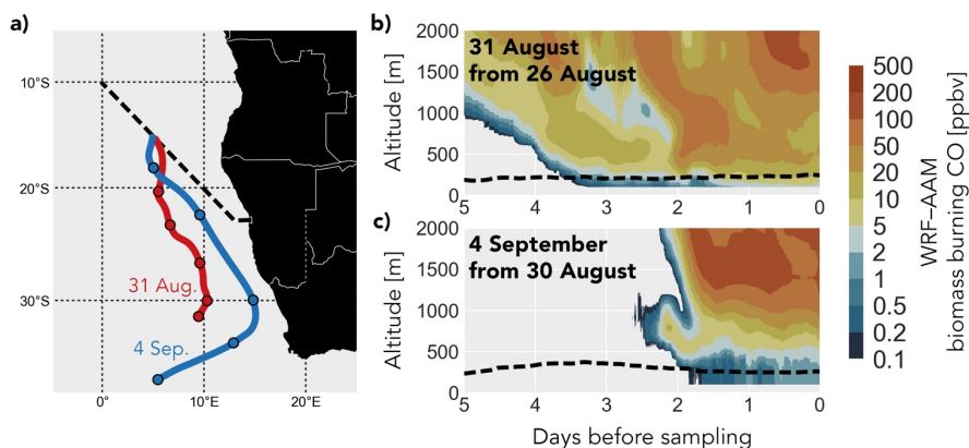
Figure 5. (a) Map of HYSPLIT MBL back trajectories for 31 August (red) and 4 September (blue). Circles are plotted every 24 hours after initialization. The ORACLES-2016 routine flight path is plotted as a dashed black line for reference. Curtains of WRF-AAM biomass burning tagged CO along the path of the trajectories are plotted in (b) for 31 August and c) for 4 September, with the trajectory altitude indicated by the dashed black line.
