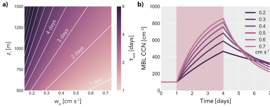
5 Figure 7. (a) Characteristic (e-folding) entrainment mixing timescale for a range of plausible z_i and w_e values. Contours at one day intervals for reference. (b) Evolution of \text{CCN}_{\text{MBL}} over time in response to the introduction of a smoke plume with \text{CCN}_{\text{FT}} = 1000 \text{ cm}^{-3} at day 1 and its removal at day 4 (highlighted). Curves show results for a range of entrainment timescales with z_i = 1 \text{ km} and w_e varying between 0.2 and 0.7 \text{cm s}^{-1} .
