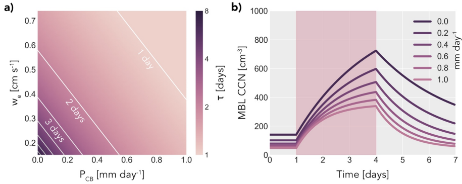
Figure 8. (a) Characteristic (e-folding) entrainment mixing timescale for a range of plausible w_e and P_{CB} values. Contours at one-day intervals for reference. (b) Evolution of \text{CCN}_{\text{MBL}} over time in response to the introduction of a smoke plume with \text{CCN}_{\text{FT}} = 1000 \text{ cm}^{-3} at day 1 and its removal at day 4 (highlighted). Curves show results for a range of equilibration timescales with z_i = 1 \text{ km} , w_e = 0.4 \text{ cm s}^{-1} , h = 300 \text{ m} , and P_{CB} varying between 0 and 1 \text{ mm day}^{-1} .
