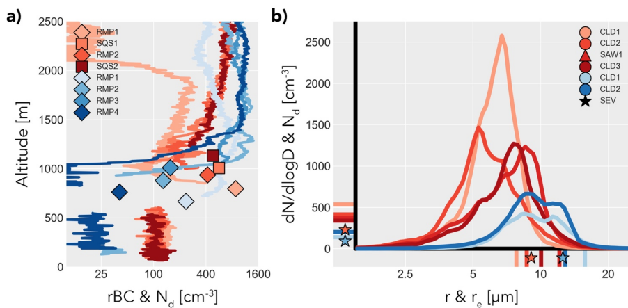
Figure 4. Cloud microphysical properties and rBC for the 31 August (reds) and 4 September (blues) flights. (a) Vertical profiles of rBC number concentration (lines) and average N_d (markers) for each RMP and SOS profile. The vertical positions of the markers indicate cloud top height for each profile and the horizontal positions indicate the average N_d value. Note that rBC and N_d share the same x-axis because they have the same units and similar magnitudes. (b) Average cloud droplet spectra (curves), N_d (ticks on y-axis), and r_e (ticks on x-axis) for each CLD and SAW leg. Stars indicate the values of N_d and r_e from SEVIRI (SEV) averaged over the 31 August (light red) and 4 September (light blue) flight paths.
