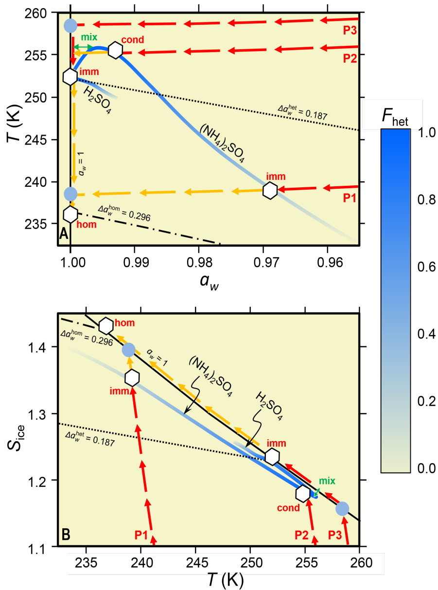
110 Figure 9. Phase diagrams, a_w - T (panel A) and T - S_{ice} (panel B), showing the development of aerosols containing microcline in dry (P1), moist (P2) and wet (P3) air parcels undergoing adiabatic cooling (red arrows) until ice nucleates (white hexagons). Blue curves: heterogeneous freezing onset temperatures, T_{het} , of 2 wt% microcline suspended in aqueous (NH_4)_2SO_4 or H_2SO_4 solutions. Color coding: heterogeneously frozen fraction, F_{het} , ranging from high (blue) to vanishing (yellow). In aqueous (NH_4)_2SO_4 , ice can nucleate heterogeneously on microcline. In aqueous H_2SO_4 , microcline is largely deactivated and ice nucleates homogeneously only after further cooling (yellow arrows) and forming a supercooled liquid water cloud (filled blue circles). Solid black line: water saturation ( a_w = 1 , RH = 100%). Dash-dotted black line: homogeneous ice nucleation, horizontally shifted from the ice melting curve by a constant offset \Delta a_w^{hom} = 0.296 . Dotted black line: shifted by \Delta a_w^{het} = 0.187 derived from microcline suspended in pure water. Atmospheric freezing modes: “imm” = immersion; “cond” = condensation; “hom” = homogeneous. Entrainment/detrainment at cloud edges may cause nucleation at up to 4 K higher temperature than “imm” (green double arrow, “mix”). 115 120
