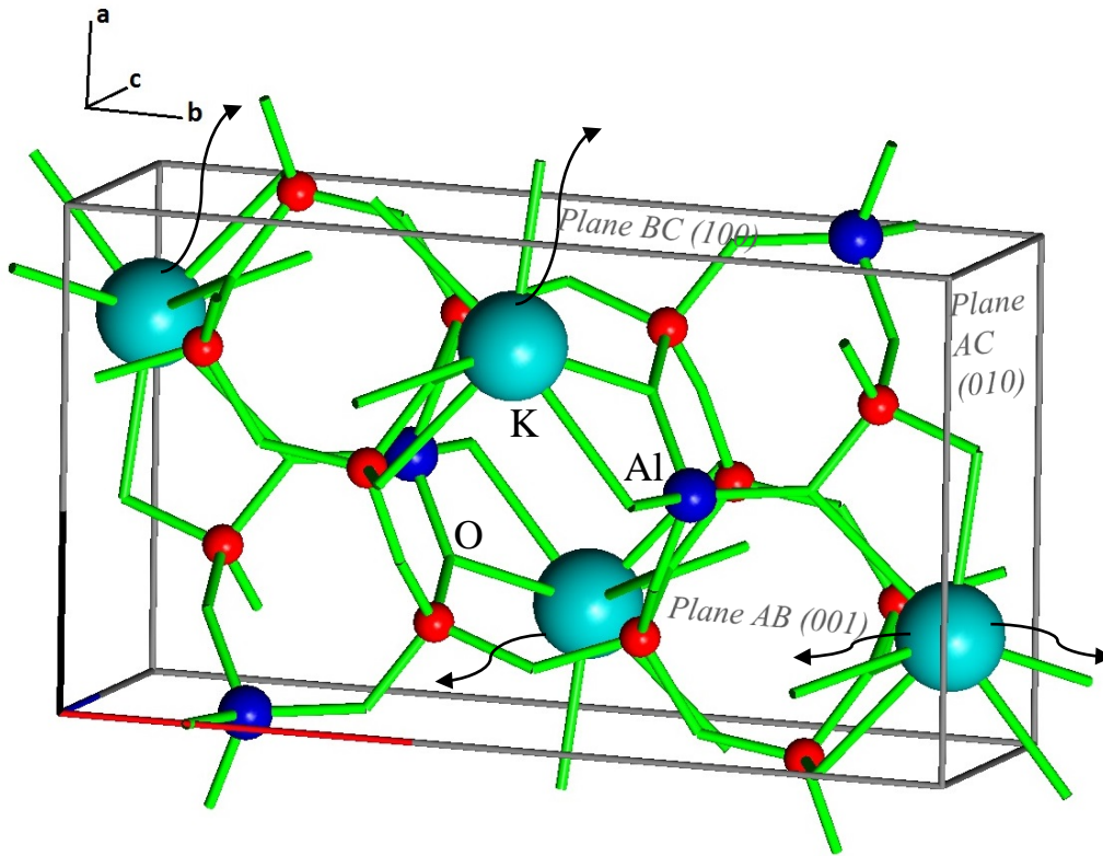
Figure A1. Simplified parallelepiped version of a primitive unit cell of microcline (chemical composition K_4Al_4Si_{12}O_{32} ). Red spheres: Si atoms; blue spheres: Al atoms; cyan spheres: K atoms; green lines: -O- links between 2 neighboring Si/Al atoms. Black curved arrows show potential removal paths of K^+ from different planes of the unit cell (namely, AB, BC and AC). We assume that all K^+ from half of the unit cell are available for exchange, hence only the K^+ nearest to a plane can potentially move out from that particular plane.
