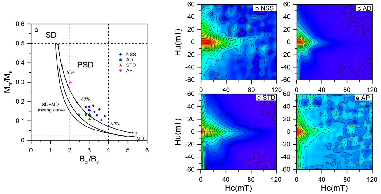
Fig. 4 (a) Day-plot of the ratios M_{rs}/M_s and B_{cr}/B_c for representative samples from NSS, AD, STD, and AP, grain size boundaries and the SD+MD matrix line are according to Dunlop (2002). Percentages in the Day plot represent the concentrations of MD in the SD+MD mixture; (b-e) FORC diagrams for representative samples of NSS, AD, STD, and AP.
