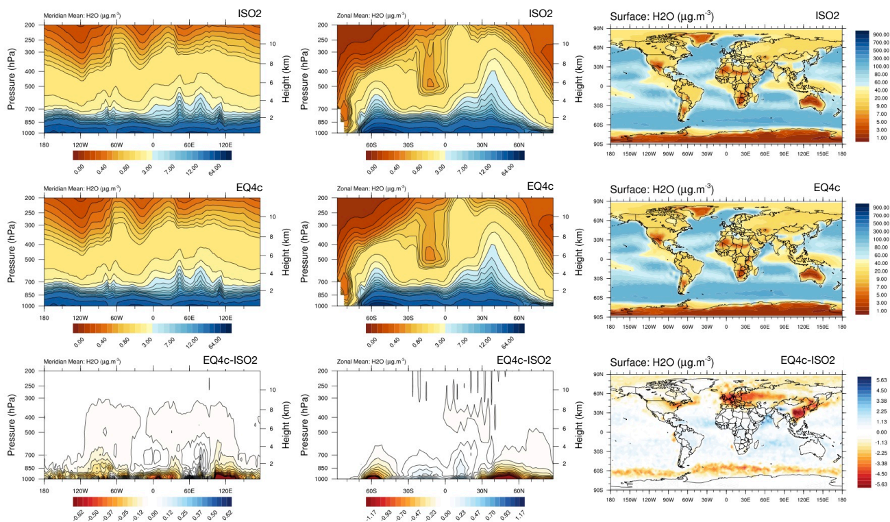
Figure 8. Fig. 7 continued for EMAC aerosol associated water (2000-2013 mean).
