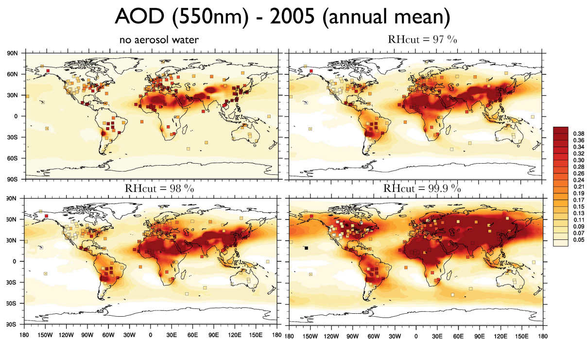
Figure 15. Sensitivity of EMAC AOD to different RH cut-offs (see text Sec. 4.3).
