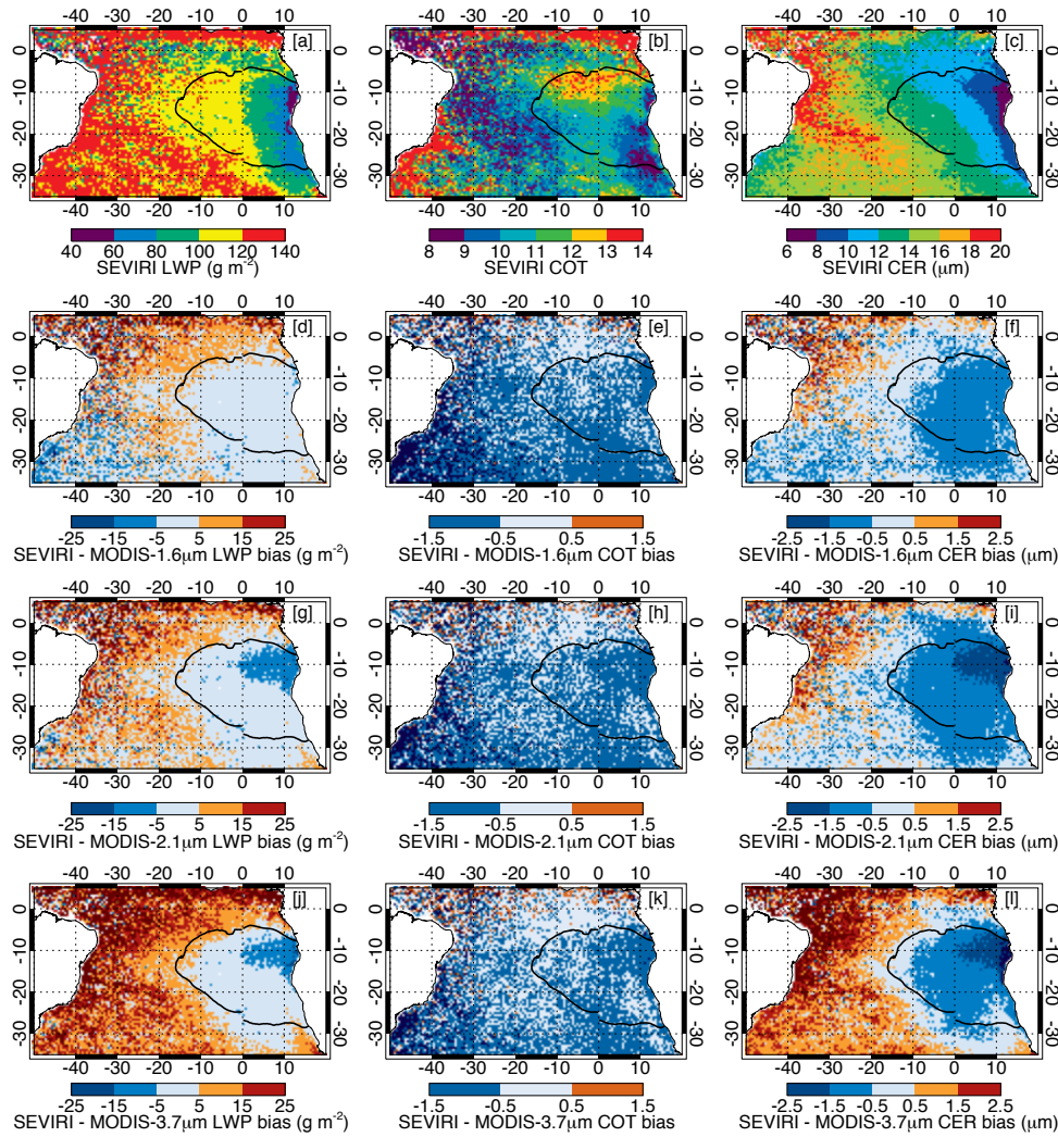
Figure 6. Two-year mean map of (a) SEVIRI LWP, (b) SEVIRI COT, (c) SEVIRI CER, (d, g, j) SEVIRI minus MODIS liquid water path biases, (e, h, k) SEVIRI minus MODIS cloud optical thickness biases, (f, i, l) SEVIRI minus MODIS droplet effective radius biases for the overcast case (LCF \geq 95% and COT > 3) in ice- and smoke-free conditions.
