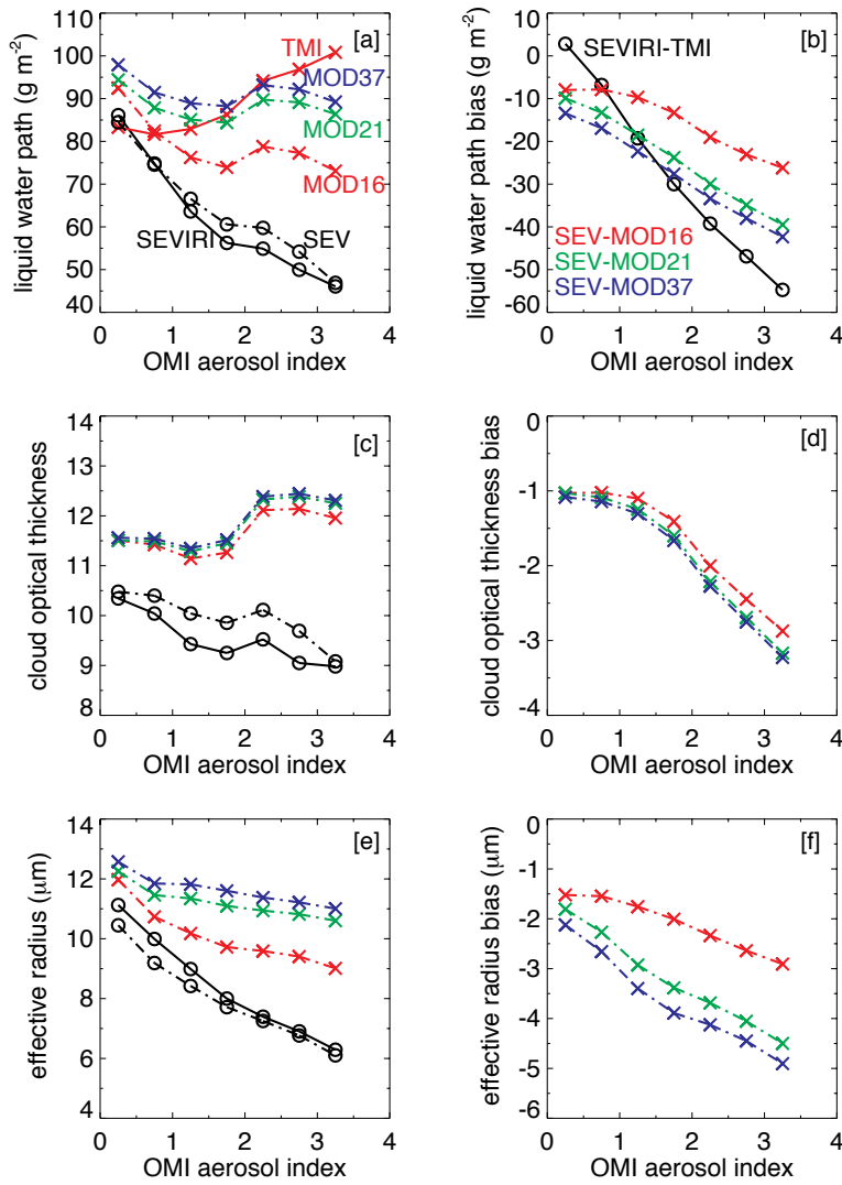
1195 Figure 2. OMI aerosol index versus (a) SEVIRI, TMI and MODIS LWPs, (b) SEVIRI LWP biases compared to TMI and 1200 MODIS, (c) SEVIRI and MODIS COTs, (d) SEVIRI – MODIS COT biases, (e) SEVIRI and MODIS CER, and (f) SEVIRI – MODIS CER biases, over the overcast Sc region for JAS 2011 and JAS 2012 for rain- and ice-free conditions. Solid lines correspond to SEVIRI vs. TMI comparison, whereas dash-dotted lines correspond to SEVIRI vs. MODIS comparison. The label “SEV” refers SEVIRI values at MODIS collocations.
