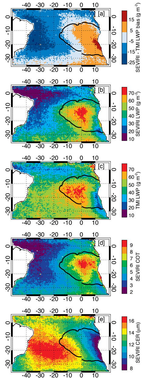
Figure S2. Two-year mean map of (a) SEVIRI minus TMI LWP difference, (b) SEVIRI LWP, (c) TMI LWP, (d) SEVIRI COT, (e) SEVIRI 1.6- \mu\text{m} CER, for the all-sky case. The solid black contour denotes the identified Sc region. Rain-, ice-, and aerosol-free conditions were applied.
