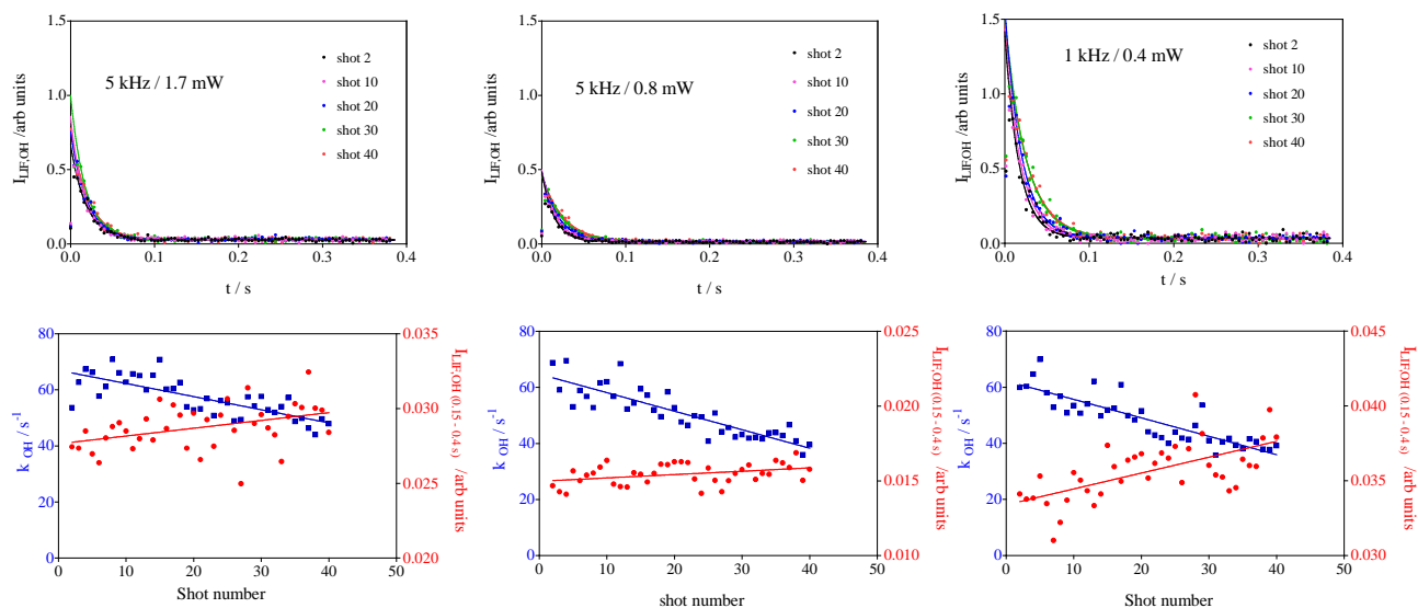
Figure 5: Photolysis of O 3 in the presence of isoprene using different excitation laser energies and repetition rates. Upper graphs: OH decays (for clarity, only every 10 th decay is shown), lower graph OH decay rate as a function of photolysis pulses (blue dots, left y-axis) and fluorescence intensity averaged over 0.15 to 0.4 s (red dots, right y-axis).
