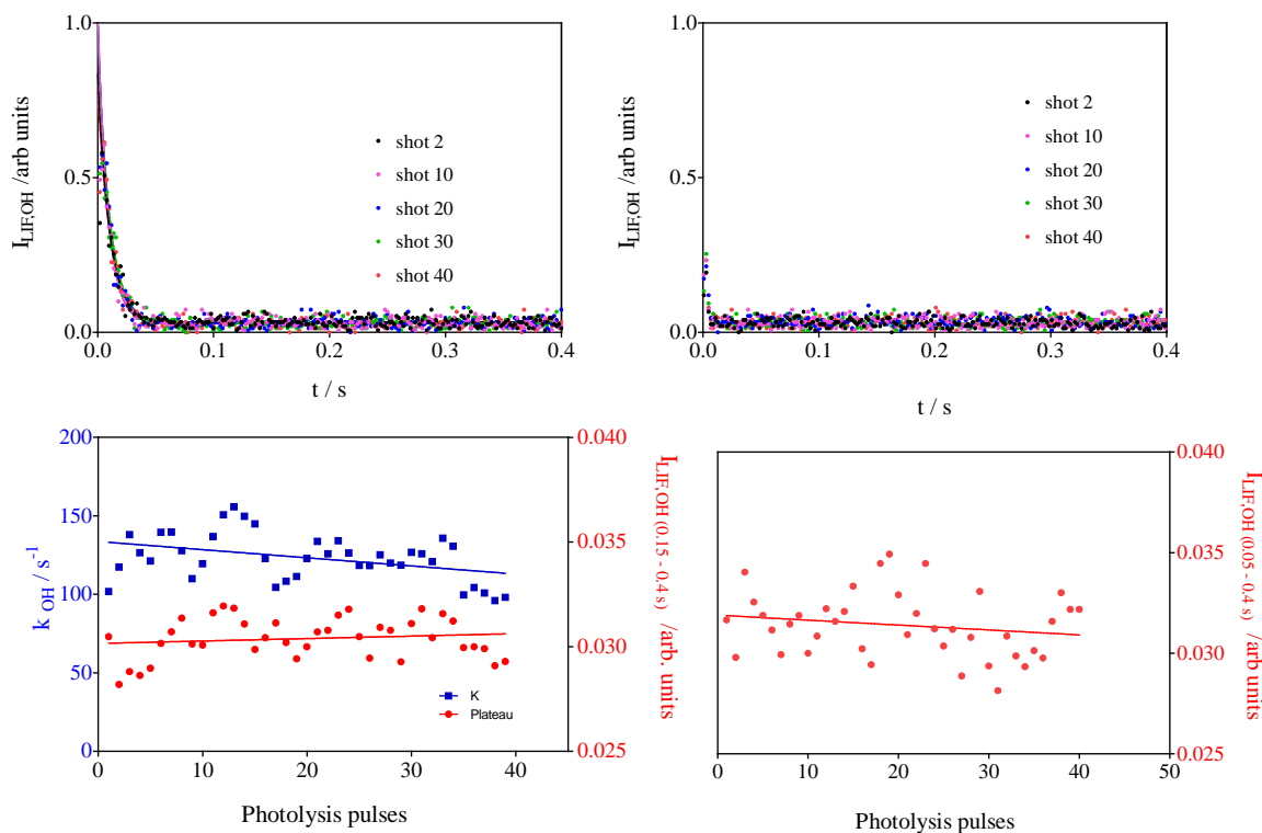
Figure 6: Experiments with high isoprene concentrations: [\text{C}_5\text{H}_8] = 1.23 \times 10^{12} and 1.23 \times 10^{13} molecule. \text{cm}^{-3} for left and right graph, respectively. Upper graph LIF signals as a function of the number of photolysis pulses (for clarity, only every 10 th pulse is shown), lower graph shows the rate constant in blue (left graph only, decay was too fast to be measurable under the conditions of the right graph) and the LIF intensity at long times (plateau from fitting for left graph, average of all data points between 0.01 – 0.4 s for right graph).
