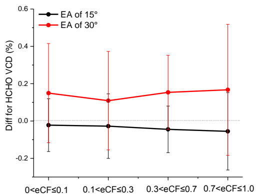
Figure 6. Relative differences in the tropospheric HCHO VCDs derived by geometric approximation and from profile inversion as a function of the effective cloud fractions (eCF), as 0 < eCF \leq 0.1 , 0.1 < eCF \leq 0.3 , 0.3 < eCF \leq 0.7 , and 0.7 < eCF \leq 1.0 for elevation angles of 15° and 30°. Error bars denote the standard deviations. Diff were calculated by Eq. (9) in the text.
